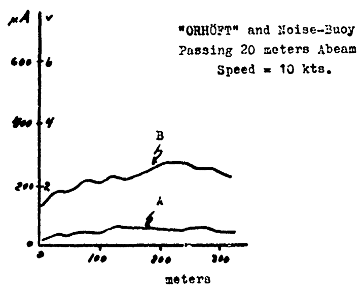
Fig. 6 AA 106 Receivers - Reaction to Ship Passing Abeam
