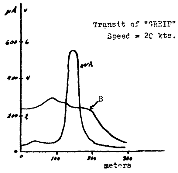
Fig. 5 AA 106 Receivers - Reaction to Ship Transit
