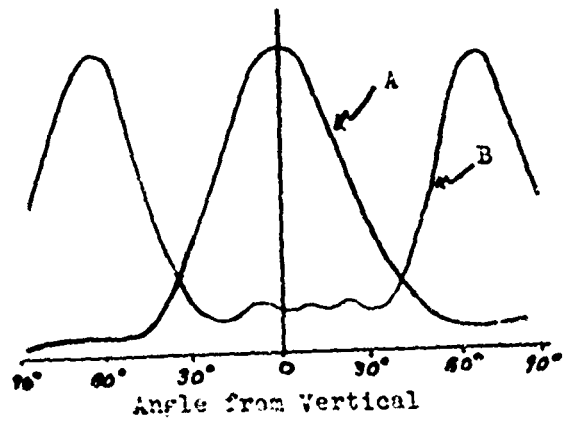
Fig. 2 Directional Characteristics - AA 1,6 Receivers
