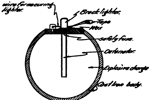
SECTION. Diameter of Grenade 3" BALL HAND GRENADE.
