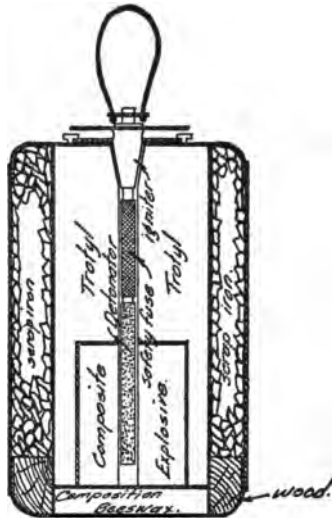
SECTION. Dimension of Cylinder 4 1/2" HAND GRENADE NO. 7.
