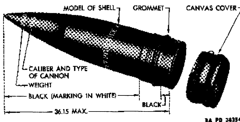
Figure 104—SHELL, C.I., 260-Lb, Mk. XVIII, 8-In., Guns, M1888-88MI-88MII and Mk. VI, Mod. 3A2 (Navy)
