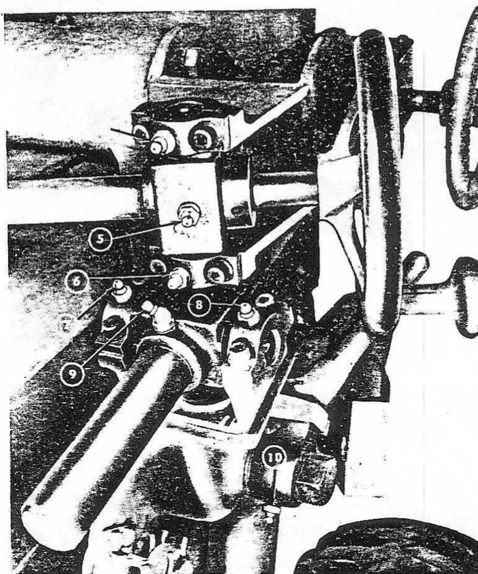
Figure 31—Lubrication Points Nos. 4 to 10 Inclusive
