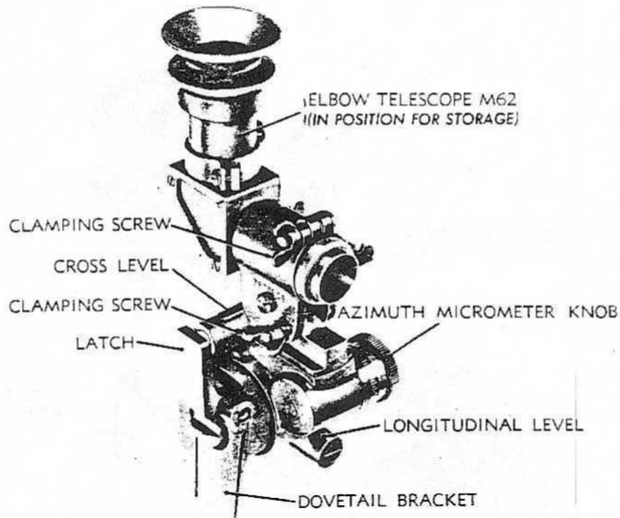
Figure 49—Telescope Mount T72E1 With Elbow Telescope M62— Telescope in Position for Storage—Right Front View
