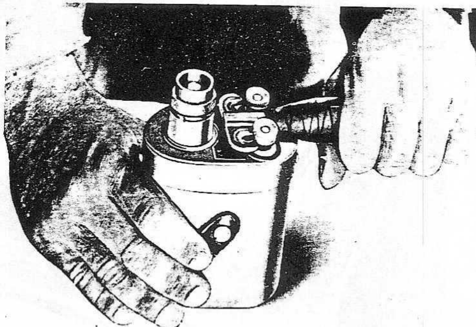
Figure 24—Connecting Firing Cable to Blasting Machine (Launcher T66)
