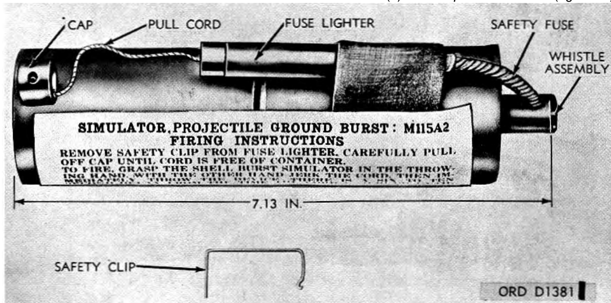
Figure 9-17. Ground burst simulator.
