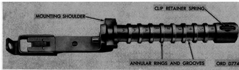
Figure 6-5. Grenade launcher.
