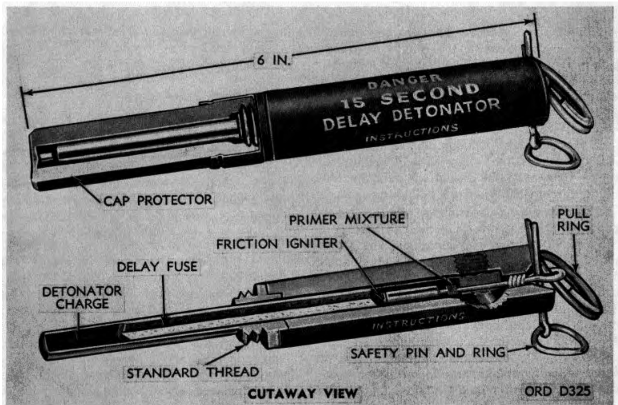
Figure 8-8. 15-Second delay friction detonator.
