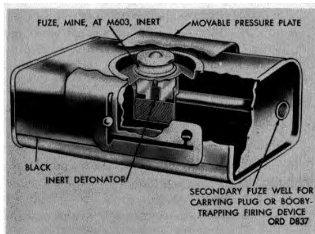
Figure 7-12. Inert light AT mine and inert fuze.
