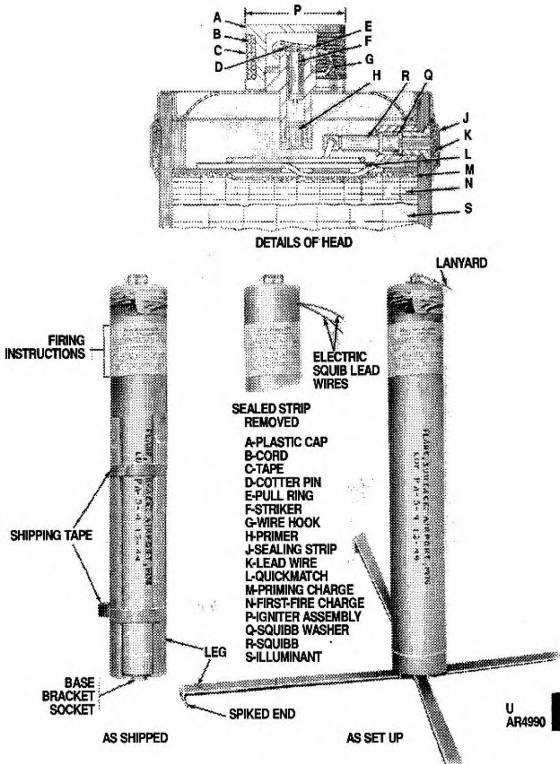
Figure 9-5. Airport flare.
