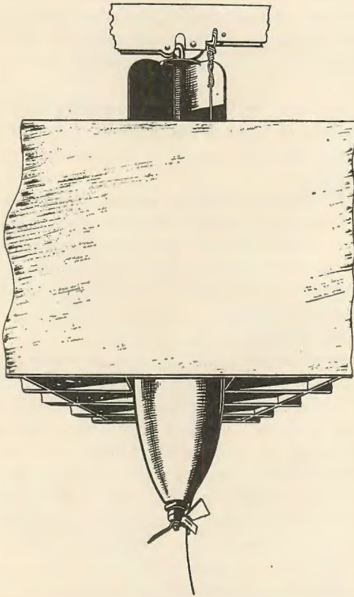
FIGURE 13.—Vertical suspension of 30-pound M1 (WP) bomb in bomb bay of airplane.
