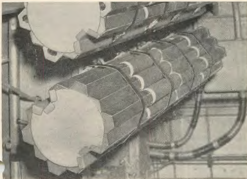
FIGURE 10.—Loaded cluster adapter M3 suspended in bomb bay of airplane.
