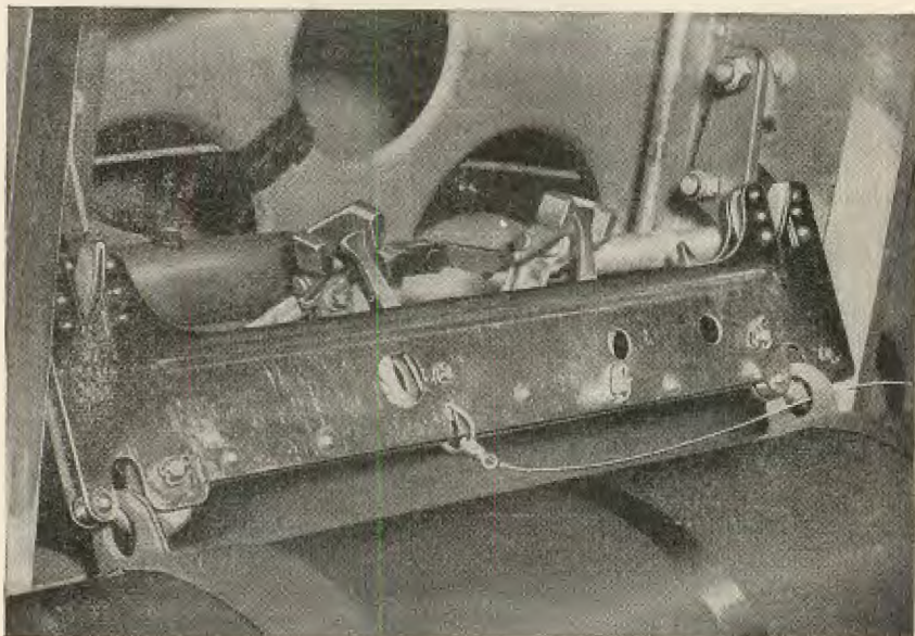
FIGURE 20.—Horizontal suspension of 100-pound incendiary bomb M47 in bomb bay of airplane.
