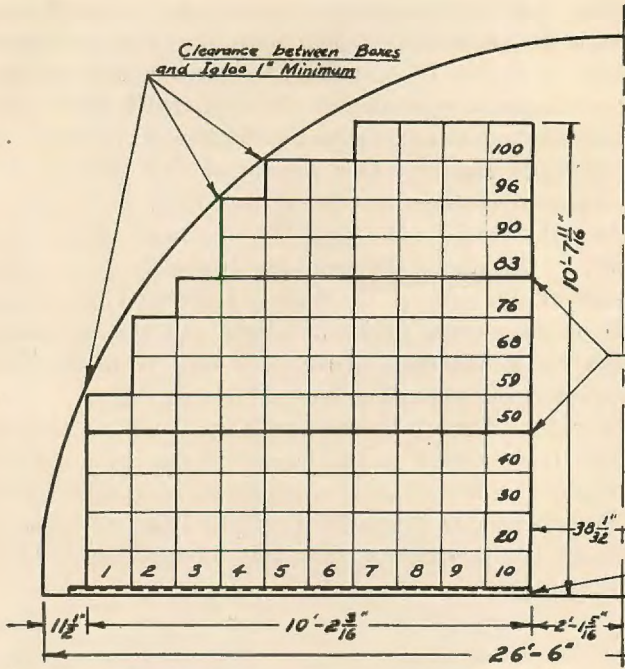
LEFT STACK ELEVATION—100 BOXES
