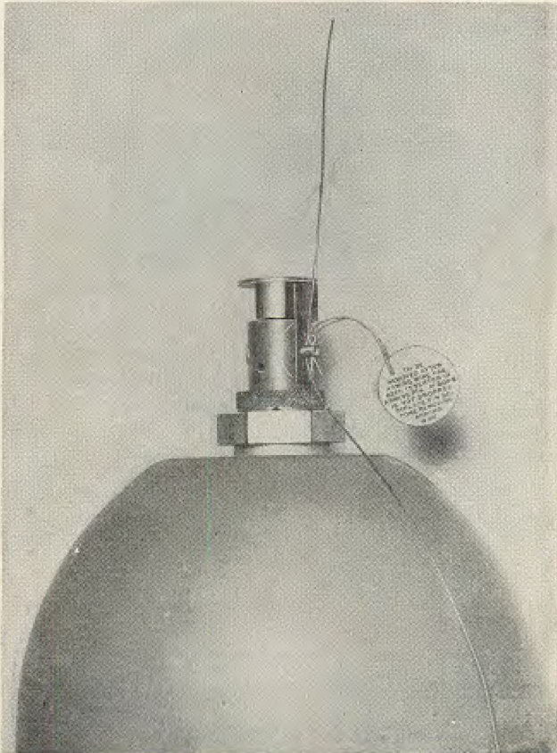
FIGURE 17.—Detail of fuze with safety block of 100-pound incendiary bomb M47.
