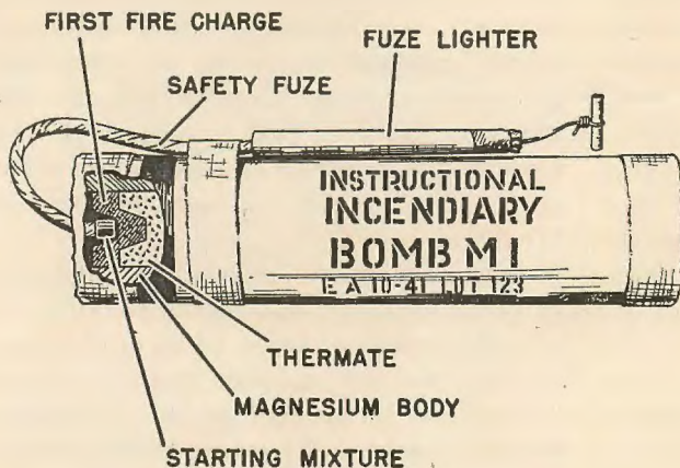
FIGURE 27.—Instructional incendiary bomb M1.
