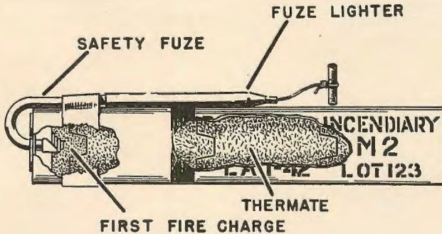
FIGURE 28.—Instructional incendiary bomb M2.
