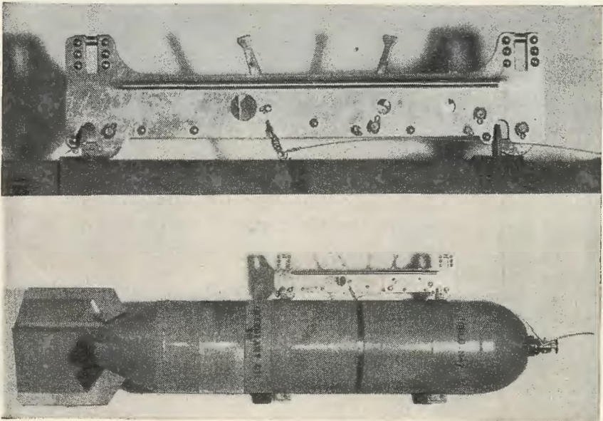
FIGURE 19.—Bomb release assembly (top) and filled and fuzed 100-pound incendiary bomb M47 attached to bomb release.
