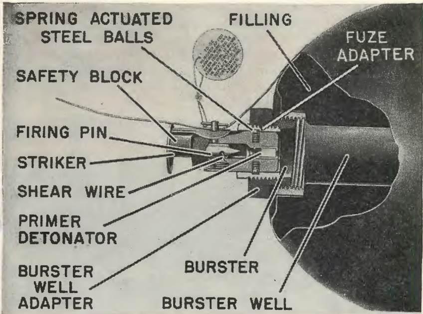
FIGURE 18.—Assembly of 100-pound incendiary bomb M47.
