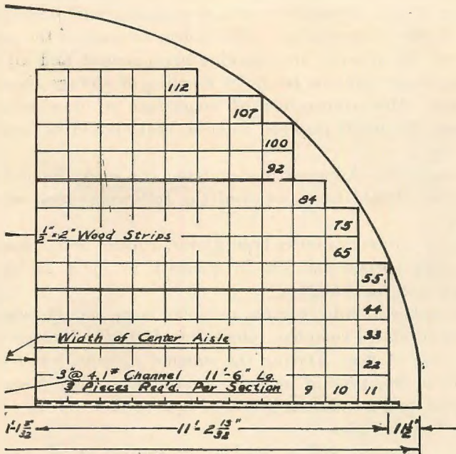
RIGHT STACK ELEVATION—112 BOXES
