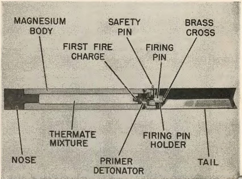
FIGURE 2.—4-pound incendiary bomb AN-M50-A1, section view.
