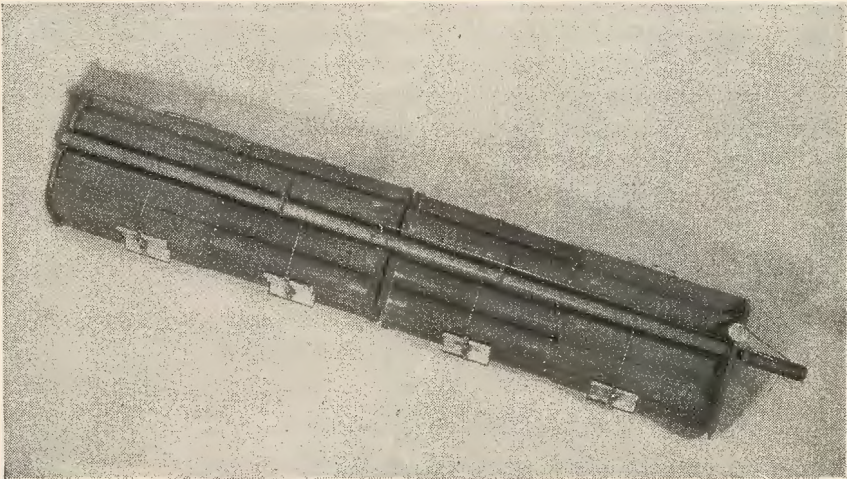
FIGURE 6.—Cluster adapter T2 (cartridge type), loaded.
