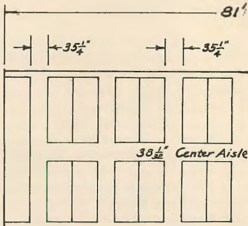
FIGURE 26.—Design of standard 81-foot reinforced concrete igloo magazine showing
