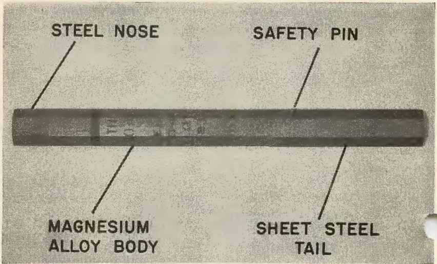
FIGURE 1.—4-pound incendiary bomb AN-M50-A1.
