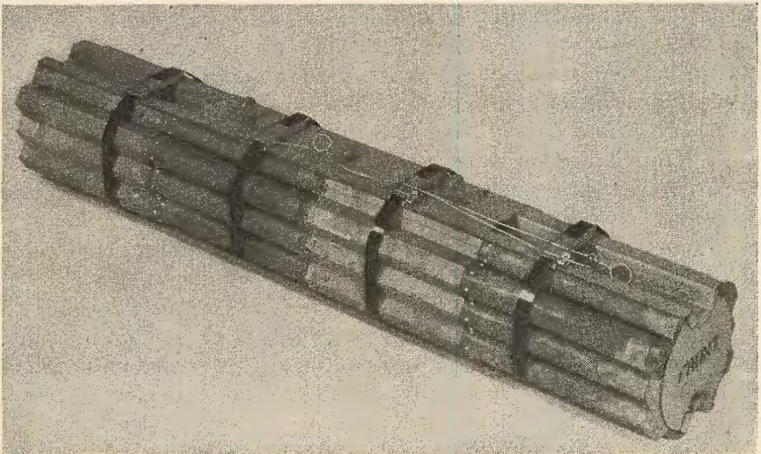
FIGURE 8.—Cluster adapter M3 (mechanical type), loaded.
