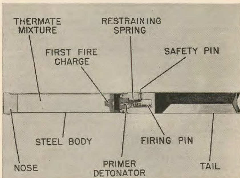
FIGURE 4.—4-pound incendiary bomb AN-M54, section view.
