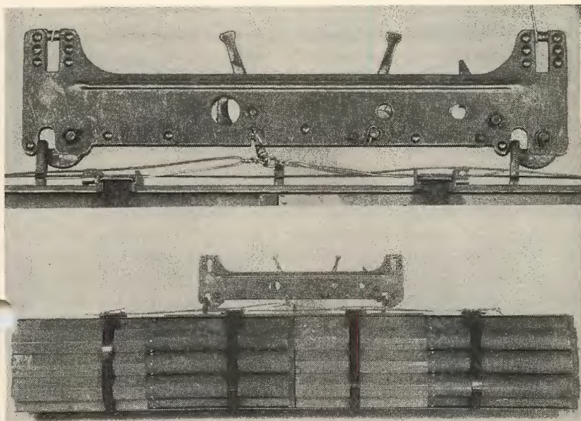
FIGURE 9.—Bomb release assembly (top) and loaded cluster adapter M3 attached to bomb release.
