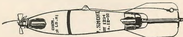
FIGURE 12.—30-pound chemical bomb M1 (WP), section view.
