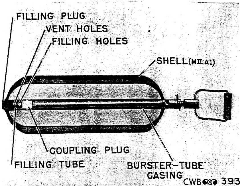
FIGURE 3.—Diagrammatic cross section of Livens shell.
