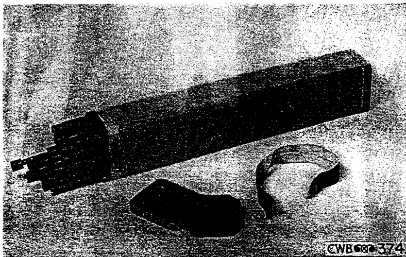
FIGURE 23.—Twenty fuze assemblies packed in tin container.
