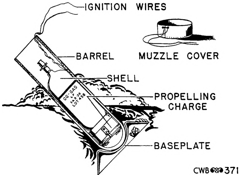
FIGURE 1.—Diagrammatic sketch, main components. Livens projector MI.
