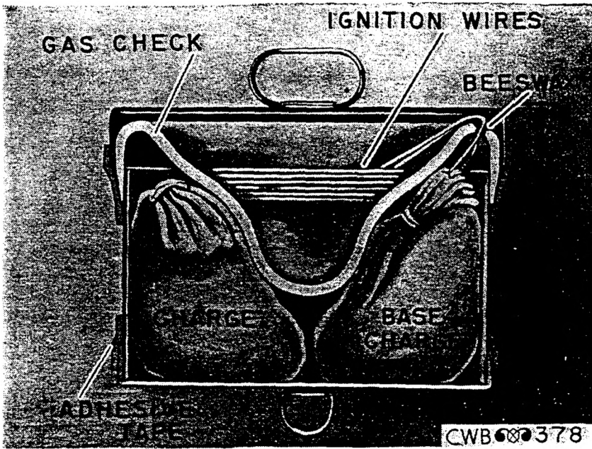
FIGURE 10.—Powder charges.
