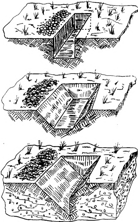
FIGURE 18.—Steps in digging trench for emplacement.
