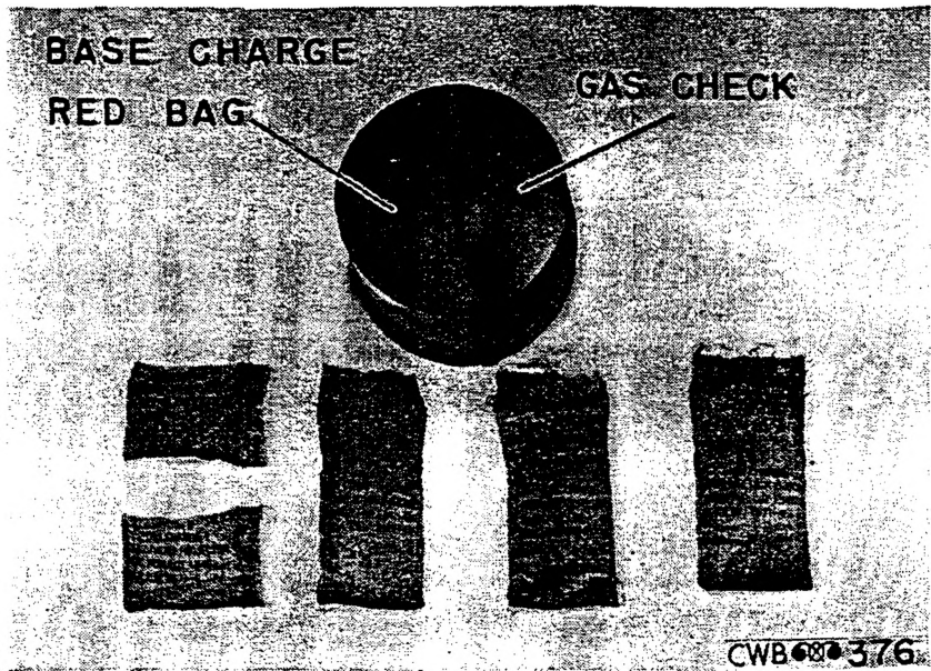
FIGURE 12.—Components of propelling charge MIII assembly.
