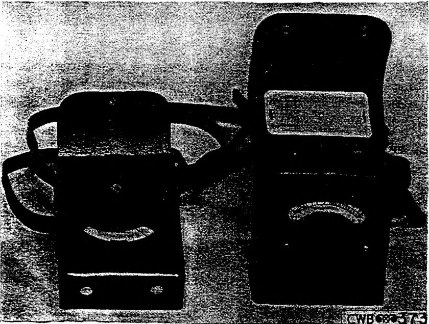
FIGURE 16.—Common types of galvanometers (circuit detectors) used with Livens projector.
