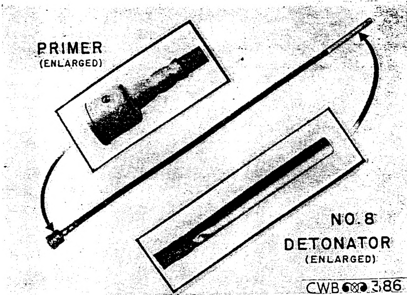
FIGURE 6.—Fuze MI assembly, showing primer and detonator.
