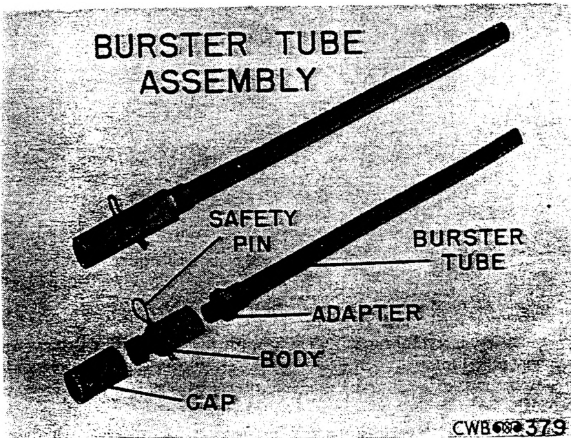
FIGURE 7.—Burster-tube MI assembly.
