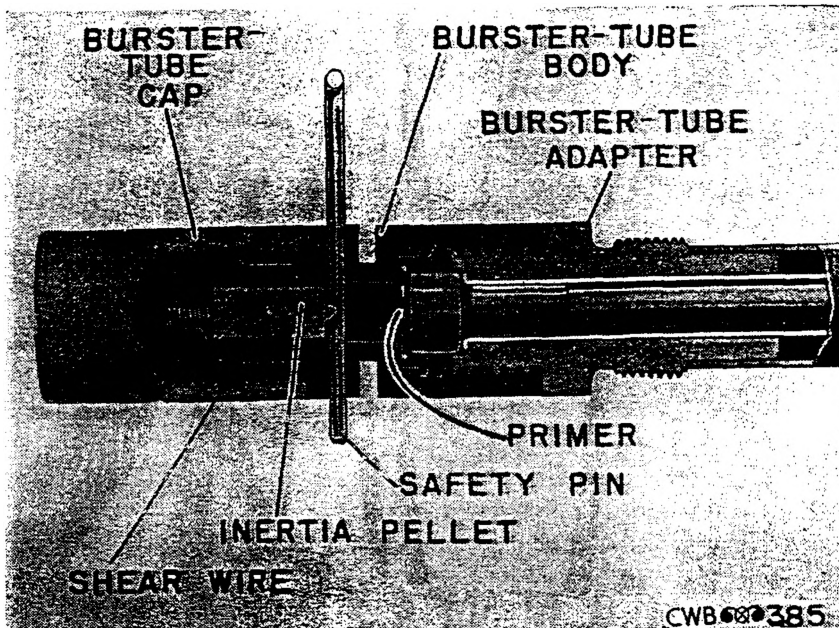
FIGURE 9.—Cross section diagram of burster-tube body.
