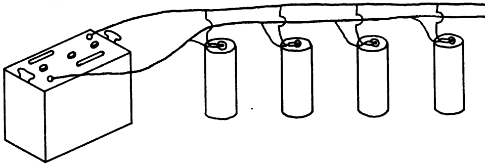
② Battery (Parallel)
