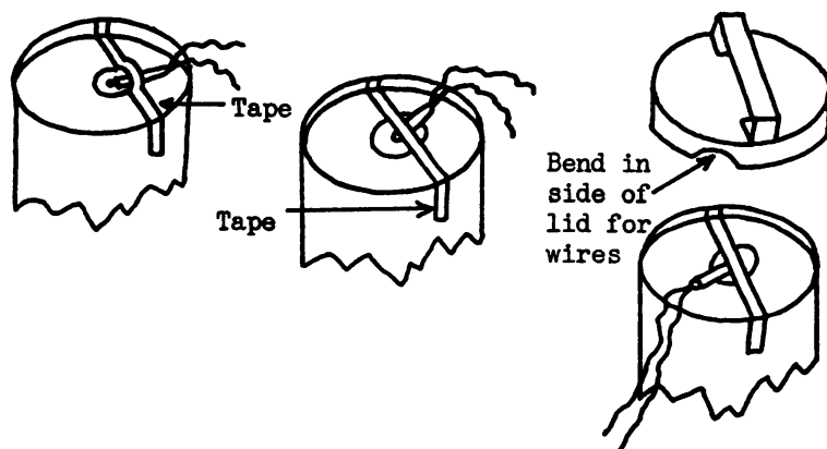
FIGURE 4.—Method of attaching squib.
