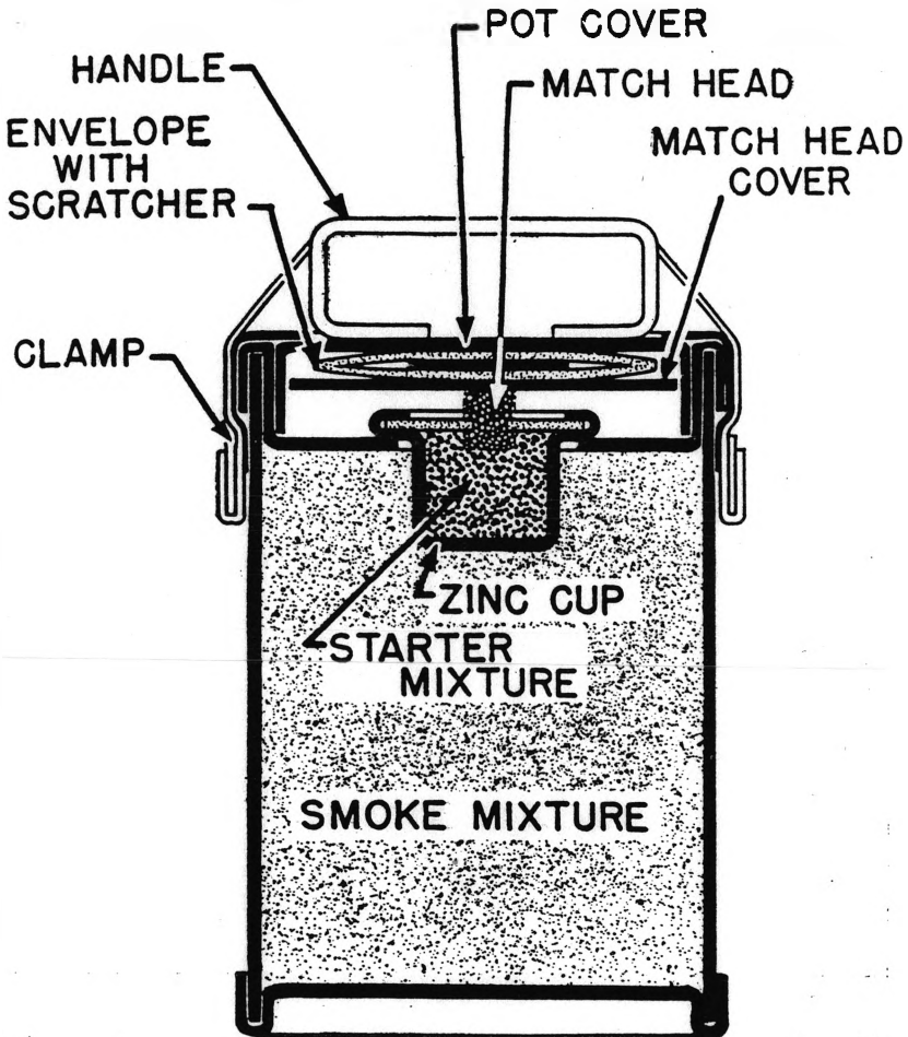
FIGURE 5.—HC smoke pot—sectional diagram.
