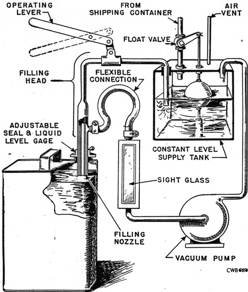
FIGURE 18.—Constant level filling apparatus, land mine.
