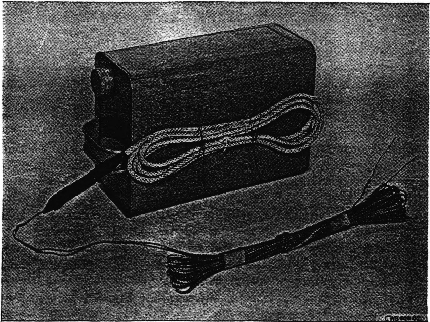
FIGURE 17.—Land mine detonating cord burster, with detonator attached, and lead wire.
