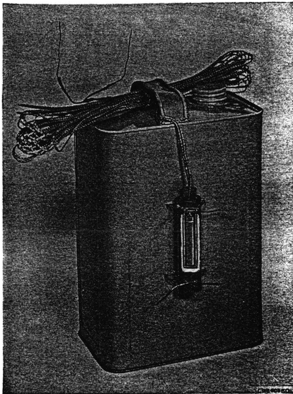
FIGURE 15.—Land mine and nitrostarch burster.
