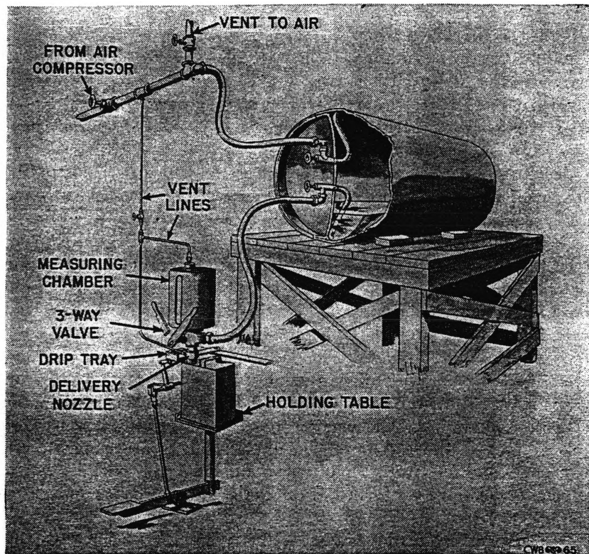
FIGURE 19.—Constant volume filling apparatus, land mine.
