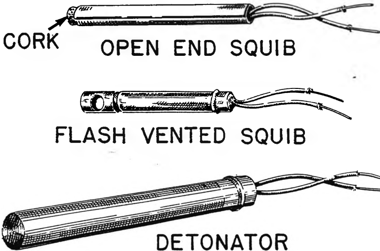
FIGURE 21.—Open end and flash vented squibs and detonator.
