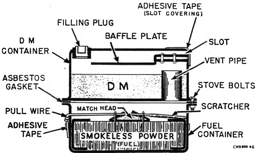
FIGURE 1.—DM irritant gas candle MI—sectional diagram.
