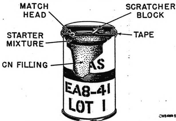
FIGURE 8.—CN tear gas pot M1—sectional diagram.
