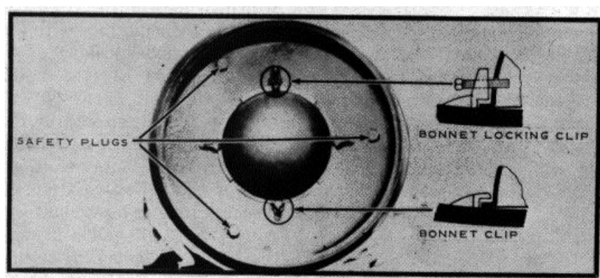
Figure 5. Shipping bonnet for 1-ton containers.
