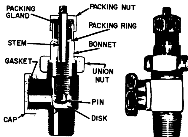
Figure 4. Angle valve.
