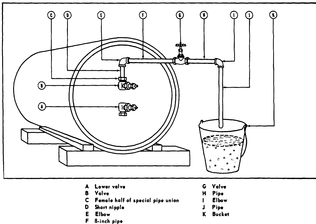
Figure 25. Venting a 1-ton container that contains a liquid chemical agent.
