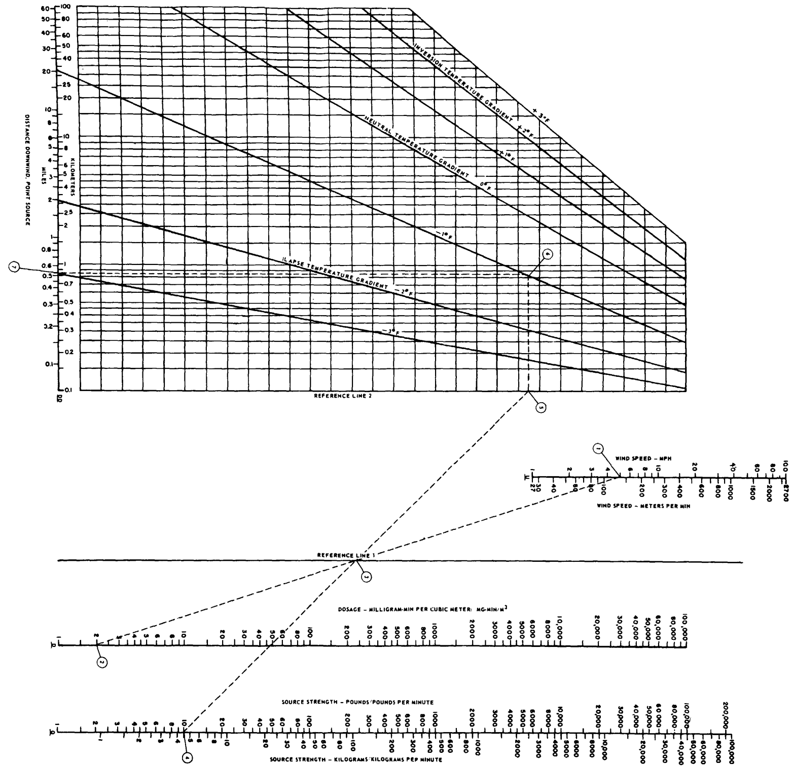
Figure 88. Point source downwind toxic vapor hazard nomgram
