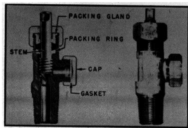
Figure 3. Needle valve.
