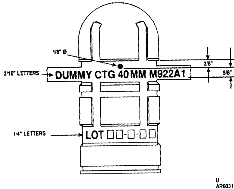
Figure 2. Typical marking for 40mm dummy cartridge M922A1.
