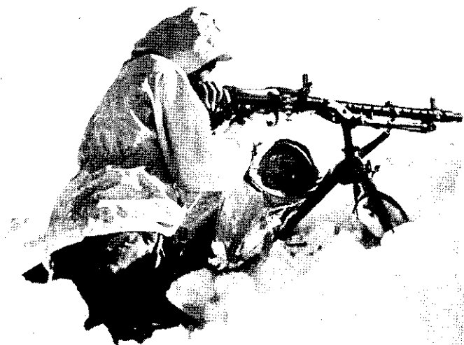
Figure 3.—Machine gun (M.G. 34) emplaced in snow. (The long-legged antiaircraft tripod is used instead of the standard mount so that the gun may be firmly emplaced in the deep snow.)
