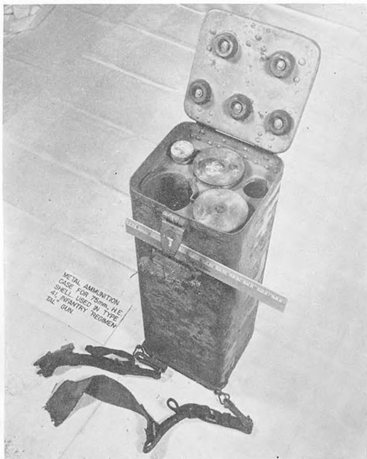
Figure 152.—Metal carrying case for 75-mm high-explosive shells (three complete rounds).
