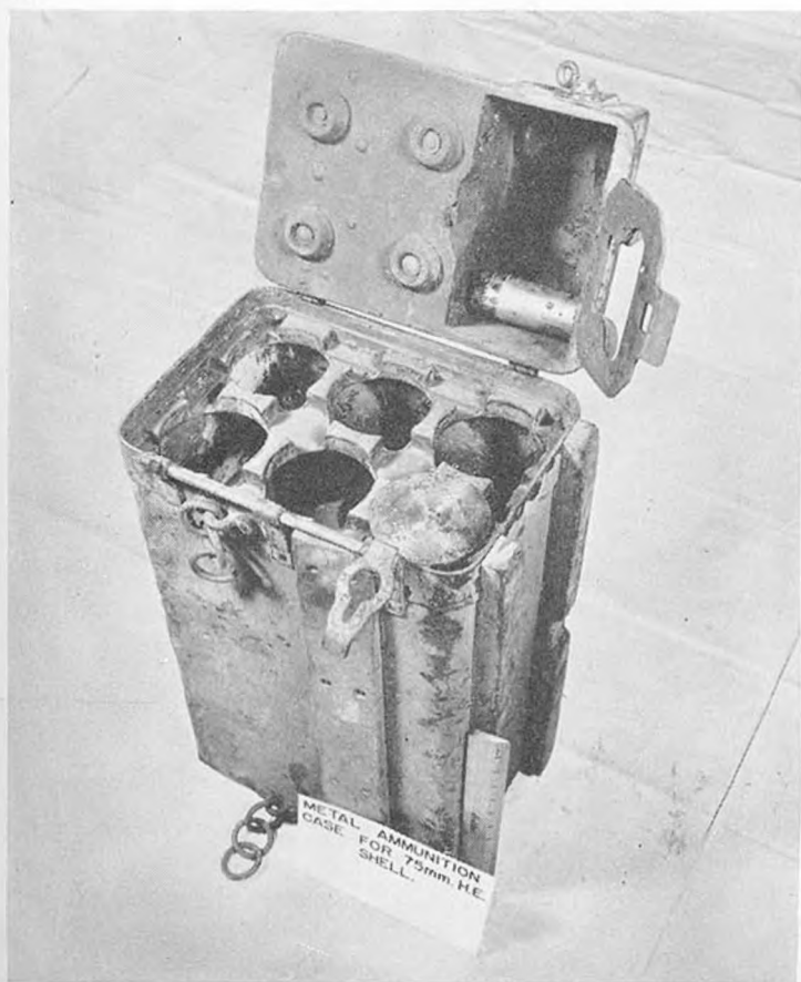
Figure 153.—Metal carrying case for 75-mm high-explosive shells (six complete rounds).
