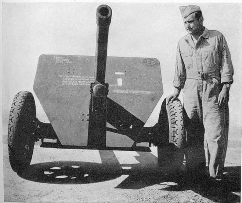
Figure 134.—Model 1 (1941) 47-mm gun (front view).
