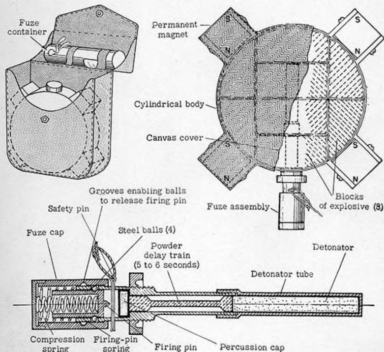
Figure 40.—Diagrammatic drawings of Model 99 (1939) armor-piercing mine (top, right) with its carrying pouch (top, left) and cross section of fuze assembly (bottom).
