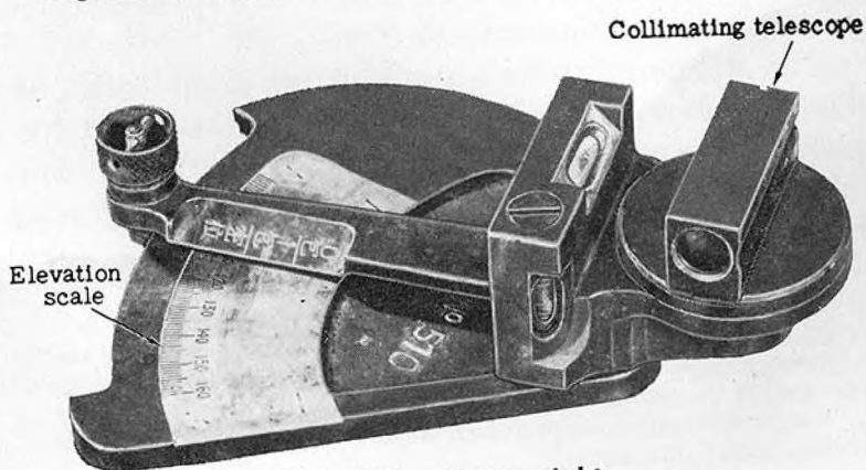
Figure 94.—Mortar sight.
