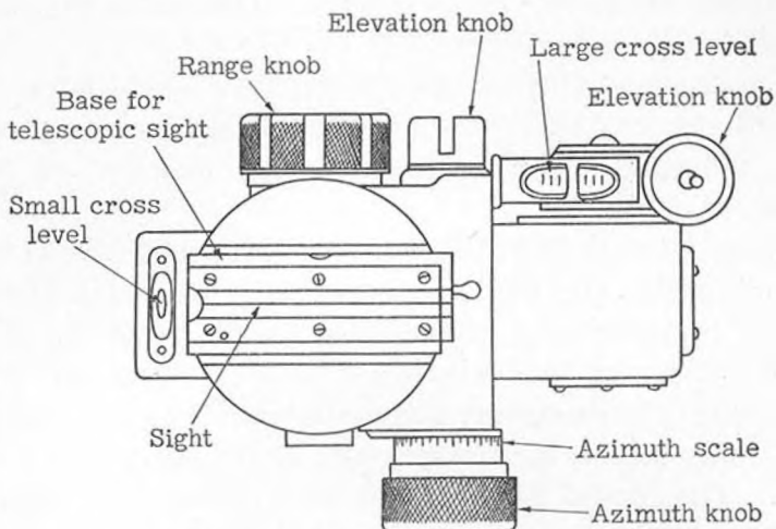
Figure 72.—Base for telescopic sight (top view).
