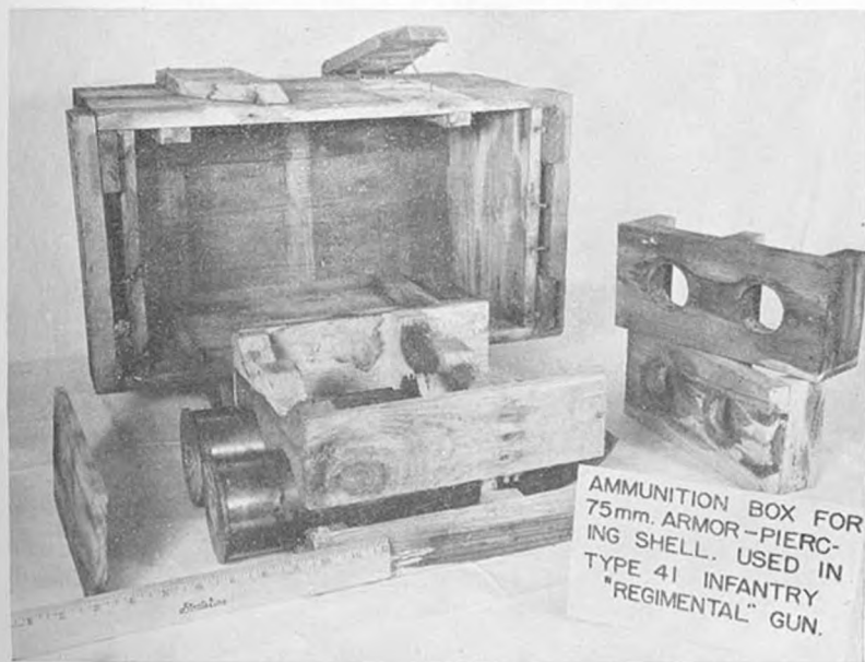
Figure 151.—Packing box for 75-mm armor-piercing shells (four complete rounds)
