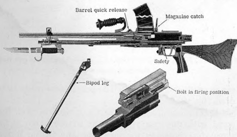
Figure 62.—Diagrammatic cross section of Model 96 (1936) 6.5-mm light machine gun, showing also various parts.
