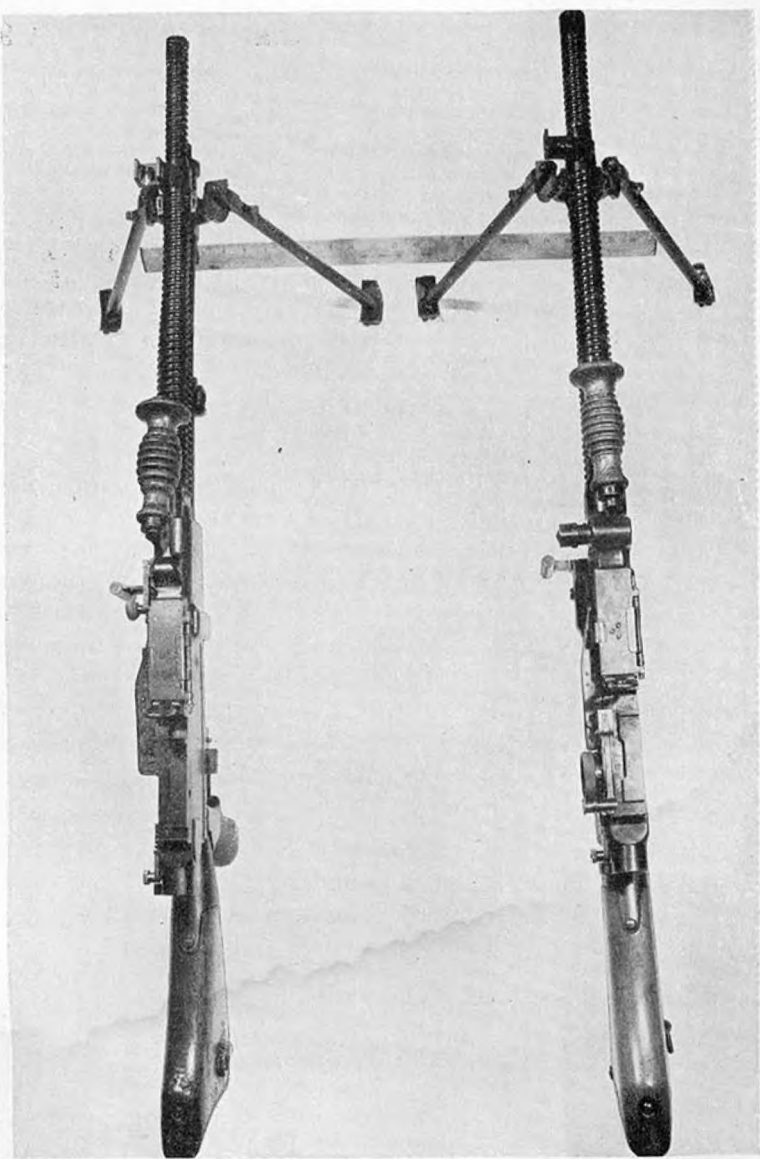
Figure 67.—Model 96 (1936) 6.5-mm light machine gun (left) and model 99 (1939) 7.7-mm light machine gun (right).
