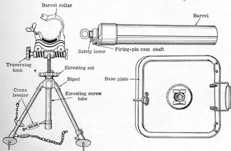
Figure 97.—Model 99 (1939) 81-mm mortar disassembled.
