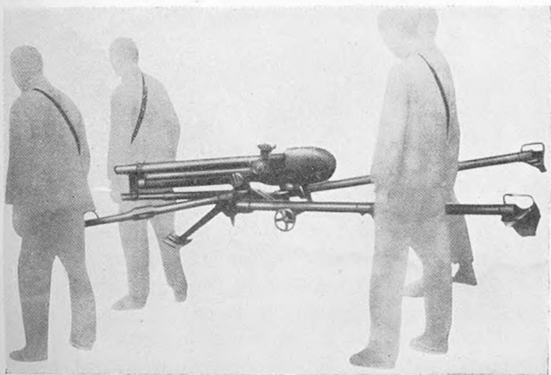
Figure 121.—Method of carrying Model 11 (1922) 37-mm gun by hand.
