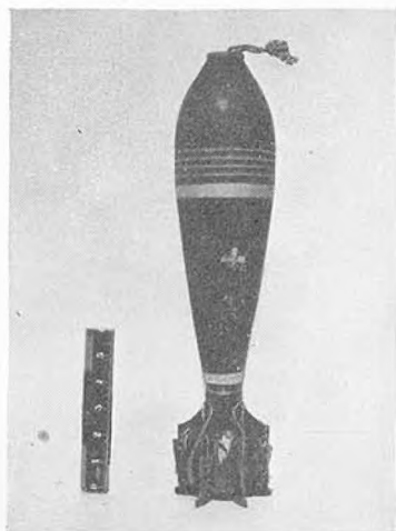
Figure 101.—Model 94 (1934) 90-mm mortar shell. (Note the propelling increments between the fins.)
