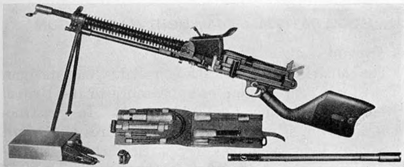
Figure 60.—Model 11 (1922) 6.5-mm light machine gun, showing also accessories.
