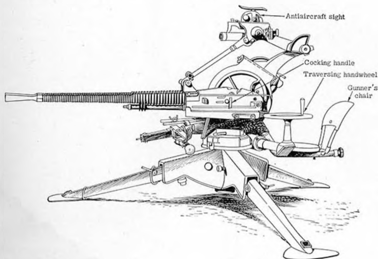
Figure 78.—Model 93 (1933) 12-mm twin heavy machine gun (left side).
