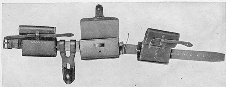
Figure 21.—Ammunition belt and pouches, and bayonet frog. (The two smaller pouches hold 30 rounds each. The larger pouch, containing 60 rounds, is worn at the rear, increasing the total for each man to 120 rounds.)
