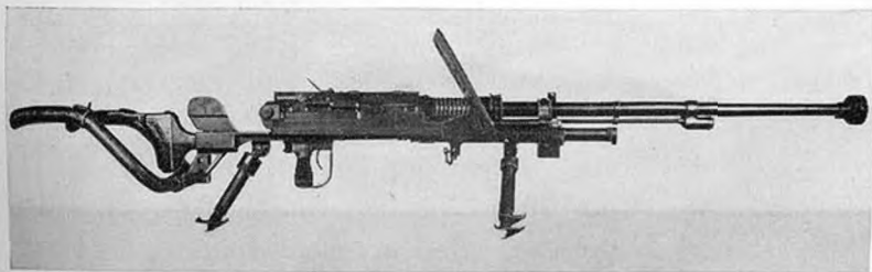
Figure 107.—Model 97 (1937) 20-mm antitank rifle with shield and rear carrying handles in place.
