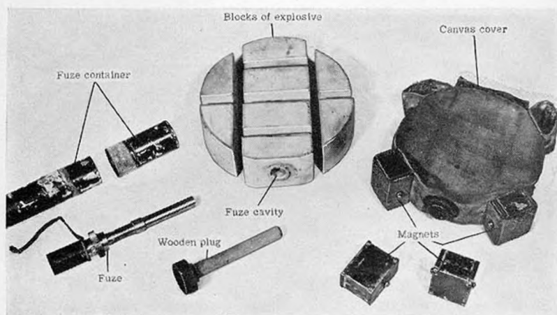
Figure 41.—Model 99 (1939) armor-piercing mine disassembled.
