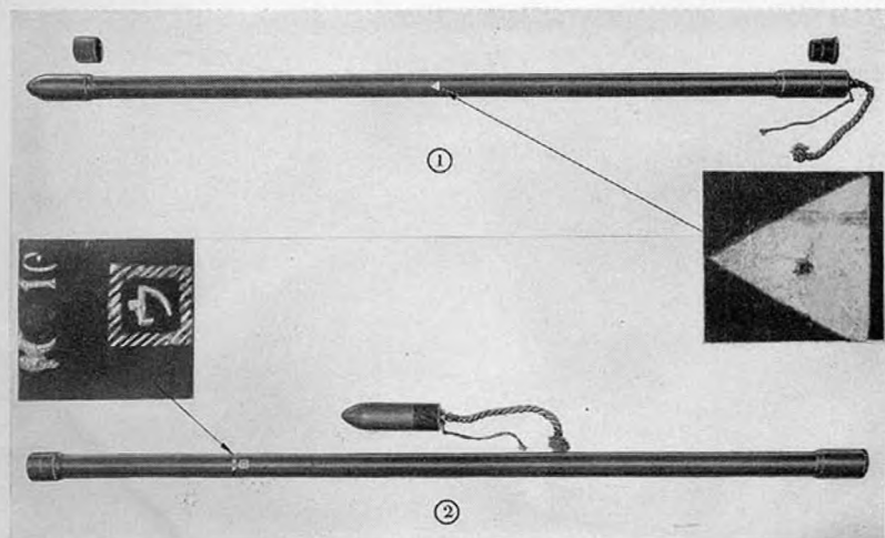
Figure 35.—Bangalore torpedo: ① ready for use and ② with fuze detached for shipment. (The markings shown were found on one torpedo.)
