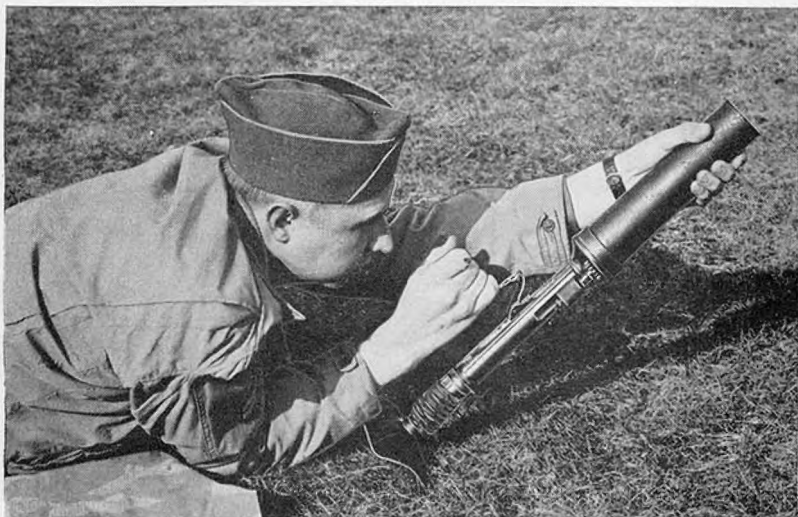
Figure 47.—Firing Model 89 (1929) 50-mm grenade discharger from prone position.
