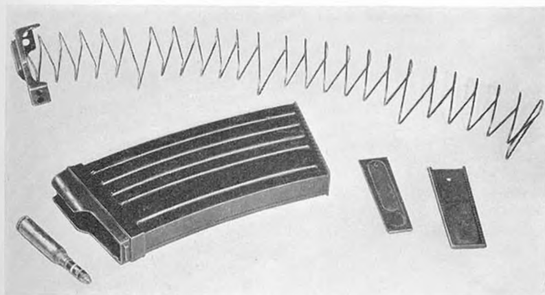
Figure 118.—Magazine of Model 98 (1938) 20-mm antiaircraft-antitank machine cannon.
