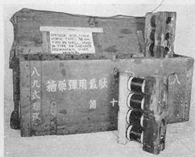
Figure 53.—Two views of packing box for Model 89 (1929) 50-mm shells, showing method of packing individual shells (40 rounds without fuzes).
