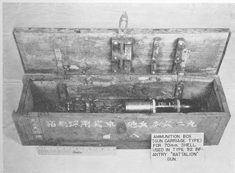
Figure 142.—Gun-carriage type of packing box for 70-mm high-explosive shells (eight complete rounds).
