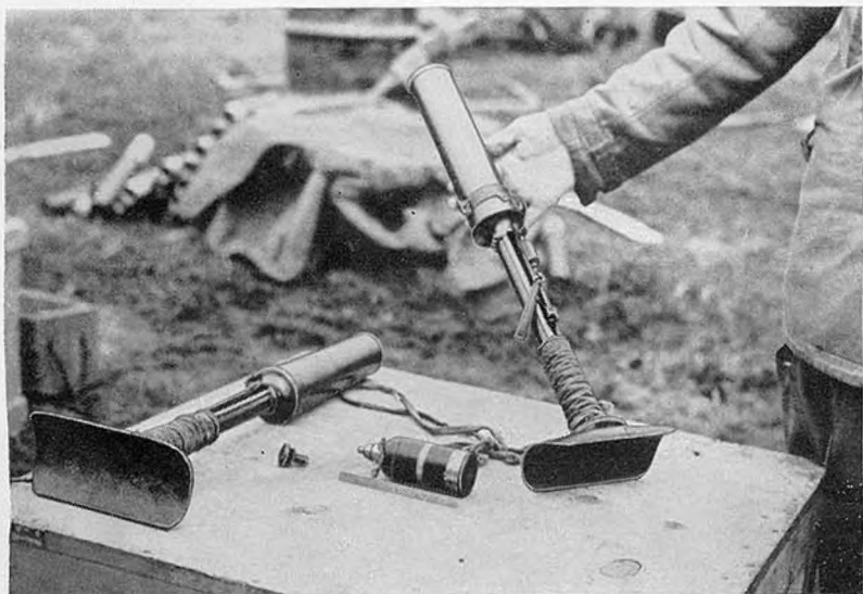
Figure 48.—Modified version of Model 89 (1929) 50-mm grenade discharger.
