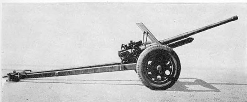
Figure 133.—Model 1 (1941) 47-mm gun (right side).
