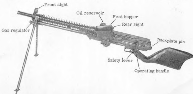
Figure 56.—Model 11 (1922) 6.5-mm light machine gun (left side).
