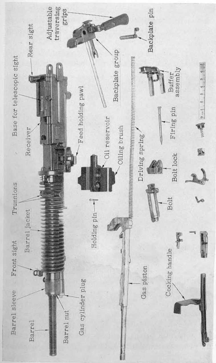
Figure 76.—Model 92 (1932) 7.7-mm heavy machine gun disassembled.
