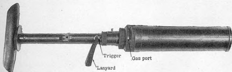
Figure 42.—Model 10 (1921) 50-mm grenade discharger.
