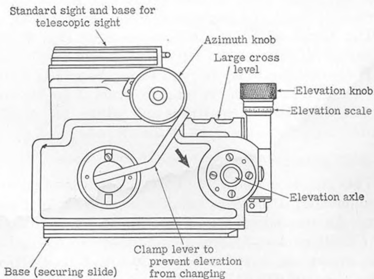
Figure 73.—Base for telescopic sight (right side).
