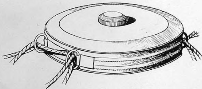
Figure 37.—Model 93 (1933) mine.
