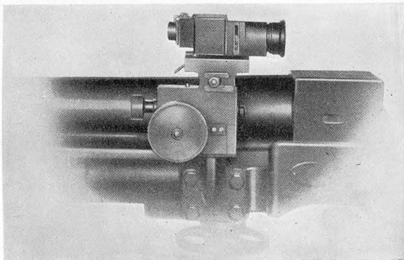
Figure 123.—Telescopic sight mounted on Model 11 (1922) 37-mm gun.
