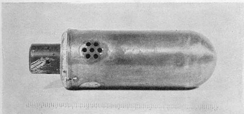
Figure 51.—50-mm incendiary grenade for use in Model 89 (1929) 50-mm grenade discharger.
