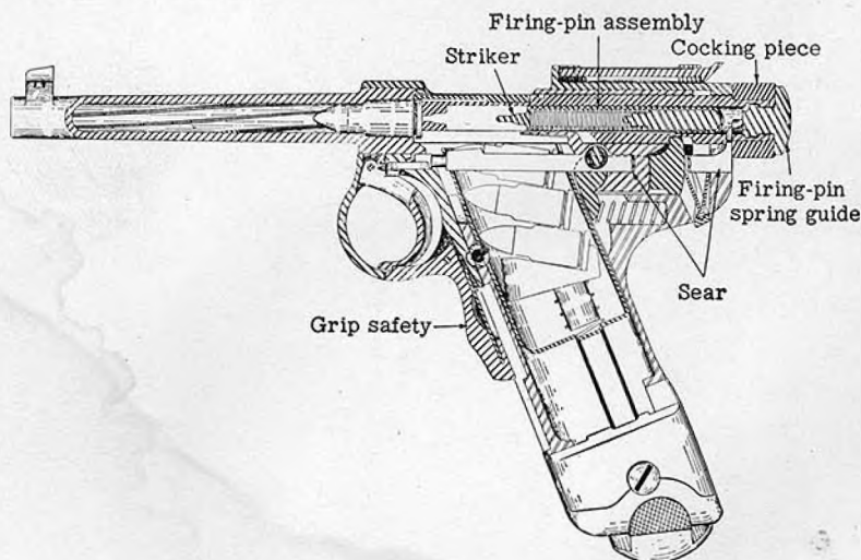
Figure 5.—Cross section of Nambu 8-mm pistol in firing position.
