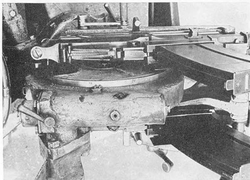
Figure 81.—Receiver of Model 93 (1933) 13-mm twin heavy machine gun as seen from above.
