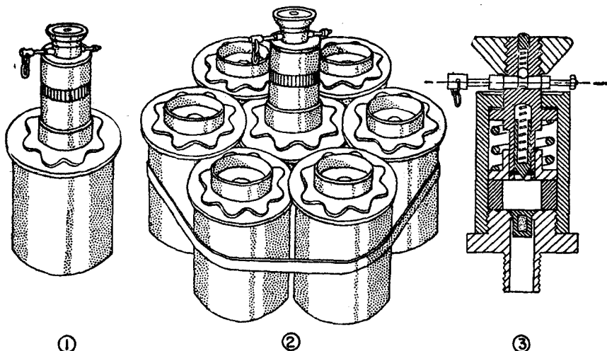
Figure 30. —① Stick grenade antipersonnel mine. (This mine is improvised from the head of a stick grenade and pressure igniter 35 ( Druckzünder 35, D.Z. 35 ), which is screwed into the head of the grenade.) ② Stick grenade cluster mine. (This mine is a variation of mine ①.) ③ Cross section of pressure igniter 35 ( Druckzünder 35, D.Z. 35 ).
