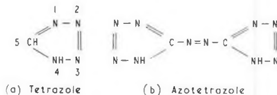
Fig. 4 Tetrazole and azotetrazole
