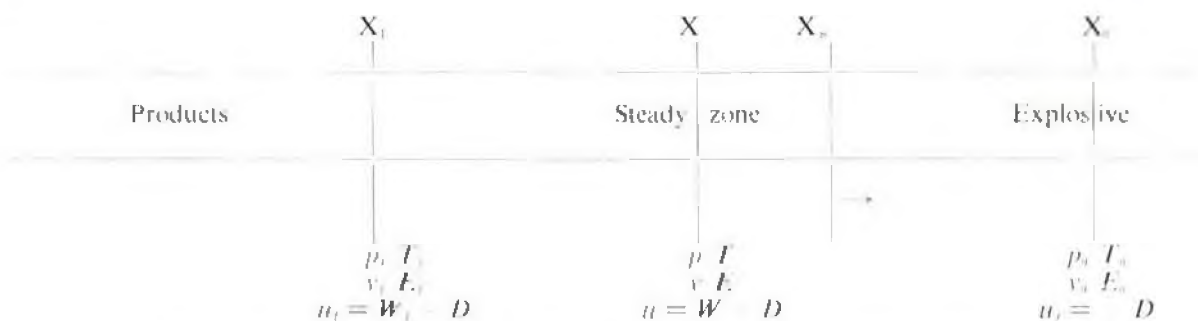
Fig. 3 A sectional diagram of the steady detonation wave from the standpoint of an observer accompanying the wave
