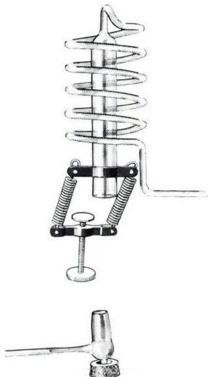
Fig. 4 Combustion tube for Will test
