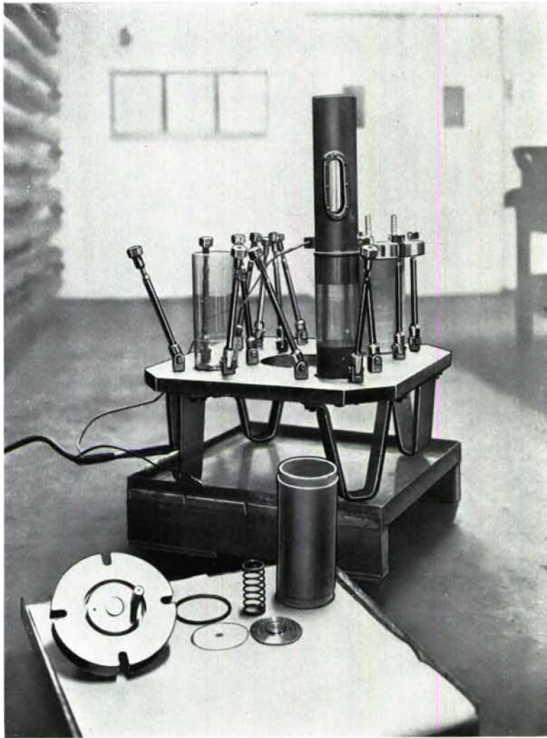
Fig 7 Casting assembly for rocket motor
