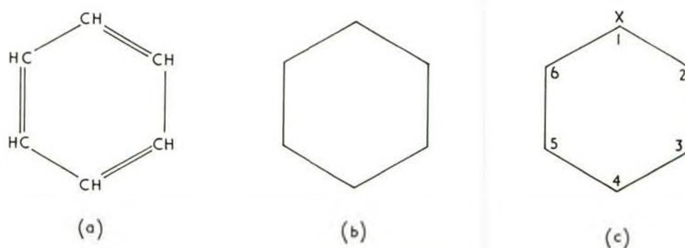
Fig. 1 Benzene-ring structure
