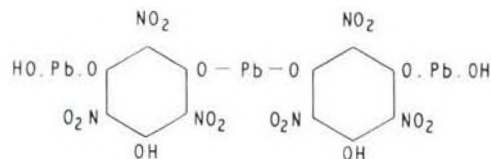
Fig. 3 Lead trinitrophenolglucinate
