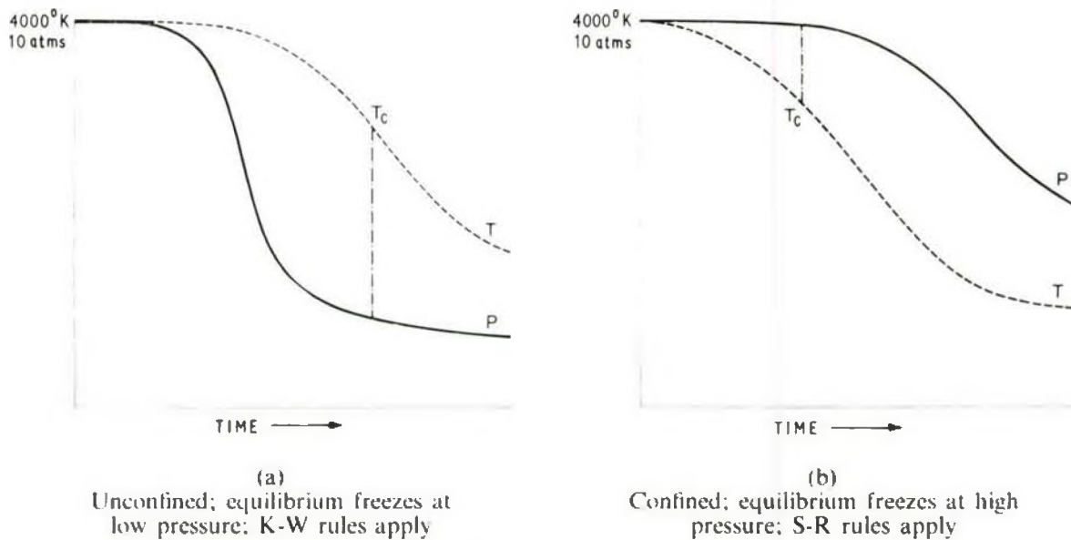
Fig. 1 Application of K-W and S-R rules to unconfined and confined explosions
