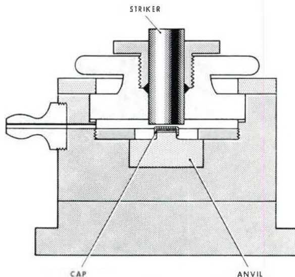
Fig. 1 Rotter impact machine chamber
