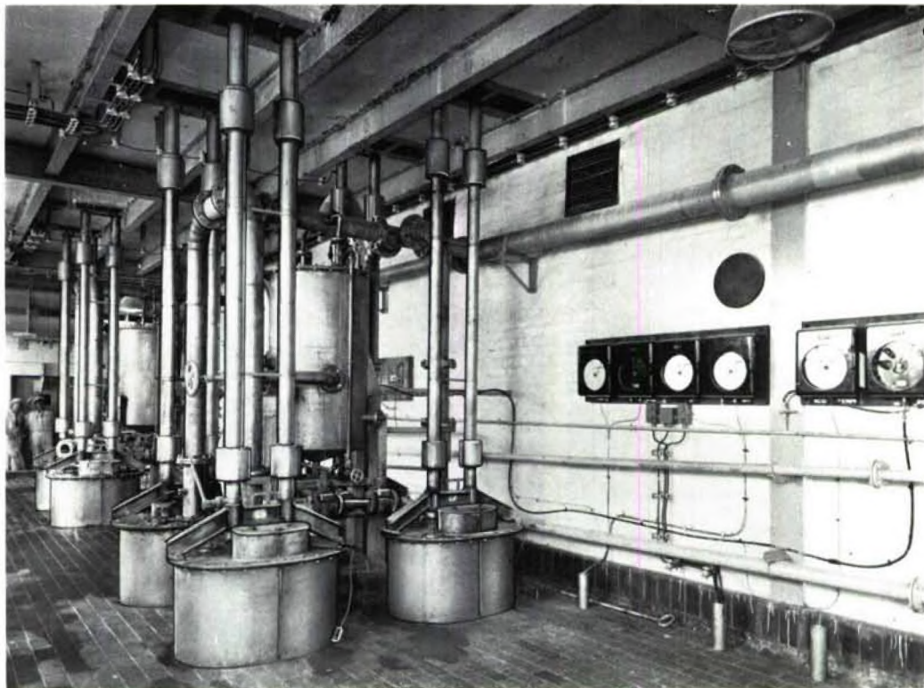
Fig. 13 Mechanical nitration
