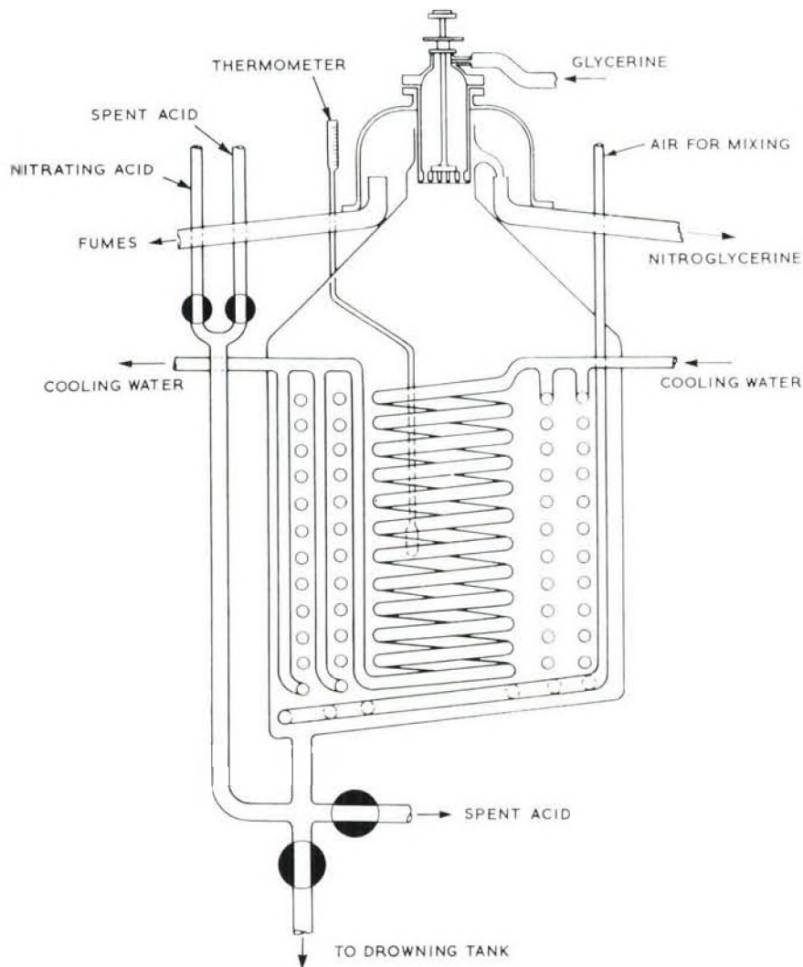
Fig. 18 Nitroglycerine manufacture
