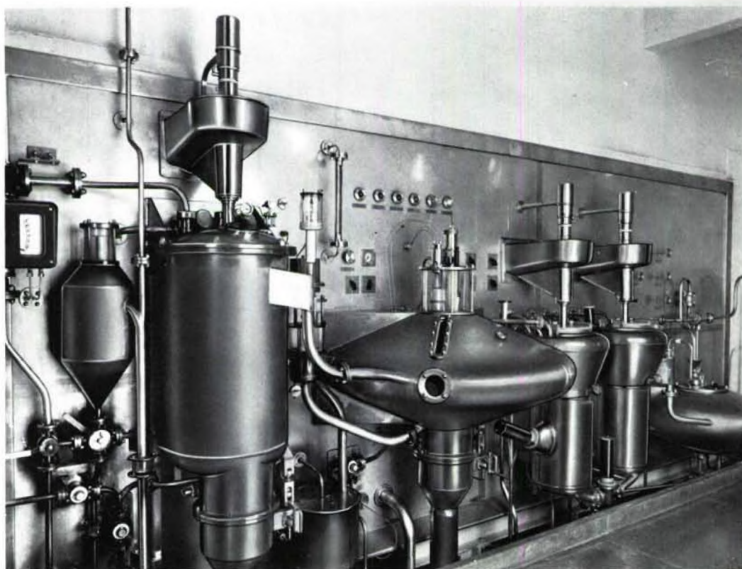
Fig. 19 Automatic Biazzi plant (Nitroglycerine manufacture)
