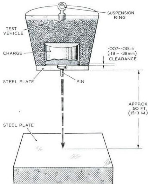
Fig. 4 Spigot-test apparatus
