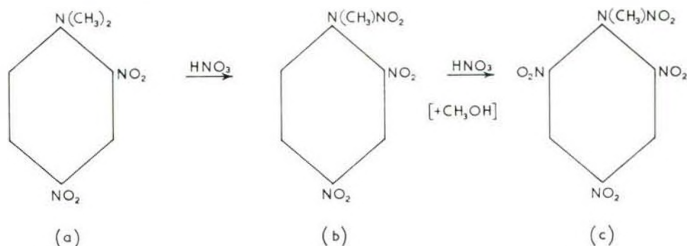
Fig. 3 Preparation of tetryl
