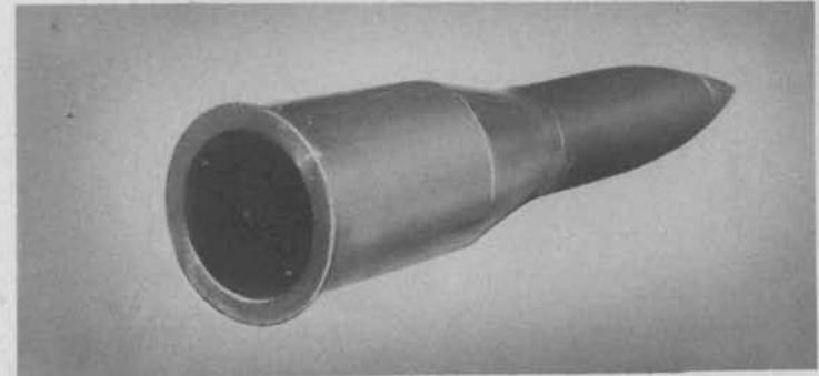
Three-quarters Rear View Showing Plastic Blow-Out Plug
