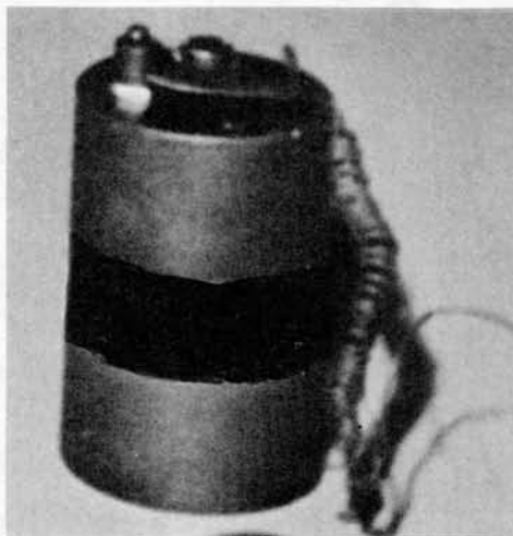
Soviet Antipersonnel Mine OZM-3 without Pull Fuze
