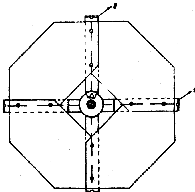
Soviet Anchored River Mine YaRM
