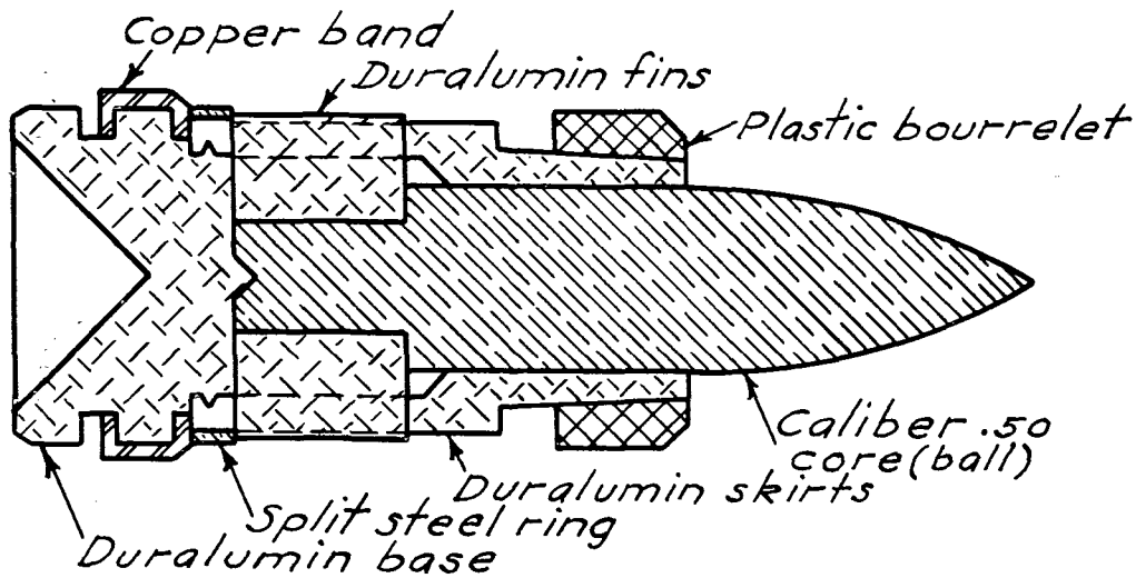
Fig. 4. The 20-mm finned projectile CF3b.
