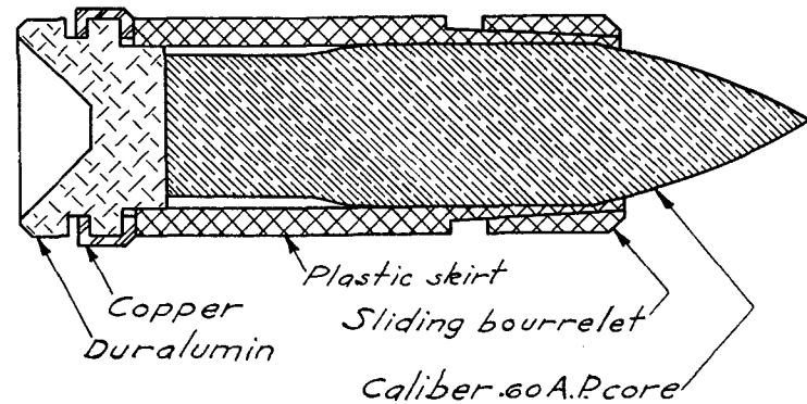
Fig. 12. 20-15 mm sabot assembly made by mounting experimental caliber .60 A.P. core in a sabot similar to CW2b.
