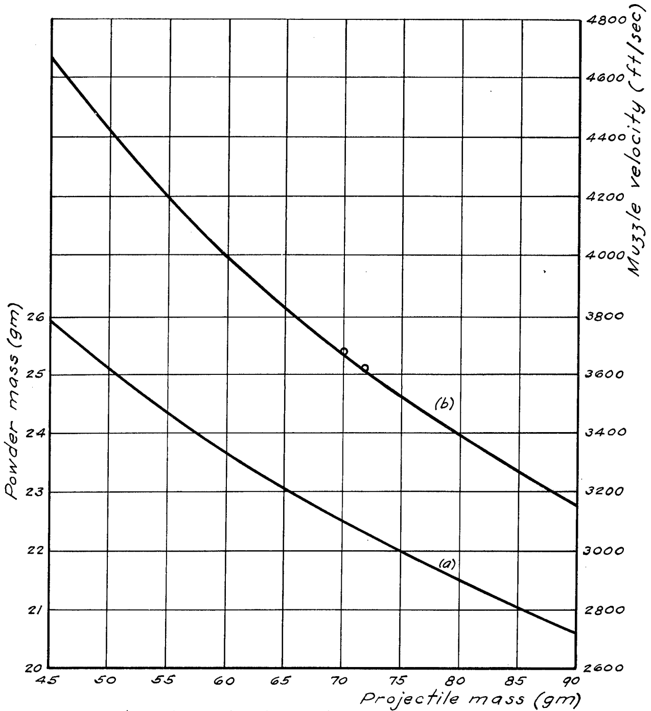
Fig. 1. Loading chart for the 20-mm Hispano-Suiza gun for Lot 4258 FNH M2, 0.015-in. web; maximum pressure, 48000 lb/in 2 ; chamber volume, 2.36 in 3 . Curve (a): mass of powder as a function of mass of projectile. Curve (b): muzzle velocity as a function of projectile mass under the assumption that the charge is that indicated by the point corresponding to the same projectile mass on curve (a).
