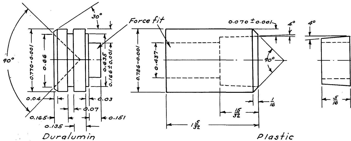
Fig. 8. Working drawings for sabot CW6. Dimensions in inches.
