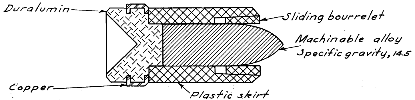
Fig. 9. Sabot assembly for the 20-11 mm type CW6.
