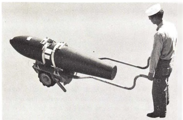
Figure 4-3. Dispenser on Aero 12B Bomb Skid With Soft-Shell Adapter Slings
