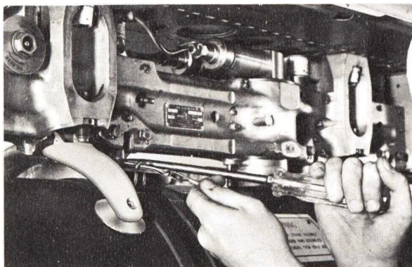
Figure 4-10. Lever Locking Pin Assembly Removed
