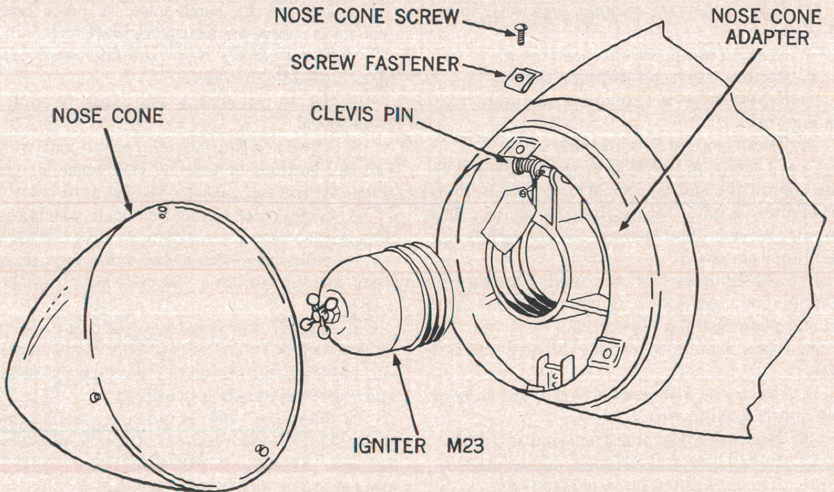
Figure 11.—Nose Cone Assembly With Igniter M23, Exploded View.
