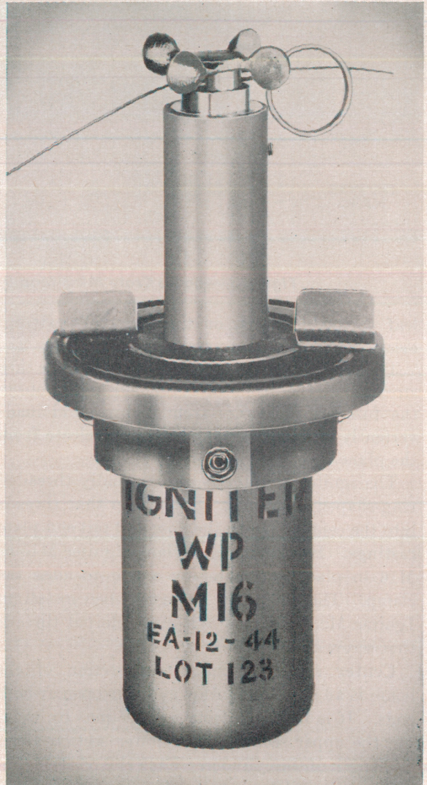
Figure 5.—Igniter M16 With Fuze M157.
