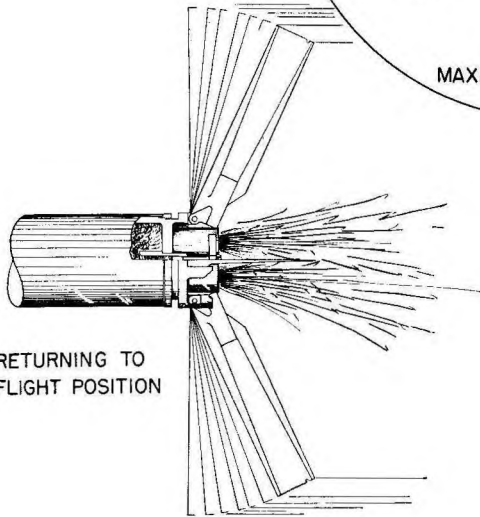
Figure 6—Phases of Fin Operation.
