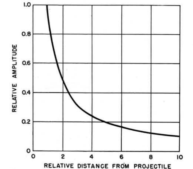
Figure 19. Variation of transmitted wave amplitude with distance from projectile.
