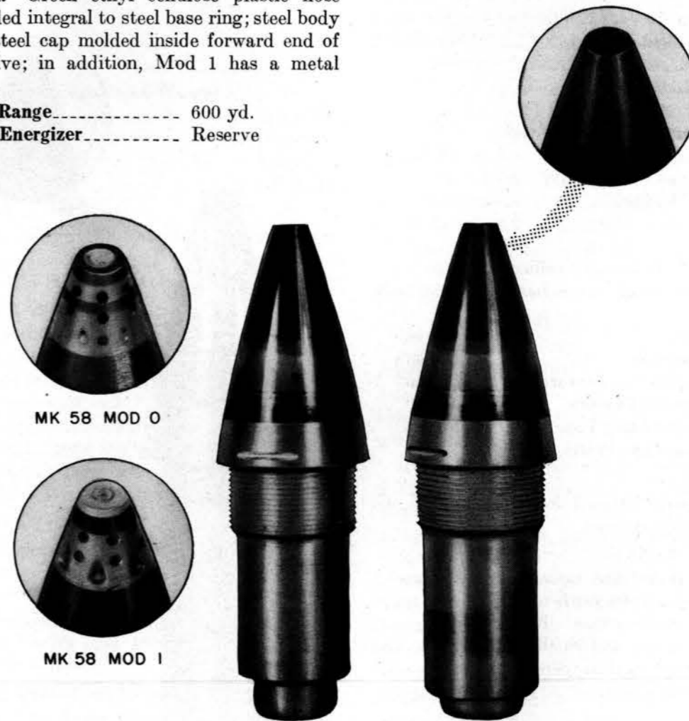
MK 58 MOD 0 MK 58 MOD 1 MK 58 MOD 2 MK 58 MODS 3 & 4 Figure 12. VT Fuze Mk 58.
