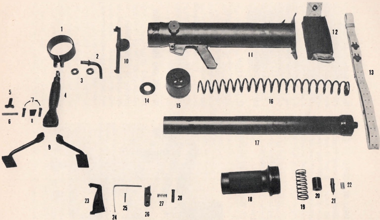
Figure 22.—Parts of the Garrett 60 mm Shoulder Mortar Mk 1 Mod 0
