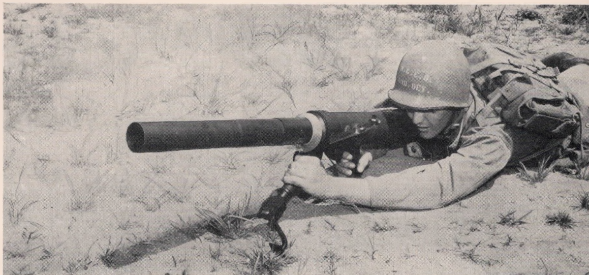
Figure 5.—Firing position with the sight aligned on the target. The gunner grasps the monopod hand grip with his left hand and moves forward until his shoulder presses firmly against the butt. The shoulder mortar must be held firmly against both recoil and counterrecoil.
