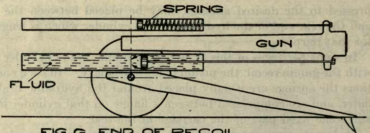
FIG. G END OF RECOIL
