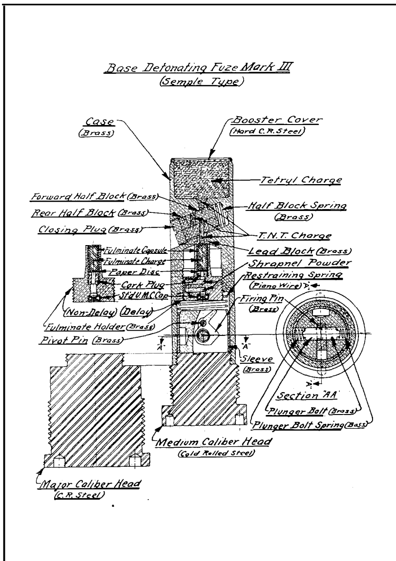
FIG. 66.—Base detonating fuze, Mark III (Sample type).
