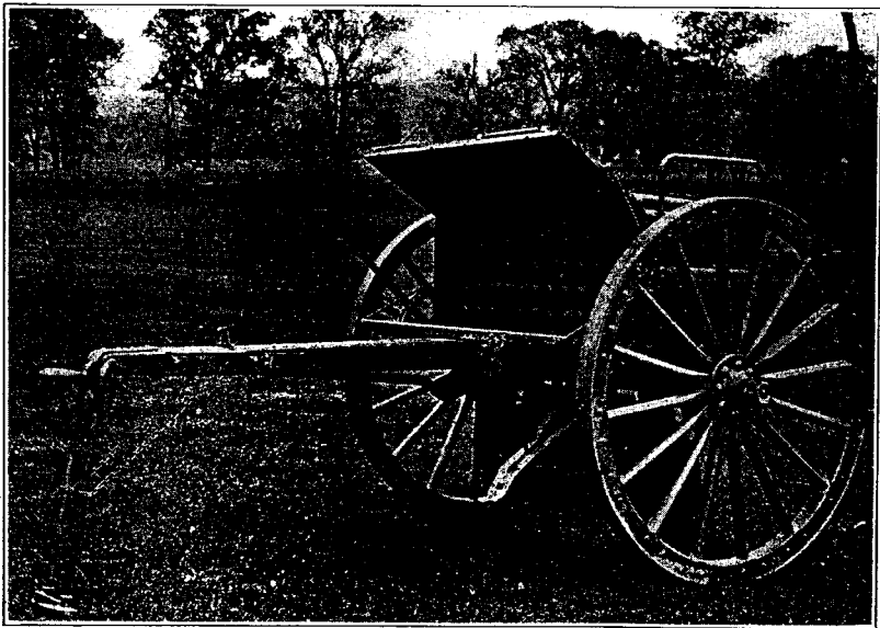
FIG. 11.—3-inch gun caisson, model of 1916, left front view, door open, apron down, fuze setter bracket down.
