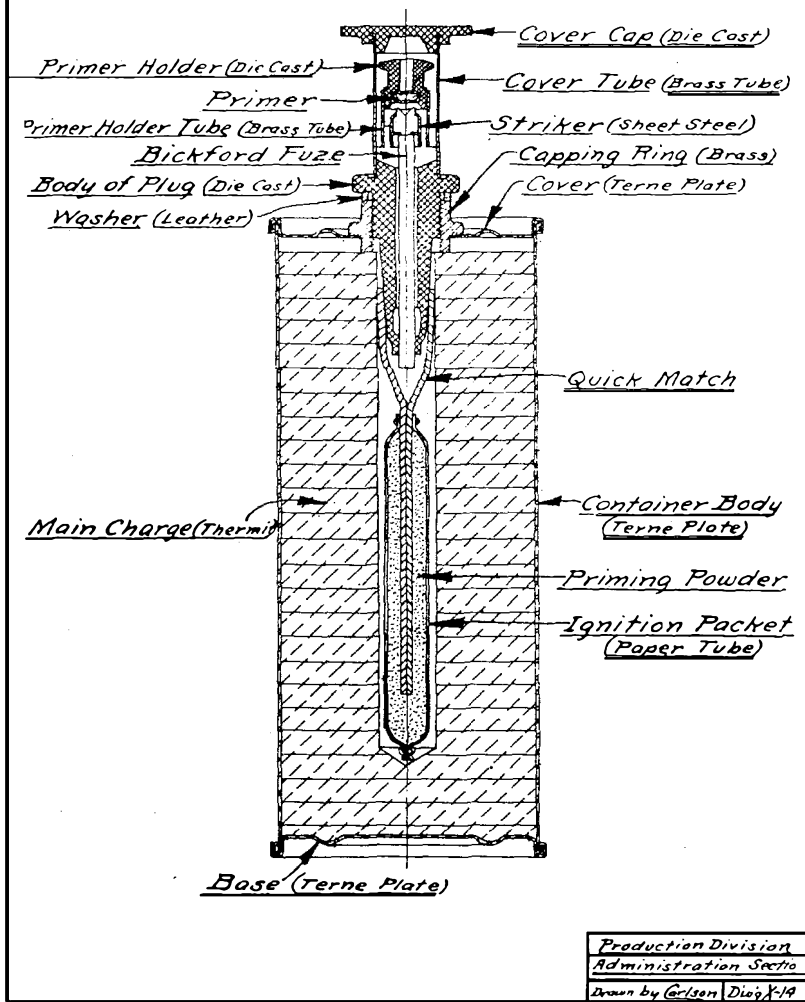
FIG. 90.—Sectional view of thermif hand grenade, Mark I.
