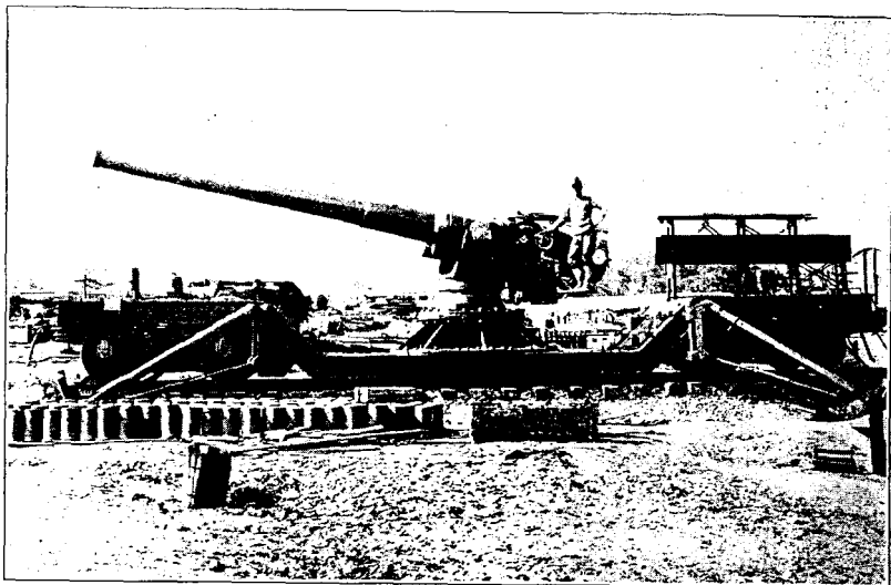
FIG. 30.—7-inch Navy railway mount, model of 1918.
