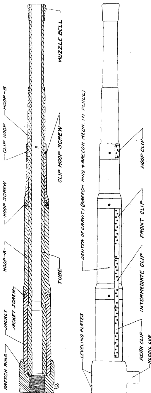
155 M.M. GUN MODEL OF 1918 (FILLoux)
