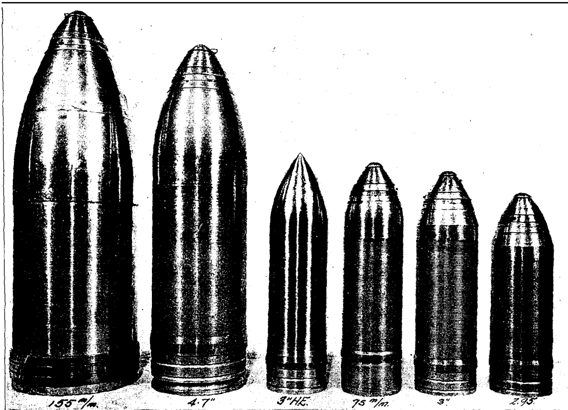
FIG. 46.—U. S. artillery ammunition. Exterior views of shrapnel and shell. Shrapnel assembled with time fuzes.
