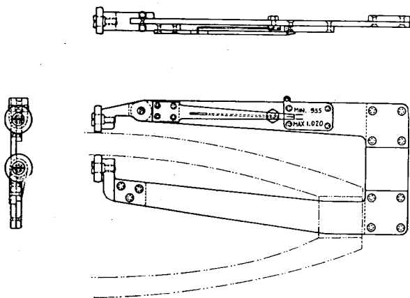
FIG. 211.—Sketch showing type of gauge used to inspect thickness of wall of shell and shrapnel.
