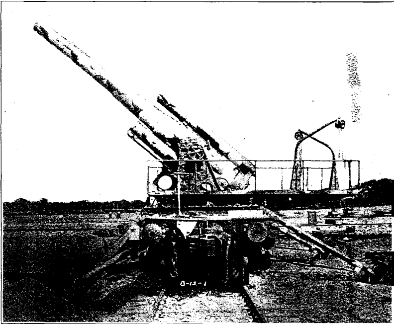
FIG. 32.—8-inch railway mount, model of 1915, arranged for firing at right angles with the track. Note the outriggers and floats.
