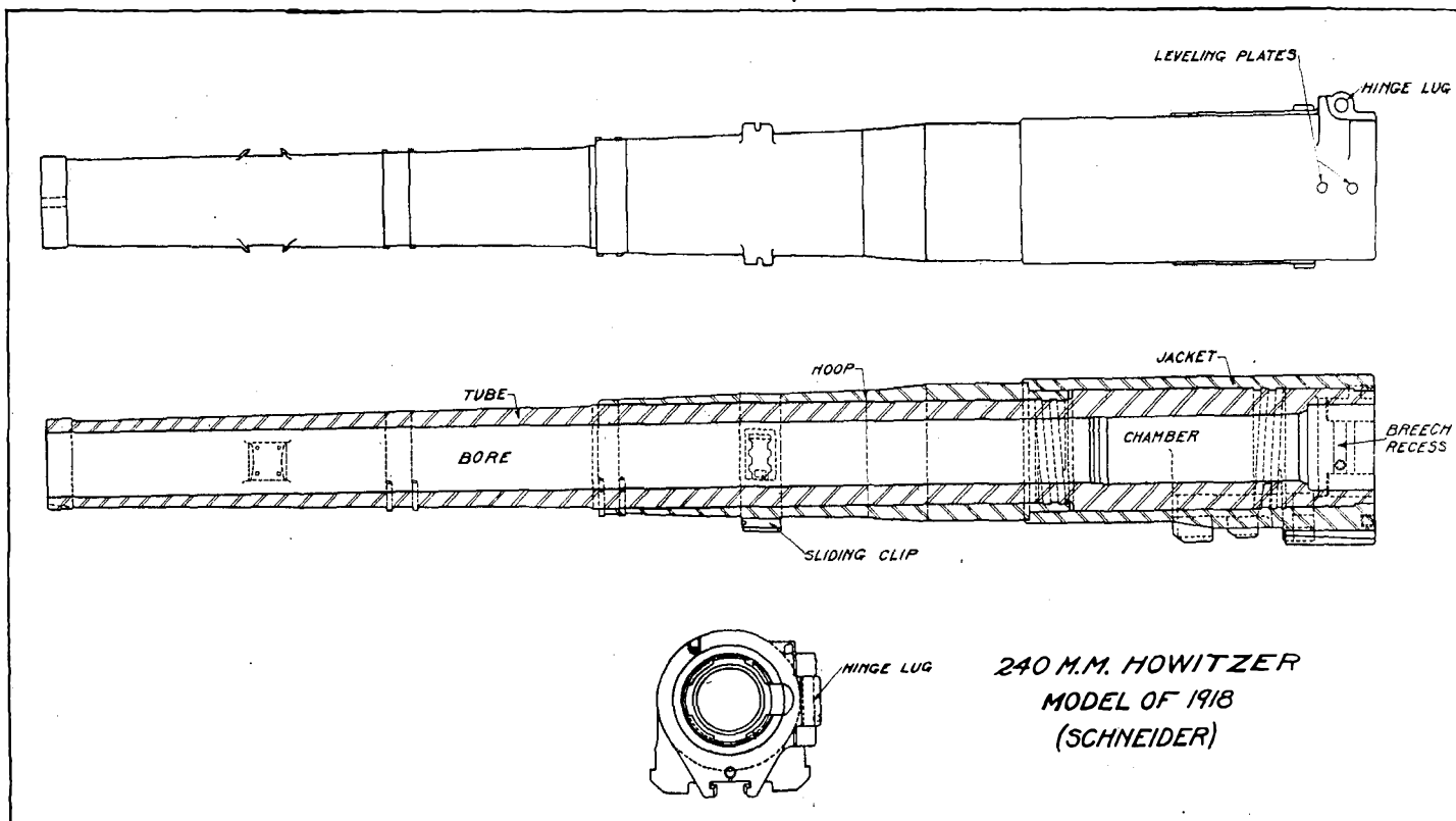
FIG. 24.—240-mm. howitzer, model of 1918 (Schneider).
