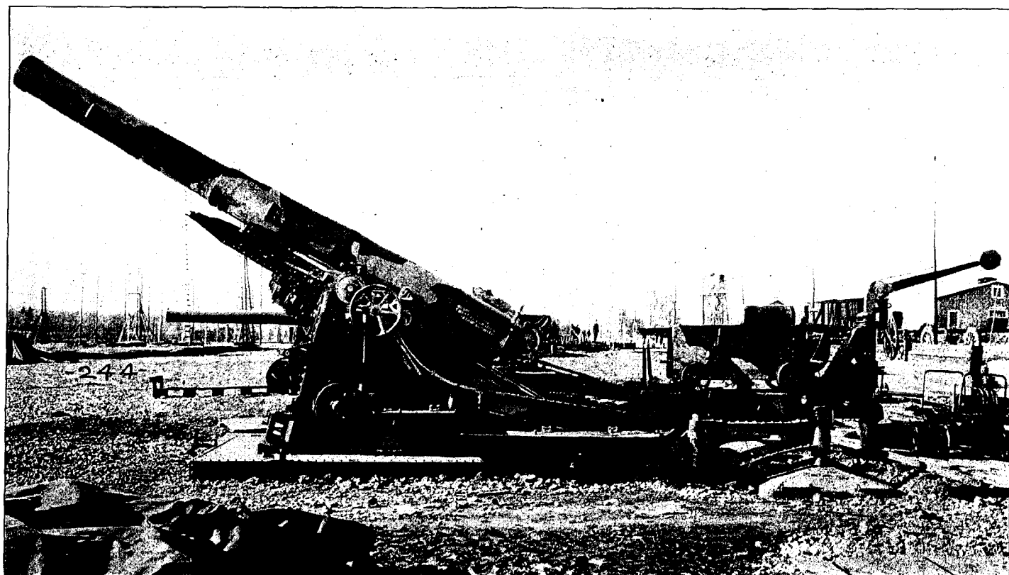
FIG. 25.—240-mm. howitzer, left side view. Elevation 30 degrees (Schneider).
