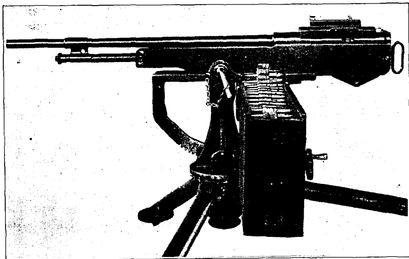
FIG. 134.—Marlin aircraft machine gun mounted on Colt tripod.
