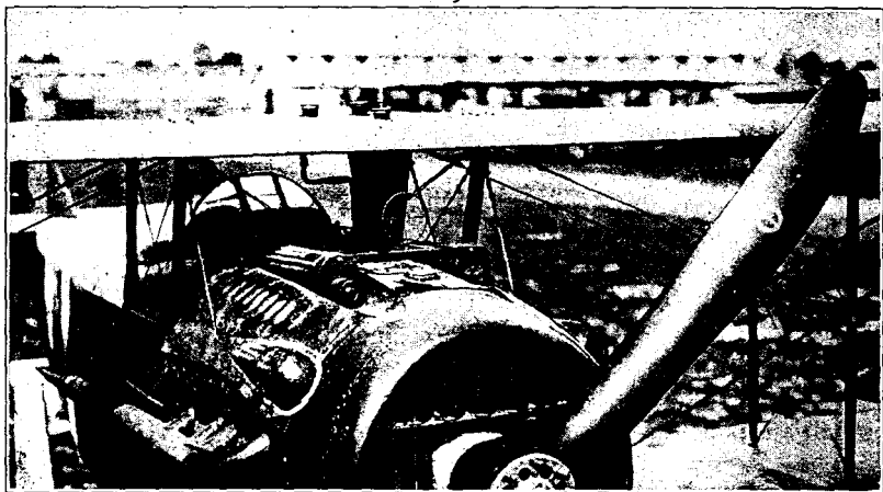
FIG. 111.—Two Vickers guns mounted parallel to motor axis of Spad XIII airplane.
