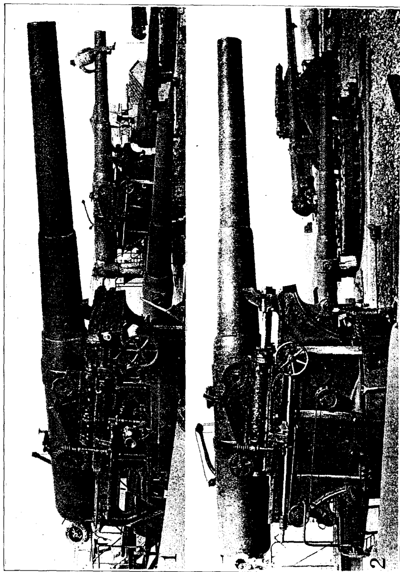
FIG. 28.—8-inch and 10-inch guns on seacoast barrette carriages. 1. 10-inch gun, model 1895. 2. 8-inch gun, model 1888.
