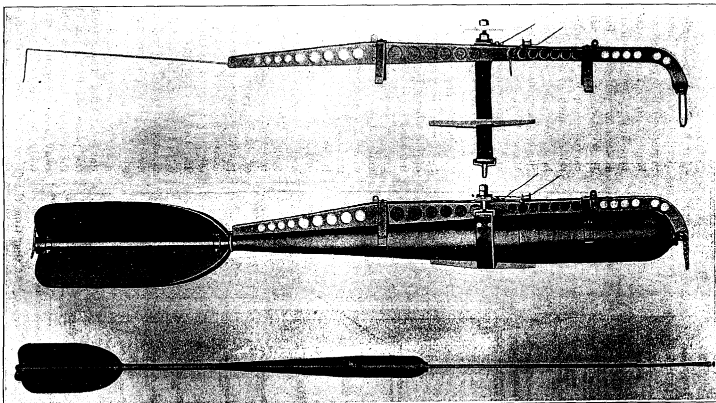
FIG. 119.—Barlow heavy drop bomb with release mechanism. Below—Barlow heavy drop bomb with rod extended.
