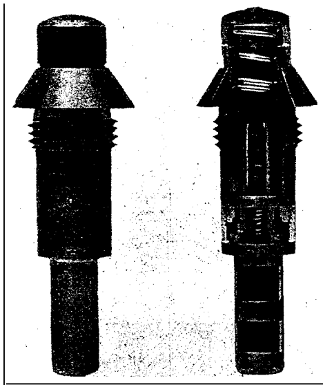
FIG. 62.—Mark V point detonating fuze, exterior view and section.
