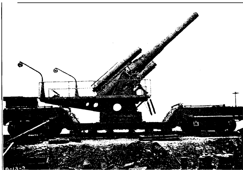
FIG. 31.—8-inch railway mount, model of 1918, showing firing platform formed by crossties laid on H-beams.
