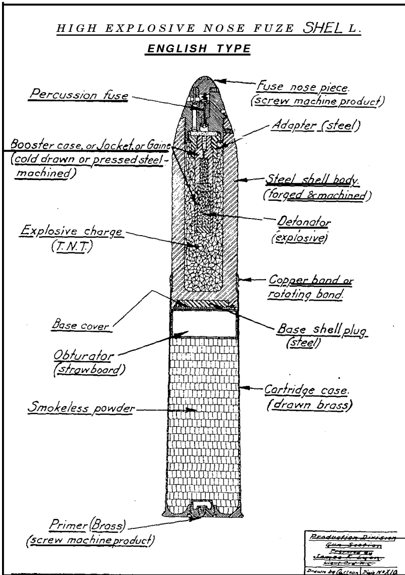
FIG. 51.—High-explosive nose fuze shell, English type.
