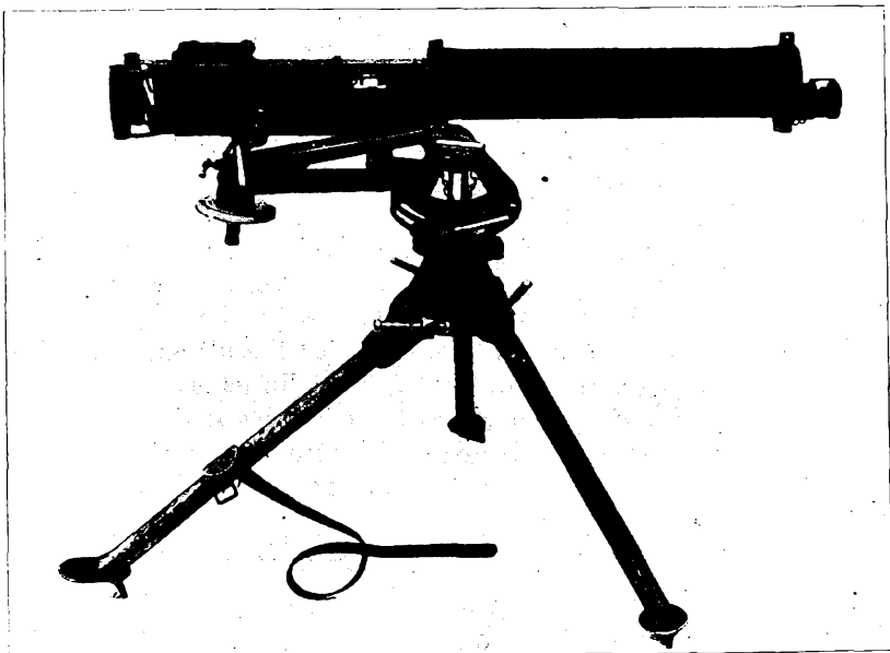
FIG. 136.—Vickers machine gun mounted on a Browning machine gun tripod, model of 1917.
