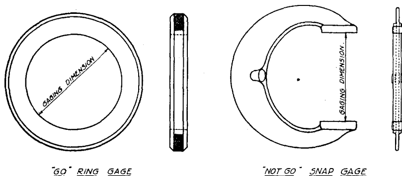
FIG. 218.—Types of ring and snap gauges.
