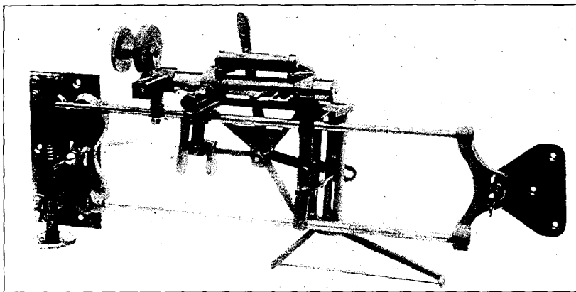
FIG. 127.—Bomb sight, Mark I-A. Side view.
