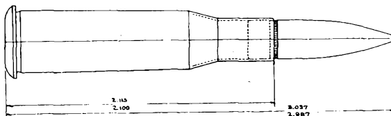
FIG. 161.—Caliber 7.62-mm. cartridge for Russian rifle.
