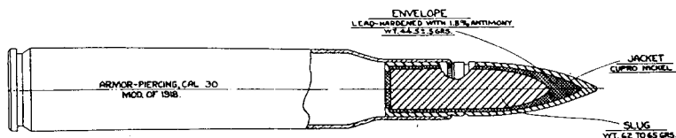
FIG. 157.—Armor-piercing cartridge, caliber .30, model 1918.
