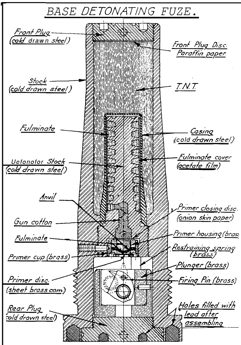
FIG. 65.—Base detonating fuze medium caliber (Model 1906).
