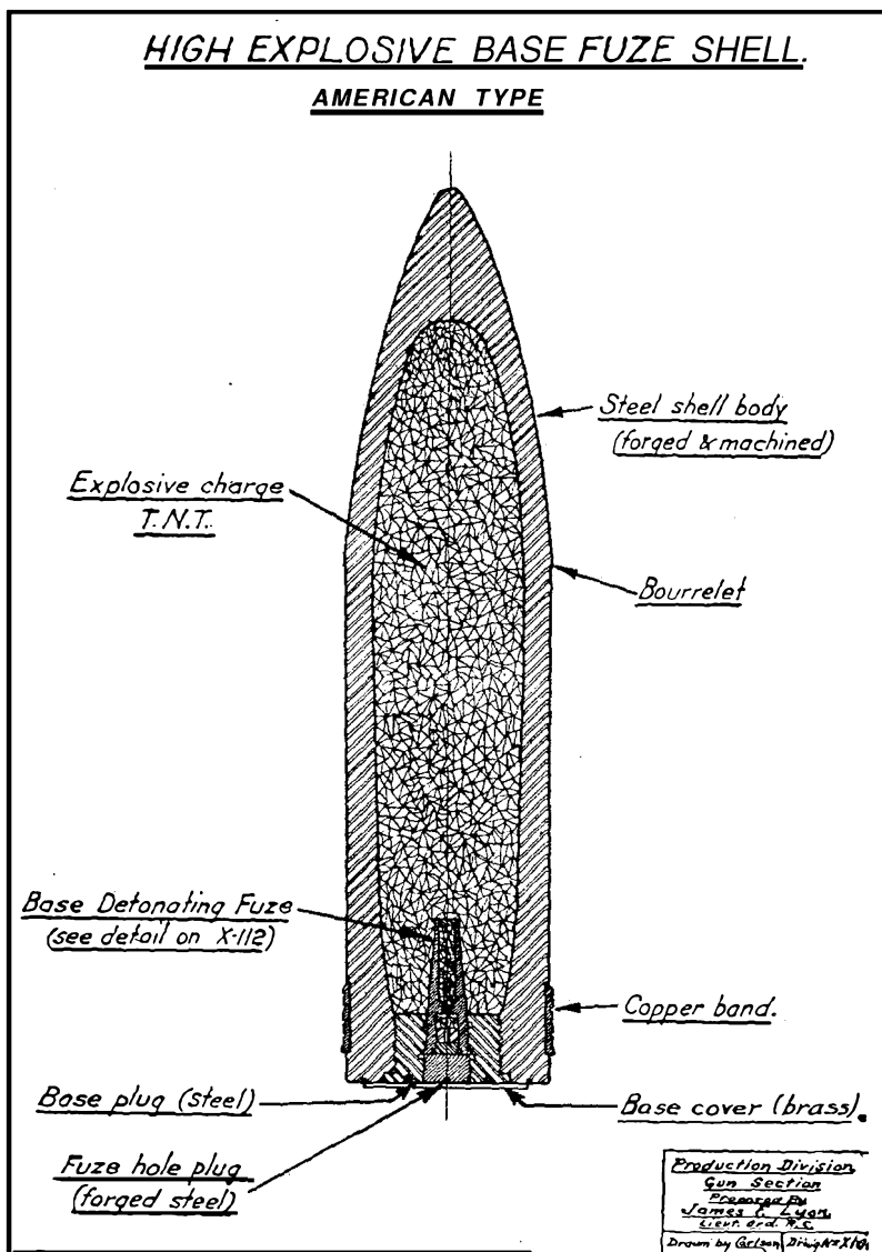
FIG. 50.—High-explosive base fuze shell, American type.
