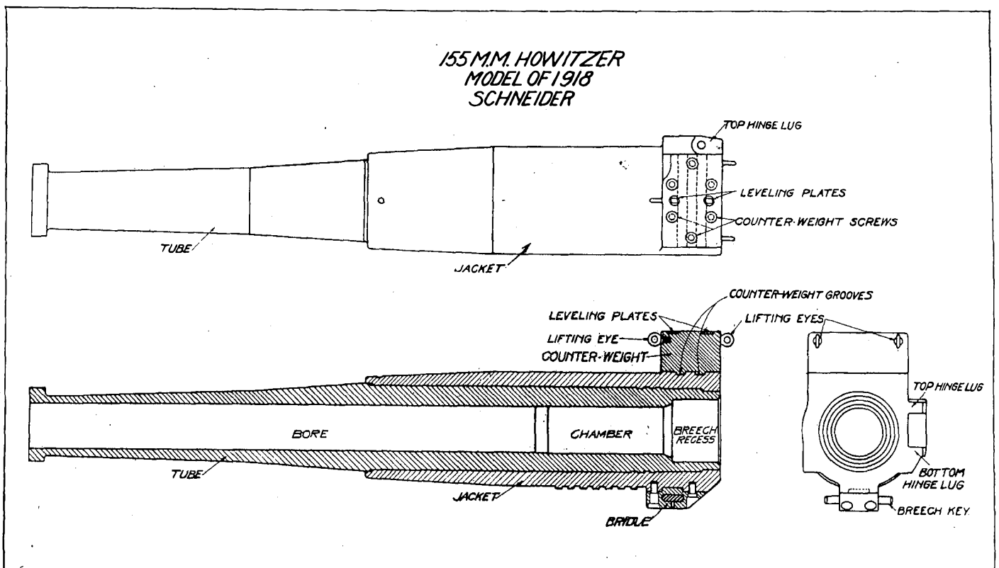
FIG. 20.—155-mm. howitzer, model of 1918 (Schneider).
