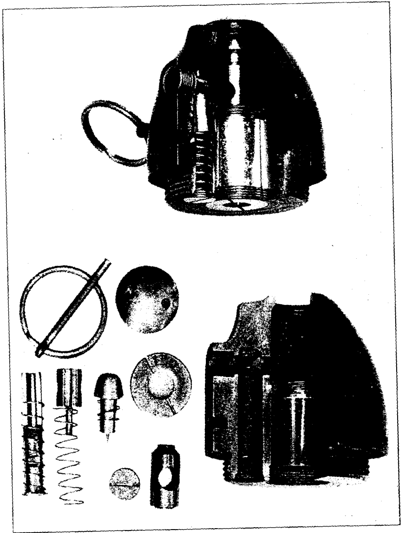
FIG. 105.—Trench mortar fuze, Mark VI. Assembly and section.
