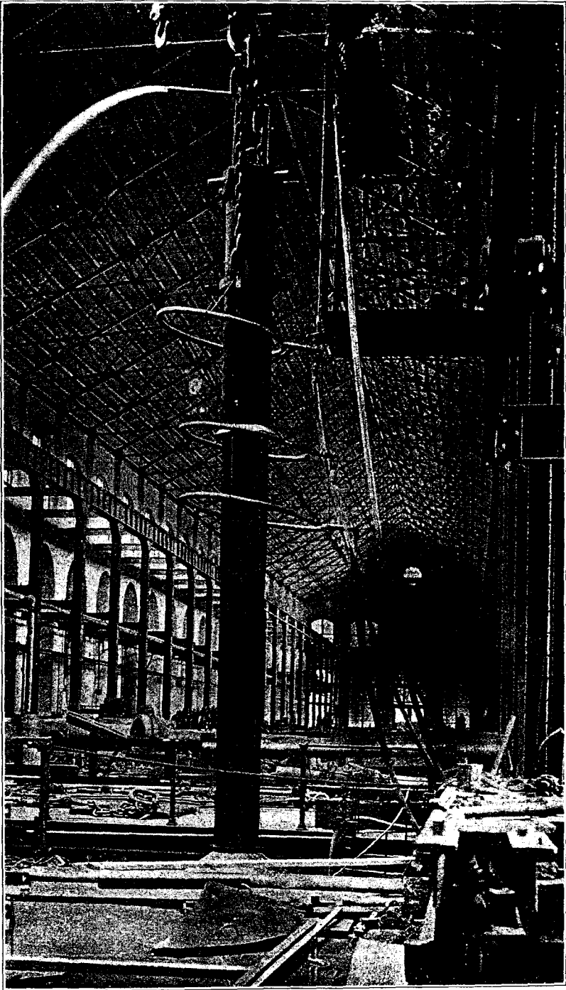
FIG. 5.—Equipment for cooling tubes at shrink pit, Watervliet Arsenal. Shrinking of 14-inch wire-wound gun.
