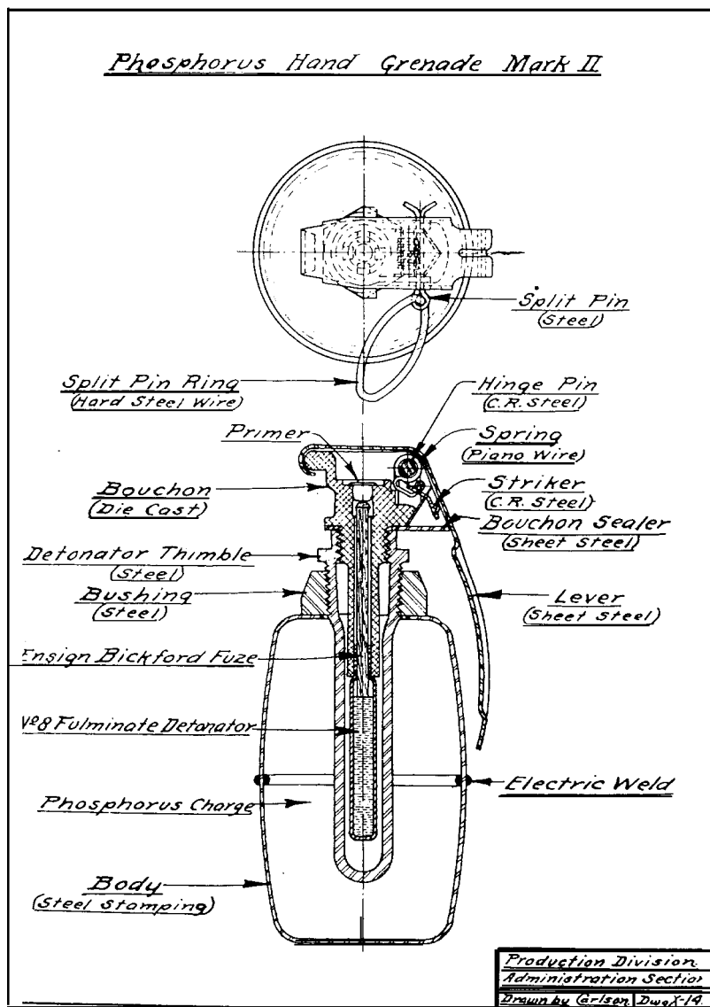
FIG. 88.—Sectional view of phosphorus hand grenade, Mark II.
