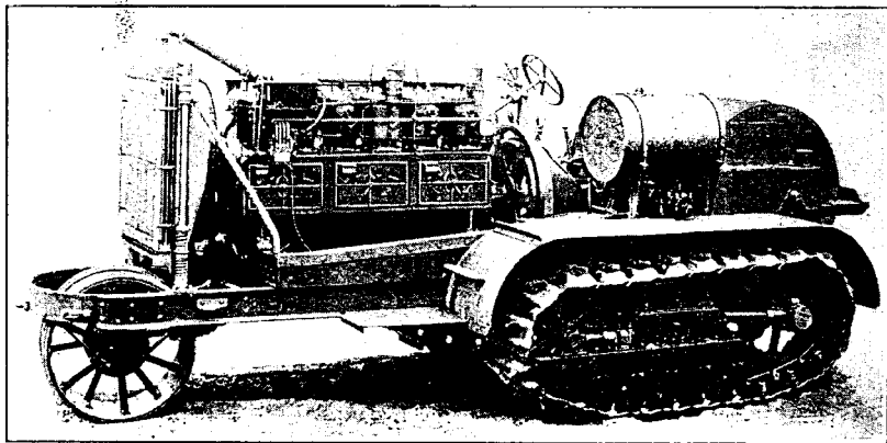
FIG. 181.—20-ton artillery tractor.
