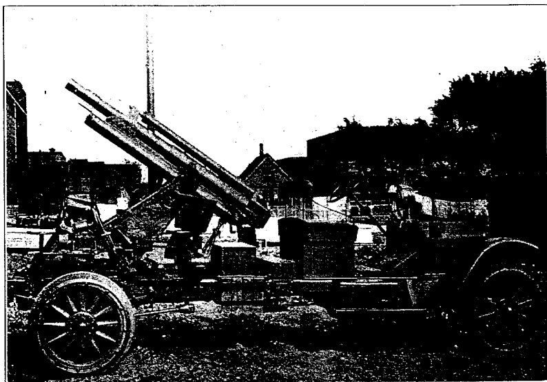
FIG. 40.—75-mm. field gun, model 1916, on A. A. truck mount, model 1917, 2½-ton White truck.
