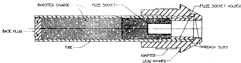
FIG. 71. Adapter and booster casing, Mark II.
