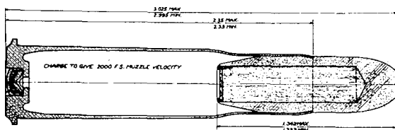
FIG. 163.—Incendiary cartridge, caliber 11-mm.
