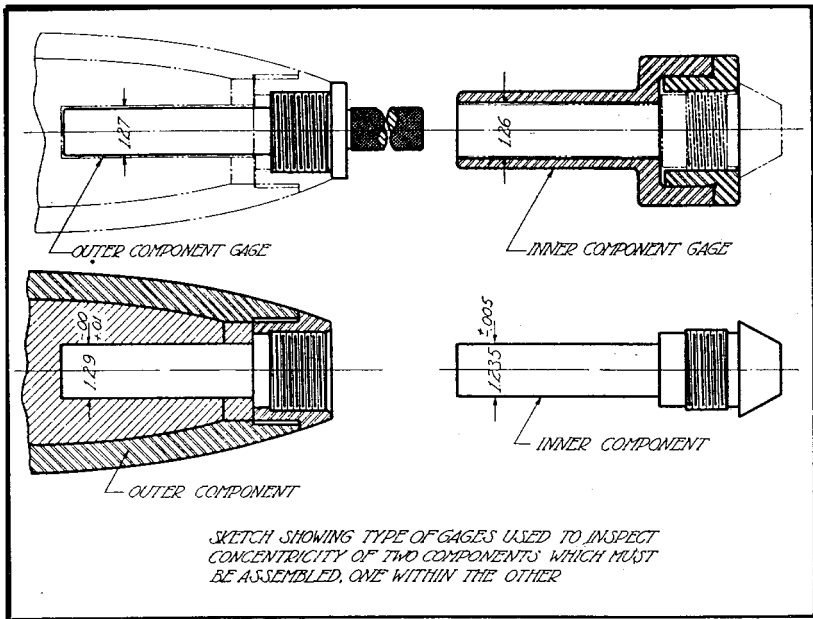
FIG. 223.—Concentricity gauges.
