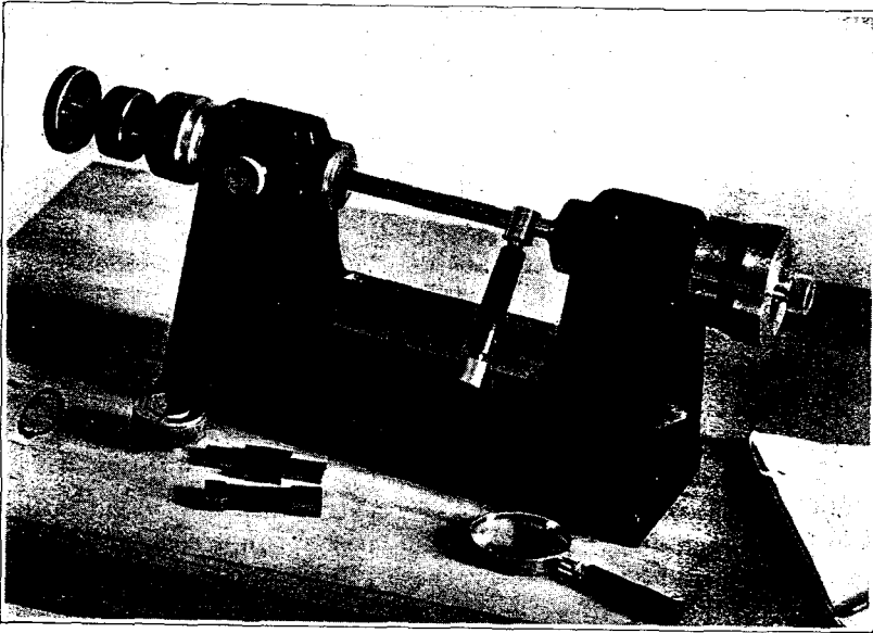
FIG. 221.—Micrometer for testing diameter of plug gauges.
