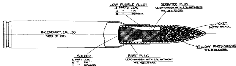
FIG. 158.—Incendiary cartridge, caliber .30, model 1918.
