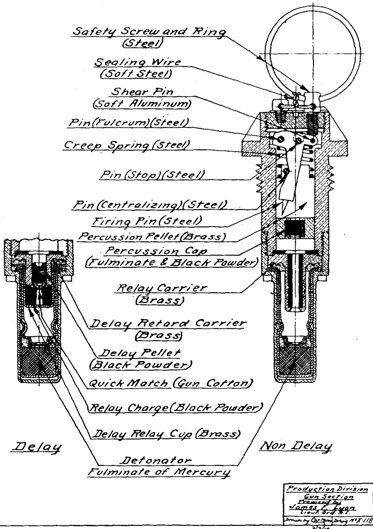
FIG. 105.—Detail of trench mortar fuze, Mark VII.
