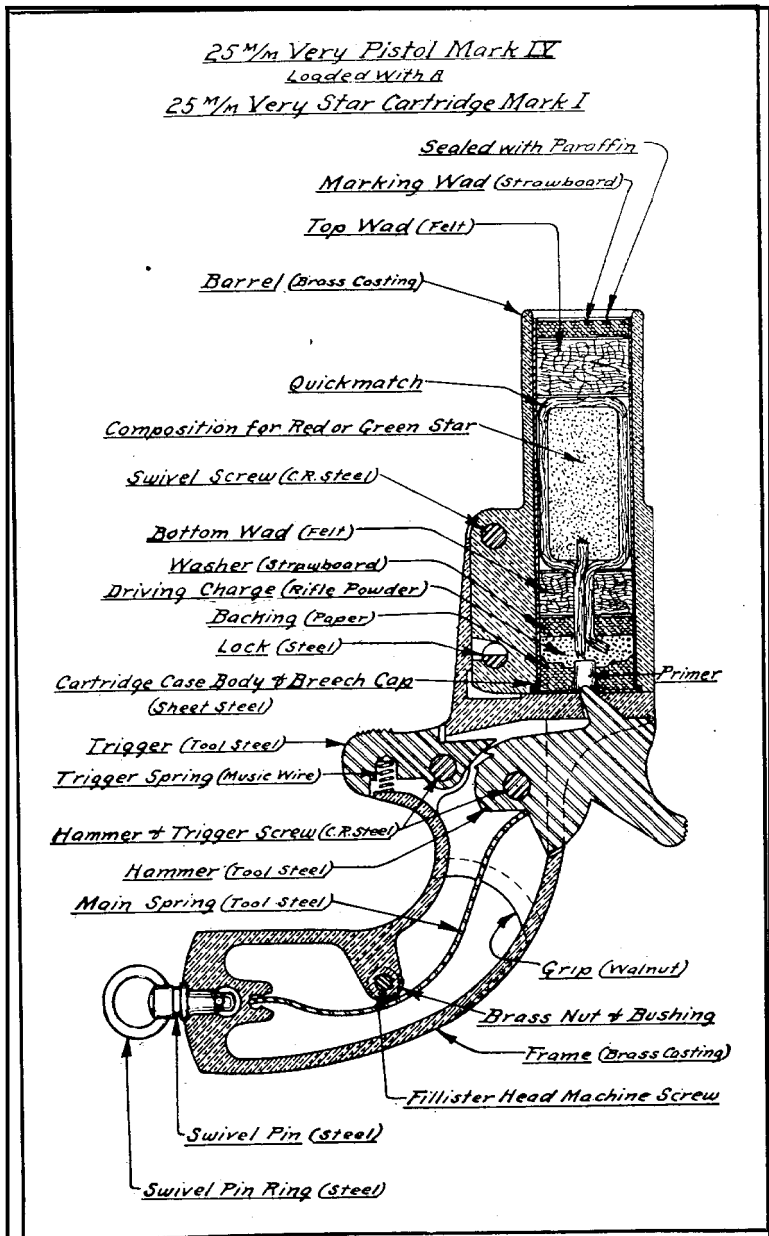
FIG. 128.—Very pistol, Mark IV, loaded with Very star cartridge, Mark I.
