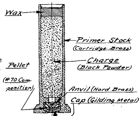
FIG. 75.—21-grain percussion primer.
