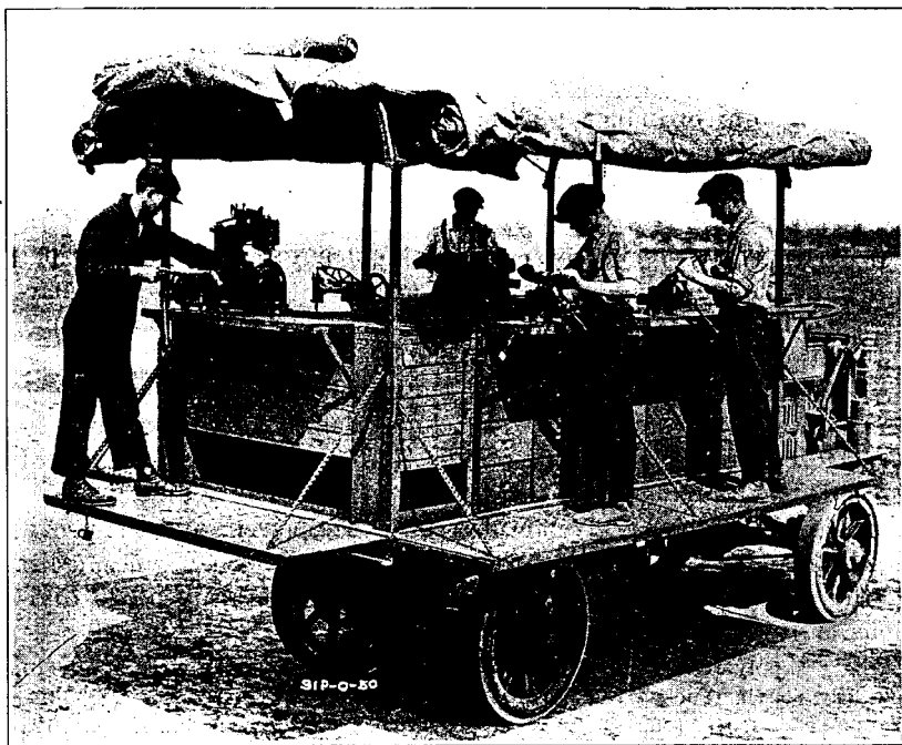
FIG. 170.—Equipment repair truck for making minor repairs of small arms, machine guns, harness, and personal equipment.
