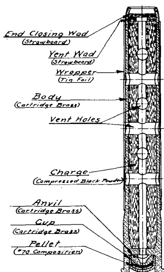
FIG. 74.—110-grain percussion primer.
