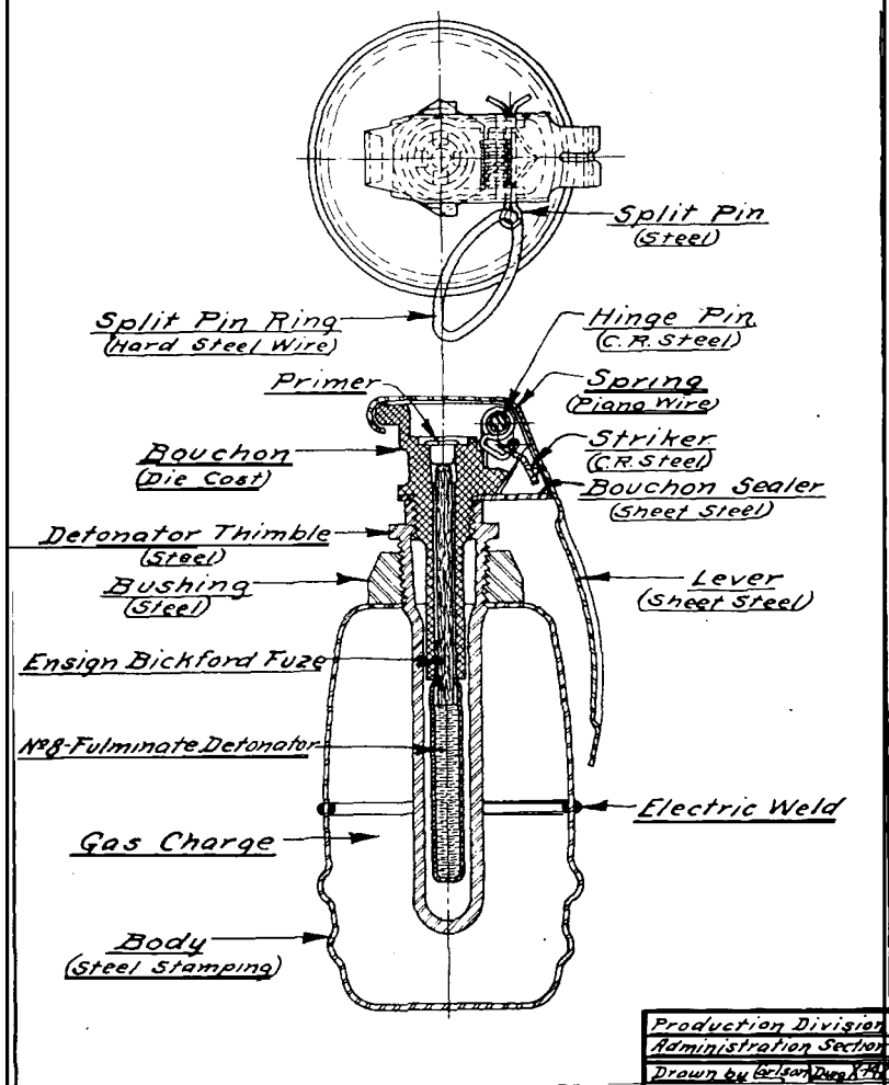
FIG. 89.—Sectional view of gas hand grenade, Mark II.
