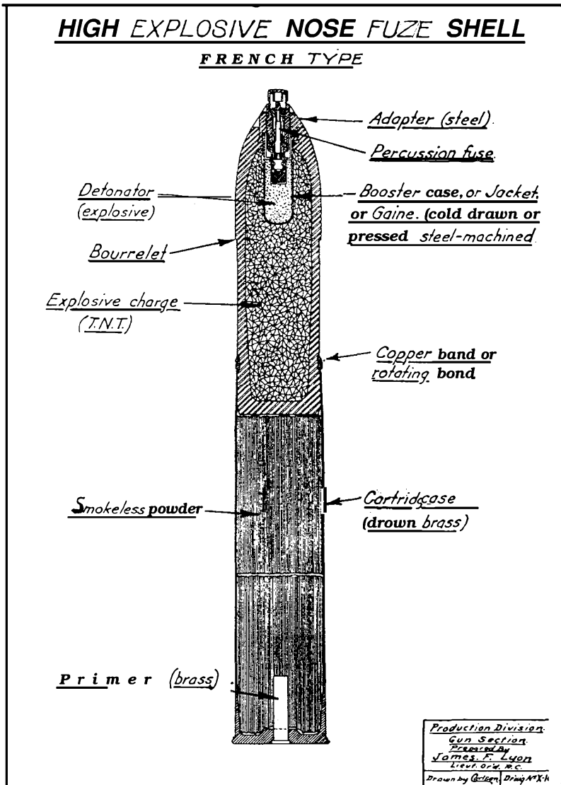
FIG. 52.—High-explosive nose fuze shell, French type.
