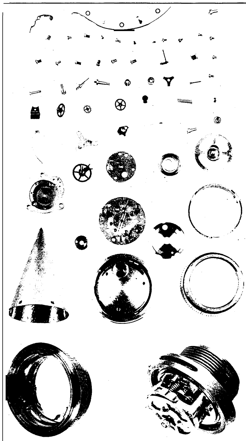
FIG. 70.—Mechanical time fuze, Mark I. Component parts.
