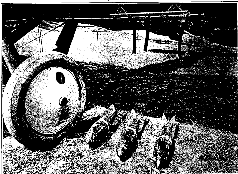
FIG. 125.—Mark III high-explosive bombs and Mark V release mechanism on D. H. 4 airplane.
