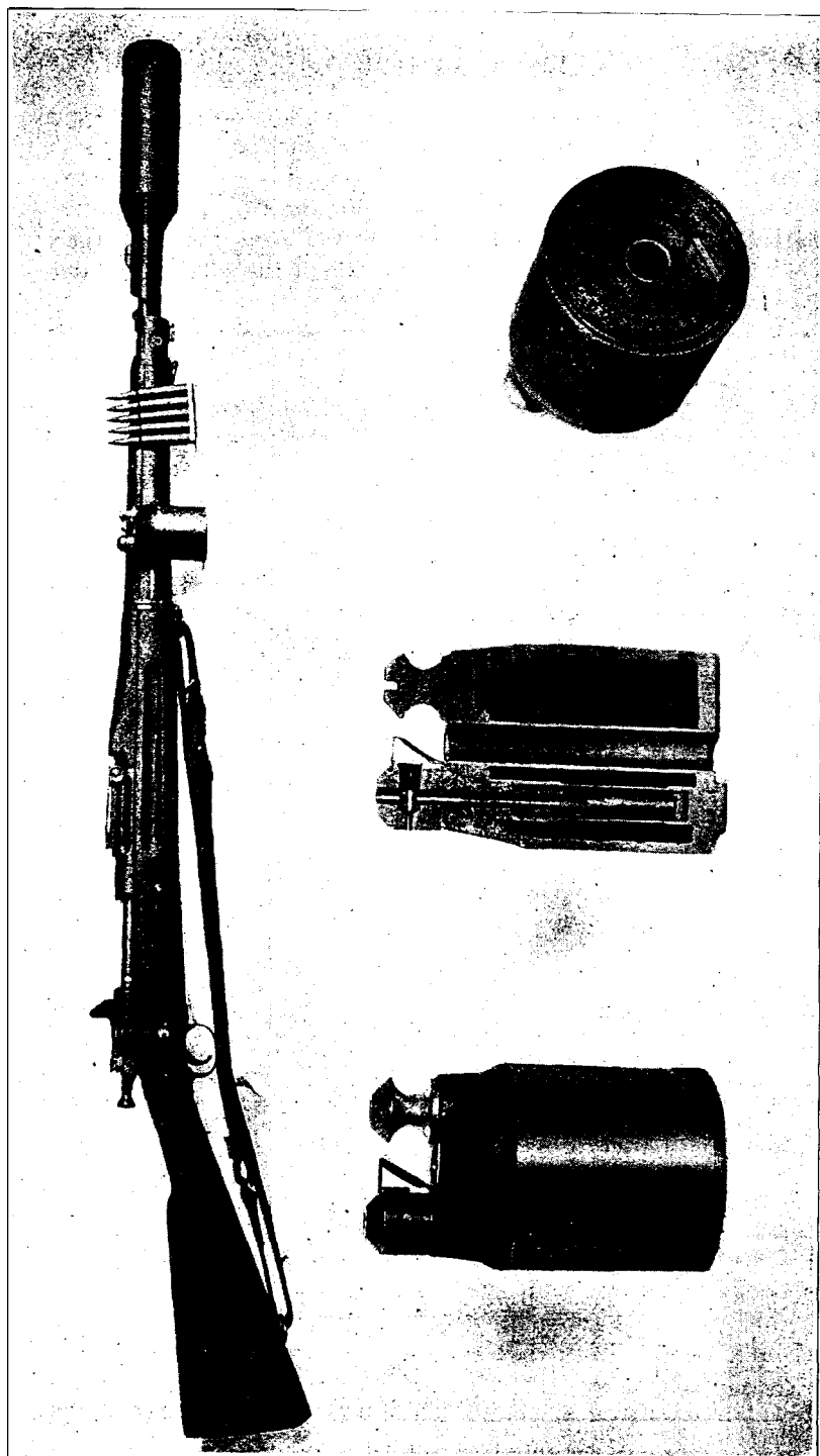
FIG. 93.—V. B. rifle grenade. Discharger mounted on rifle, together with grenade and cartridges. Side view of grenade. Sectional view of grenade. End view of grenade.
