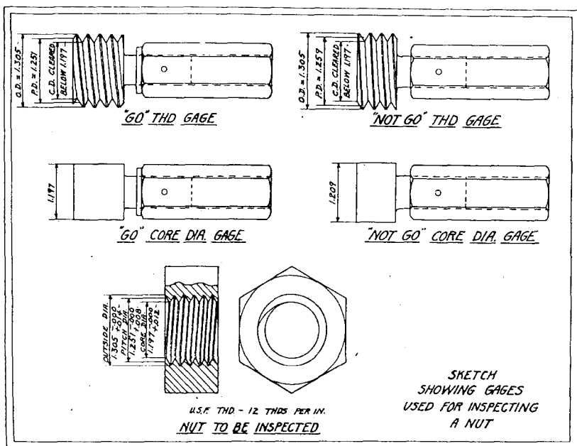
FIG. 217.—Gauges used for inspecting a nut.
