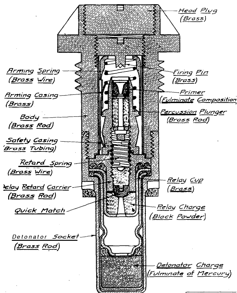
FIG. 60.—Point detonating fuze, Mark IV
