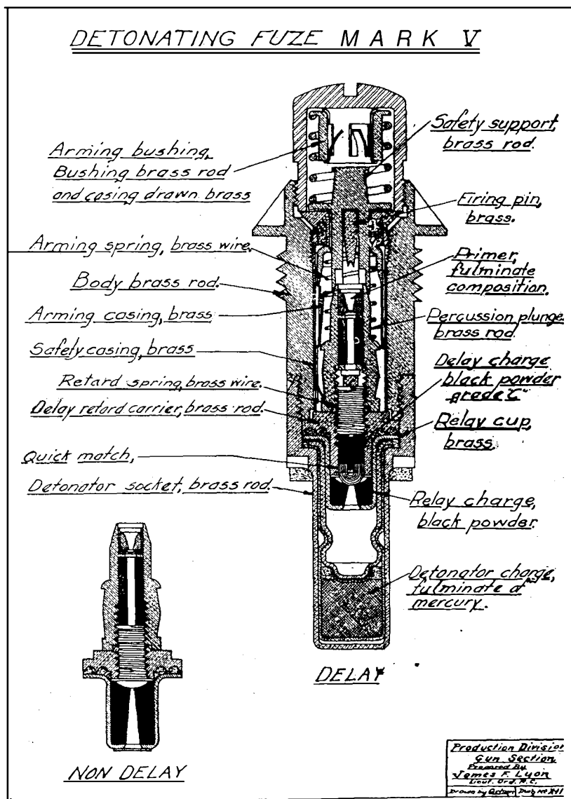
FIG. 61.—Point detonating fuze, Mark V.
