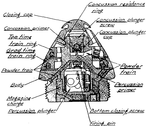
FIG. 68.—Combination time and percussion fuze—after arming.
