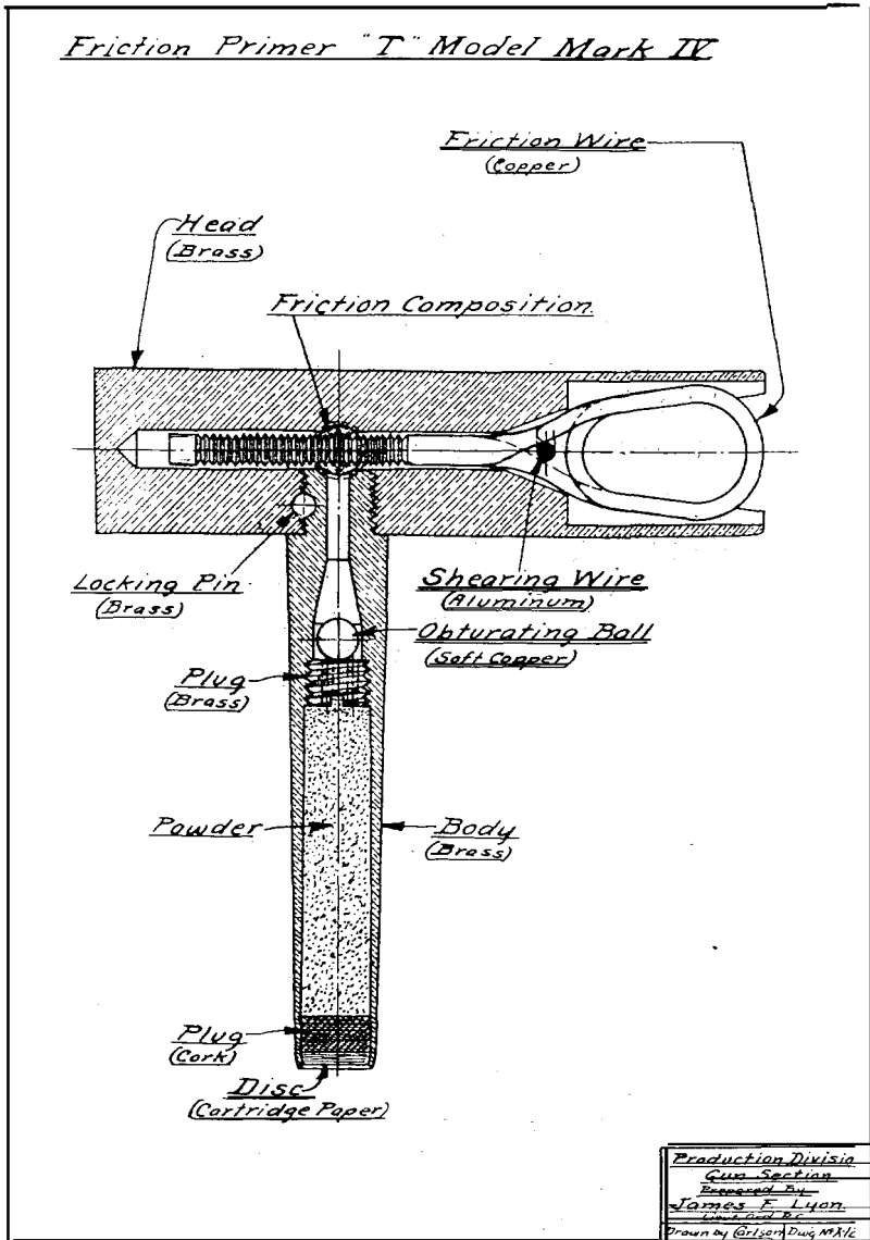
FIG. 78.—"T" model friction primer, Mark IV.
