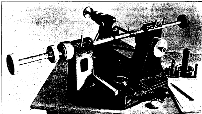
FIG. 226.—Apparatus for testing pitch diameter of screw thread gauges.
