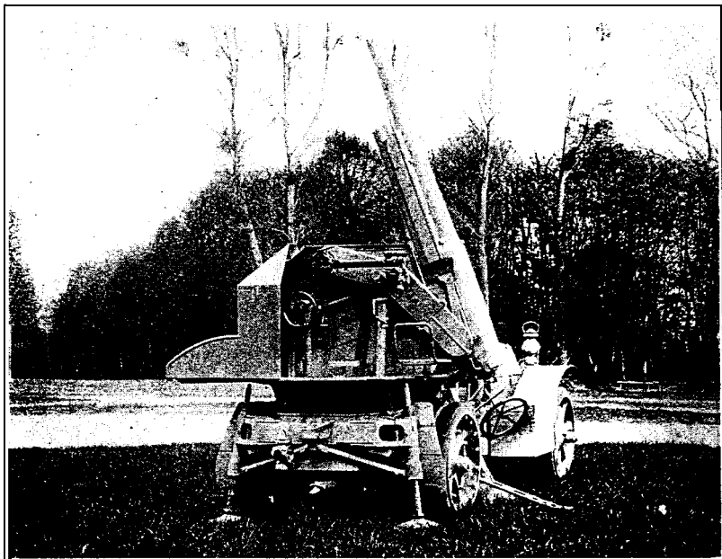
FIG. 44.—French 75-mm. A. A. gun on auto truck carriage.
