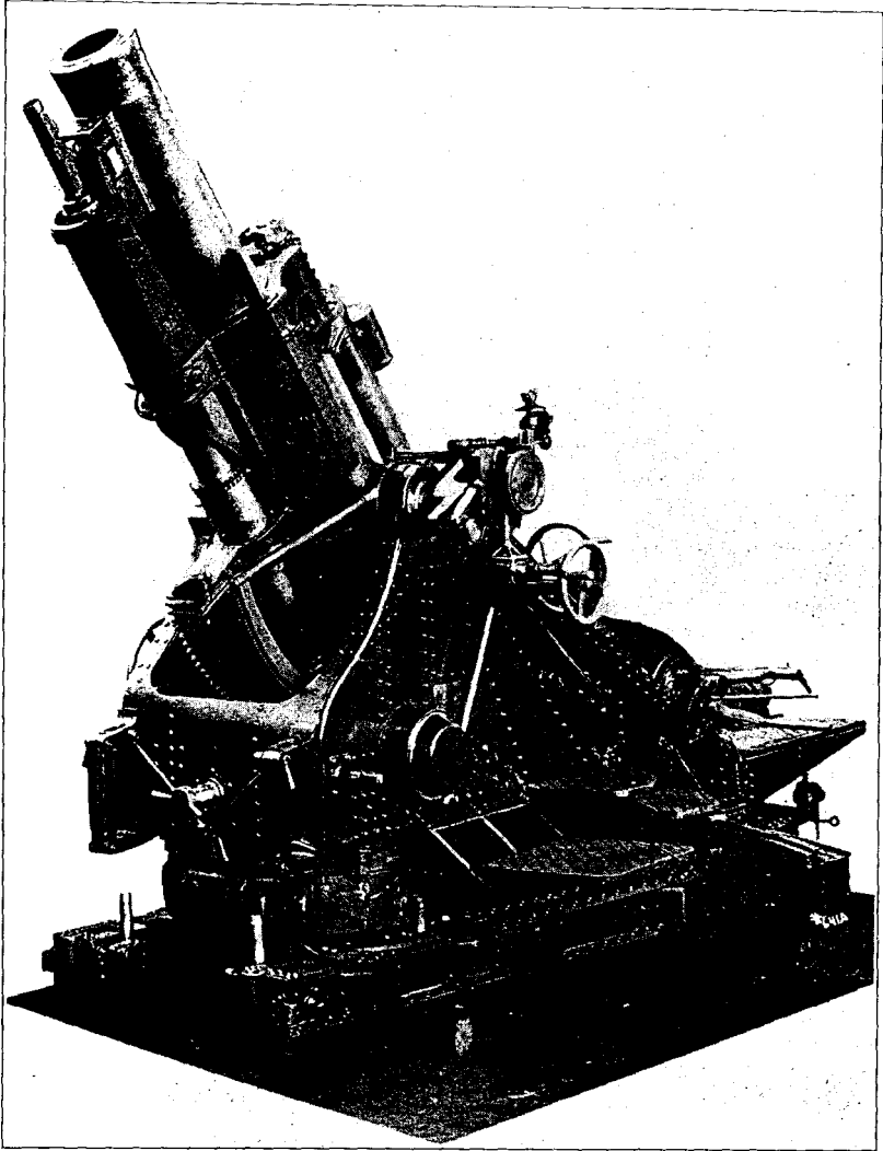
FIG. 23.—Vickers 9.2-inch howitzer, Mark I.
