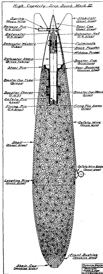
FIG. 115.—High-capacity drop bomb. Mark III.
