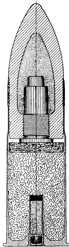
FIG. 76.—37-mm. ammunition with 20-grain primer.
