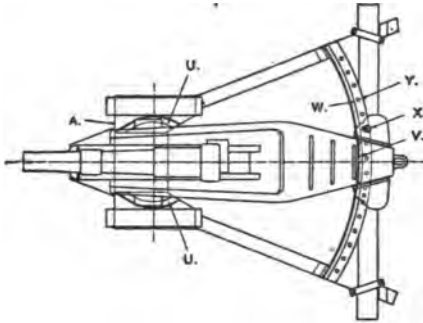
PLAN SHOWING CARRIAGE IN CENTRAL POSITION ON FIRING PLATFORM.
