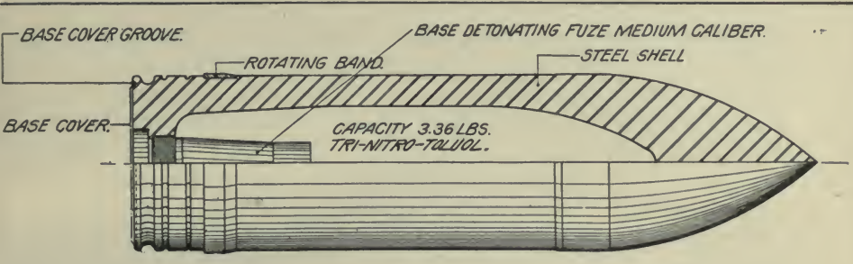
COMMON STEEL SHELL MODEL OF 1905.
