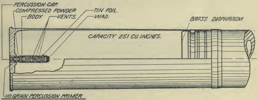
CARTRIDGE CASE.
