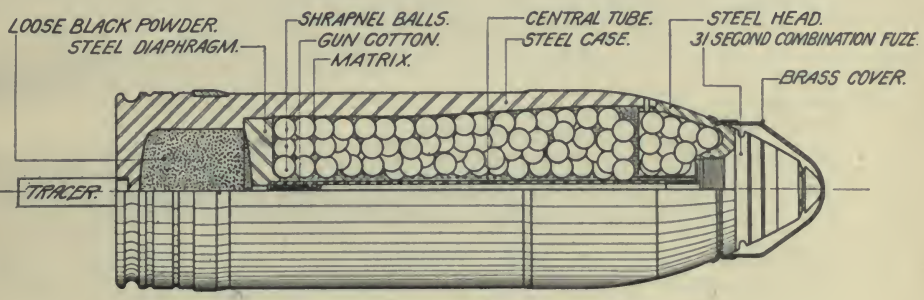
SHRAPNEL.
