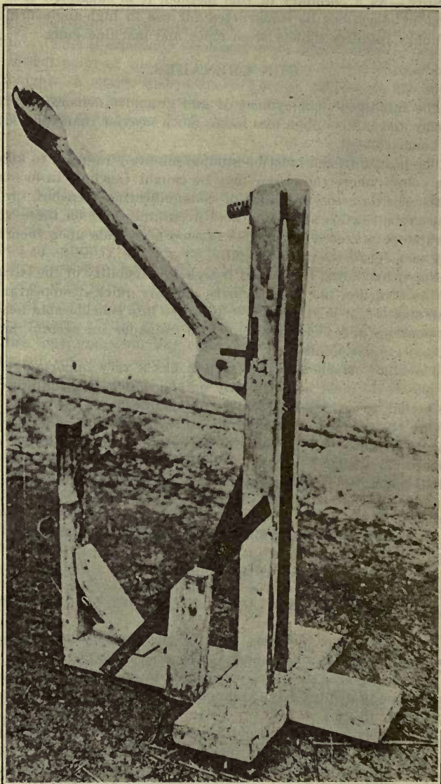
FIG. 15.—THIS DEVICE FOR CASTING GRENADES OR BOMBS IS OF VERY ANCIENT DESIGN, BUT IS BEING USED EFFECTIVELY FOR DROPPING BOMBS ON HOSTILE TRENCHES IN THE EUROPEAN WAR.
