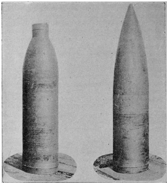
12-Inch Shell with Old Cap
