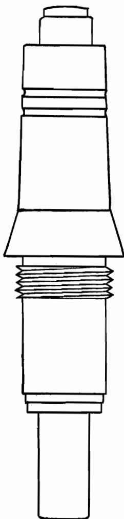
POINT DETONATING FUZE MARK XII FR. TYPE 24/31 R.Y.M. 1917. LENGTH 5.15"
