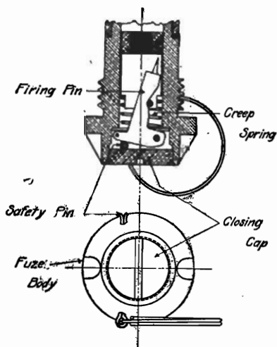
Firing Mechanism of Trench Mortar Fuze. Mark VII-E.
