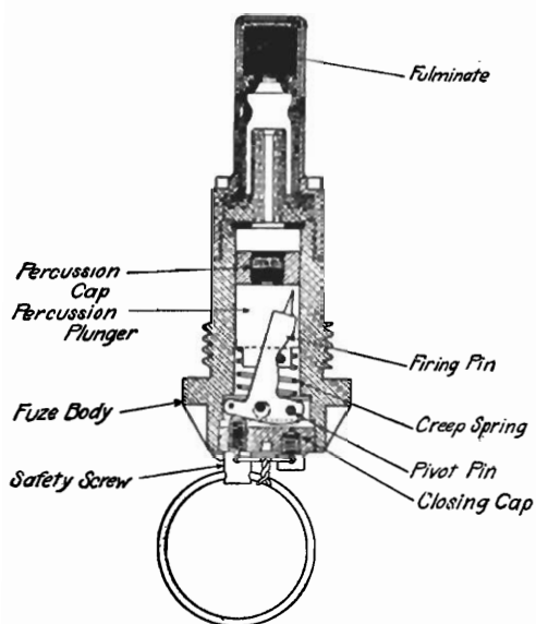
Trench Mortar Fuze, Mark VII, Nondelay.
