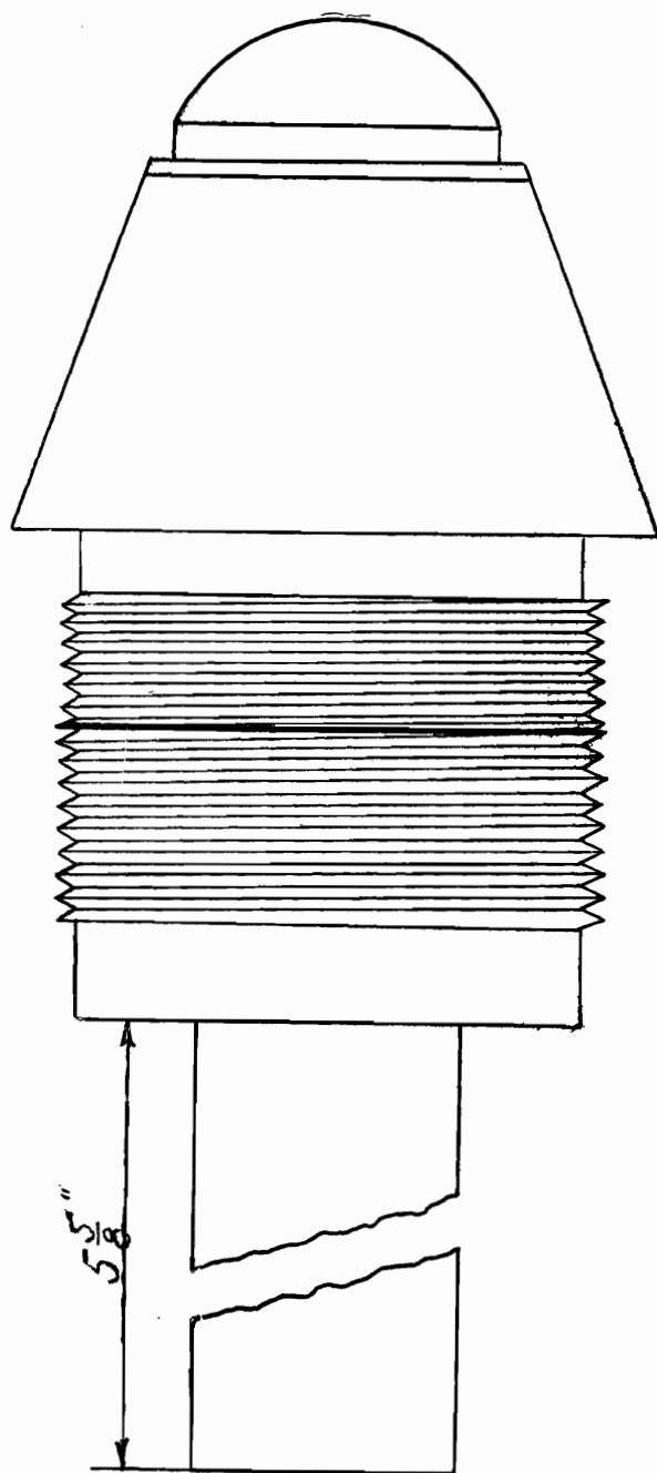
POINT DETONATING FUZE MARK IX & BOOSTER & ADAPTER MARK IX.
