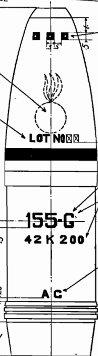
DIAGRAM FOR PAINTING AND MARKING FILLED SHELLS FOR PAINT SPECIFICATIONS SEE ORDINANCE PAMPHLET 1868A
