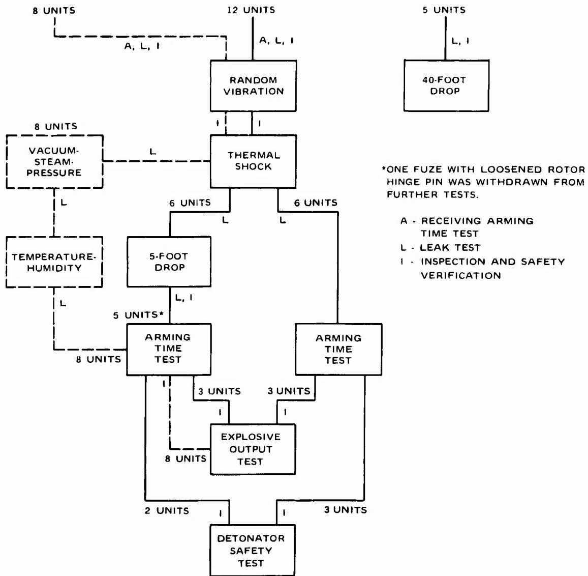
FIG. 4. Laboratory Evaluation Test Sequence of FMU-90/B Fuze.
