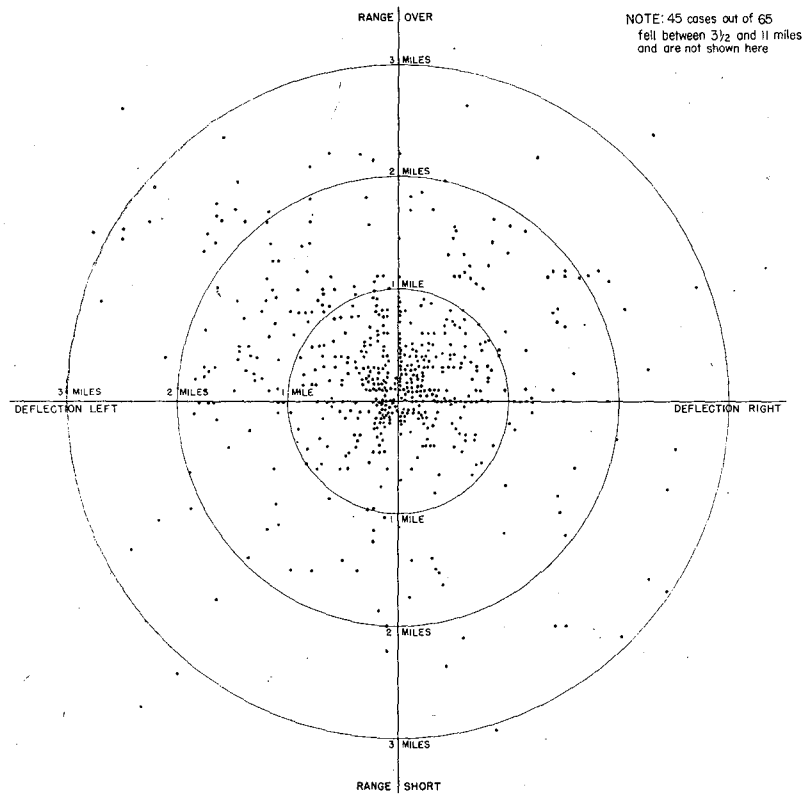
Fig. 8-Z1 Distribution of Circular Error in Radar Mine Laying
