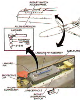
ANTISHIP VERSION BLAST-EFFECT WARHEAD
