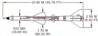
U.S.S.R. GUIDED MISSILE, SURFACE-TO-AIR, SA-2D (GUIDELINE)
