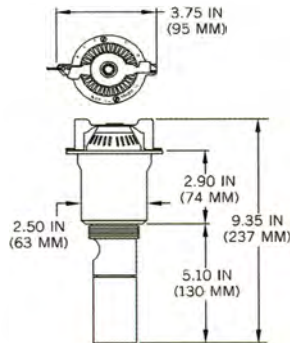
M904E1 (SHOWN)
