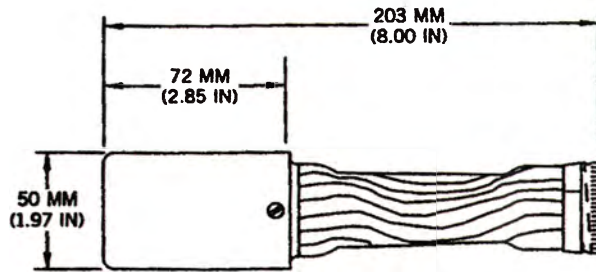
NONSERRATED SHORT CYLINDRICAL HEAD (A)
