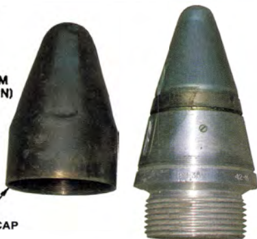
U.S.S.R. PROJECTILE FUZE, MT, VM-30
