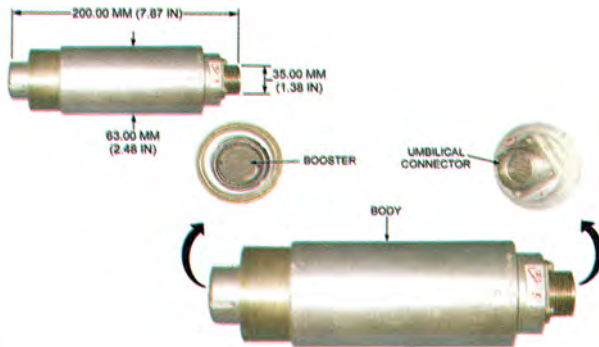
U.S.S.R. BOMB FUZE, TAIL, IMPACT/SELF DESTRUCT, AV-551
