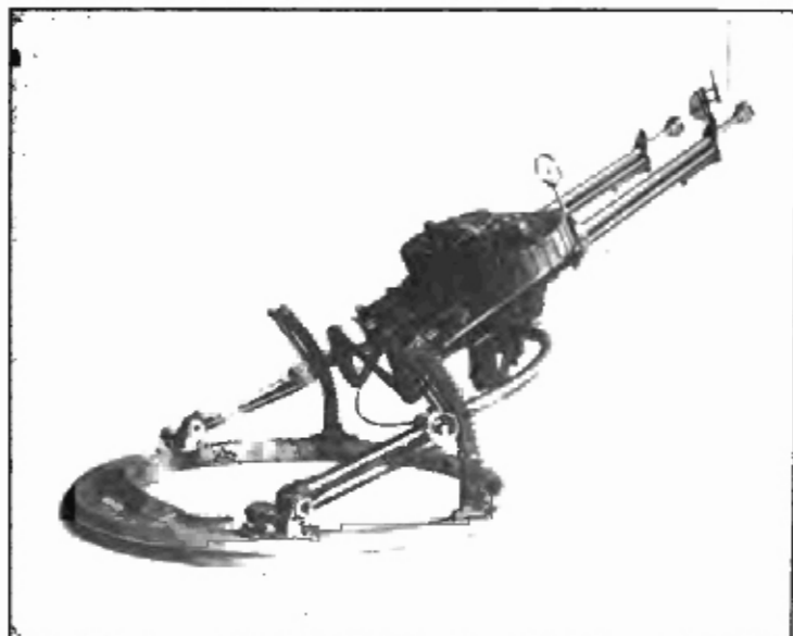
FIG. 27.—DOUBLE LEWIS GUN YOKE WITH GUNS.
