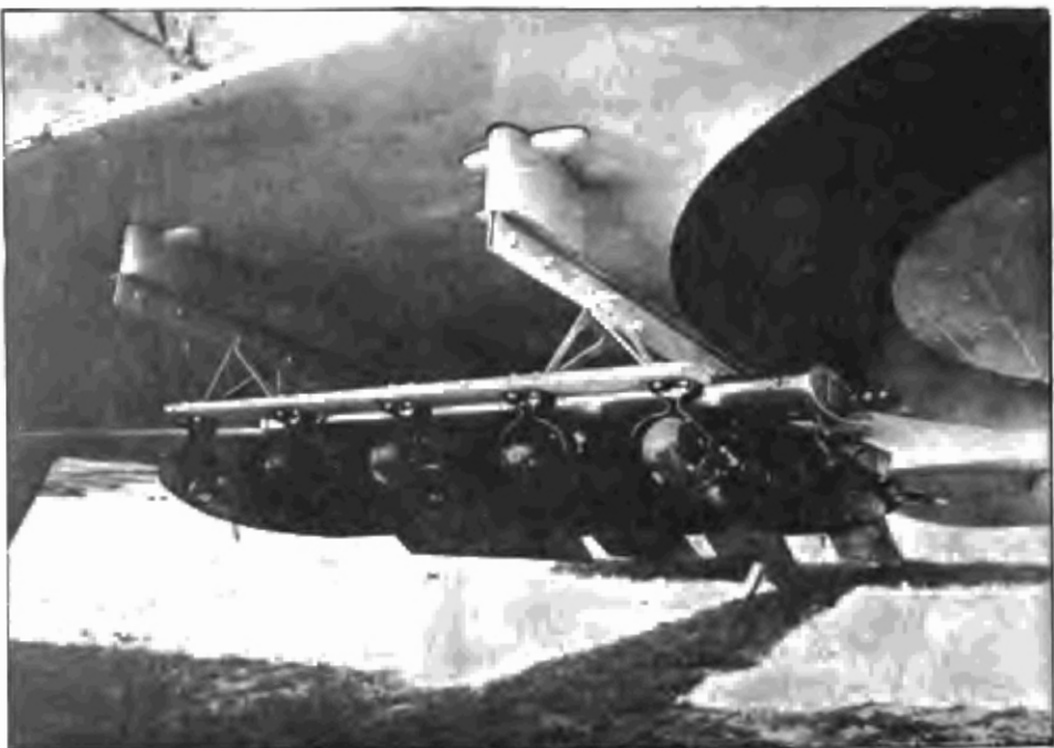
FIG. 45.—MARK V BOMB RELEASE MECHANISM ON DE HAVILLAND 4.
