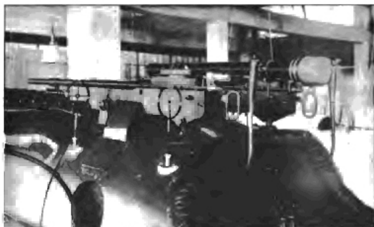
FIG. 22.—FIXED MOUNTS FOR TWO MARLIN AIRCRAFT MACHINE GUNS ON DE HAVILLAND 4.
