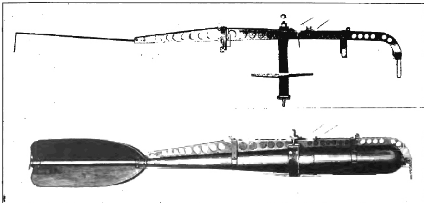
FIG. 43.—BARLOW HEAVY DROP BOMB AND RELEASE MECHANISM.
