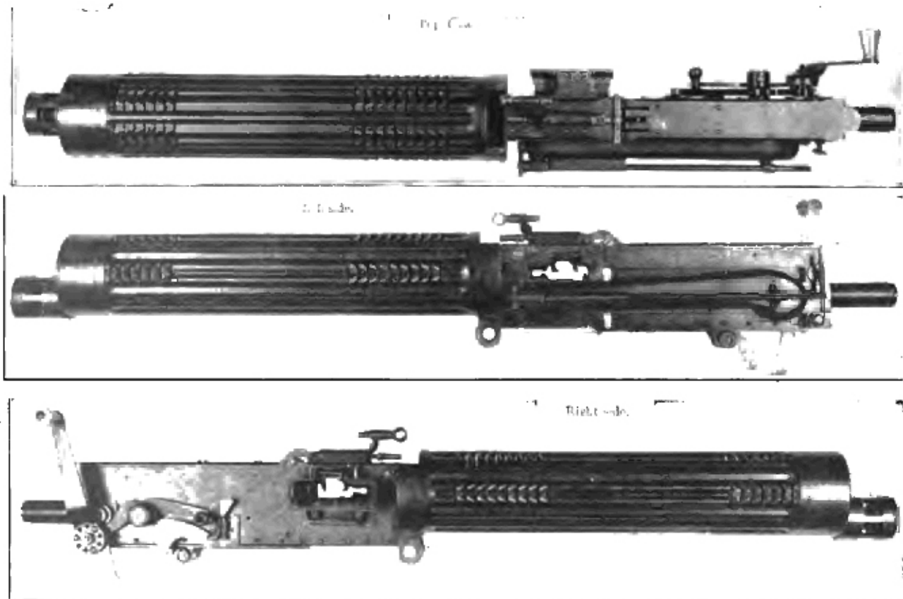
FIG. 17.—UNITED STATES VICKERS AIRCRAFT MACHINE GUN, CAL. .30, WITH LOADING HANDLE, SPEEDING-UP ATTACHMENTS, AND TRIGGER MOTOR FOR MECHANICAL SYNCHRONIZING GEAR, TYPE H-S.
