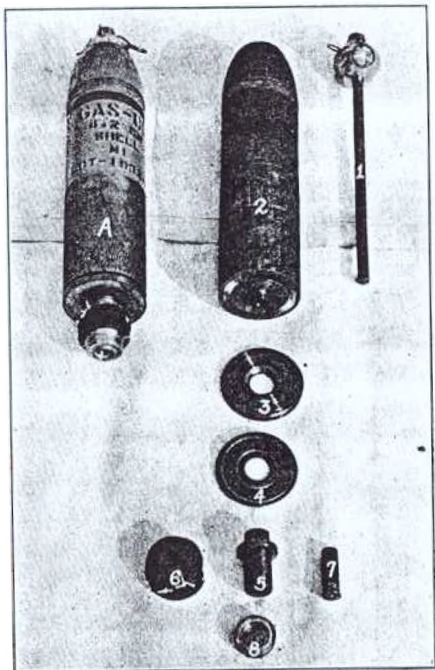
FIGURE 5.—4.2-inch chemical mortar shell
