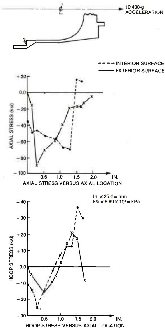
Figure 21. Combined stresses.
