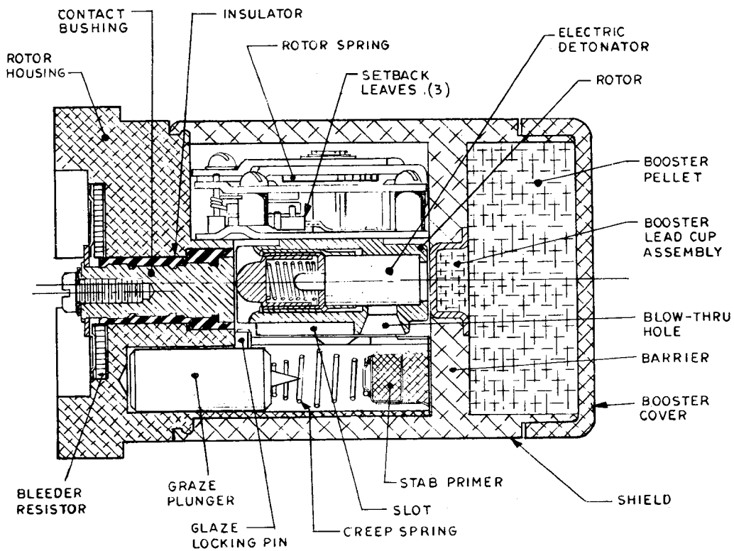
Figure 2. M530A1 fuze.
