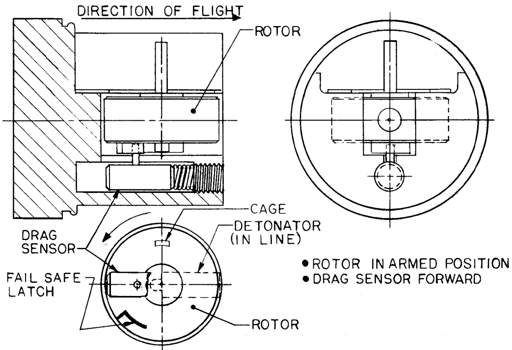
Figure 5. Condition on completion of arming.
