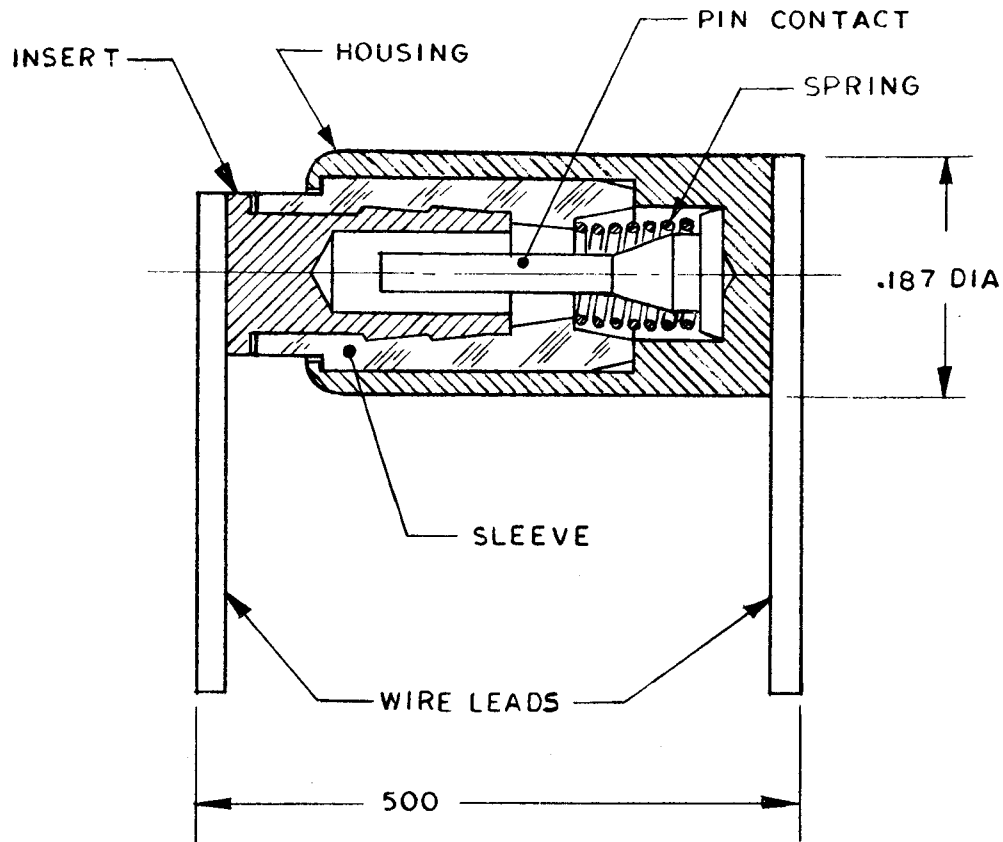
Figure 9. Inertial impact switch.
