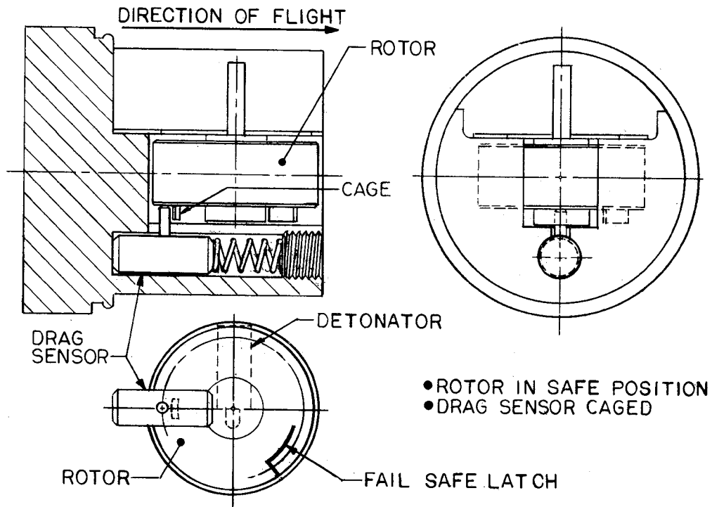
Figure 3. Condition prior to launch.
