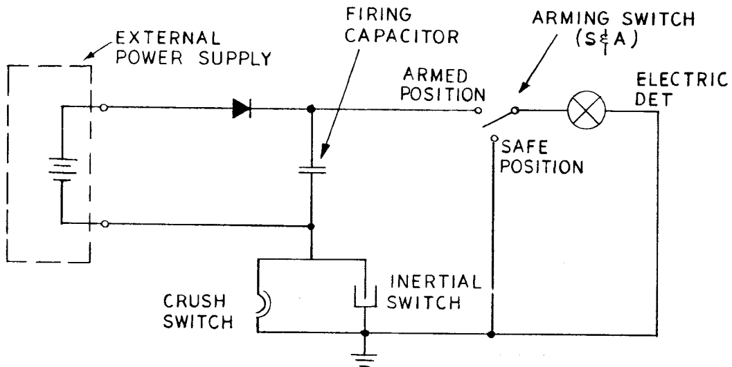
Figure 8. Basic firing circuit.
