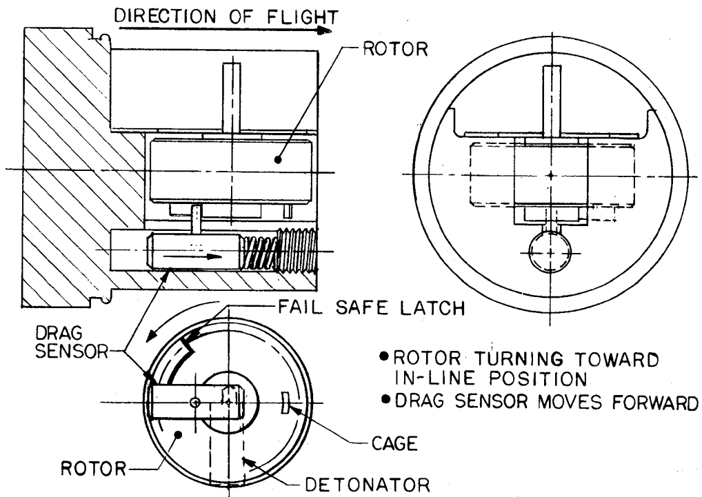
Figure 4. Condition following normal launch (drag exceeds 4 g).
