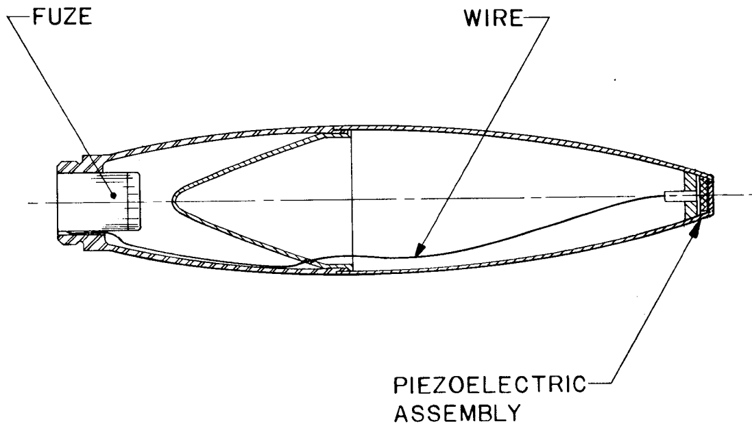
Figure 1. Conventional PIBD fuzing system.
