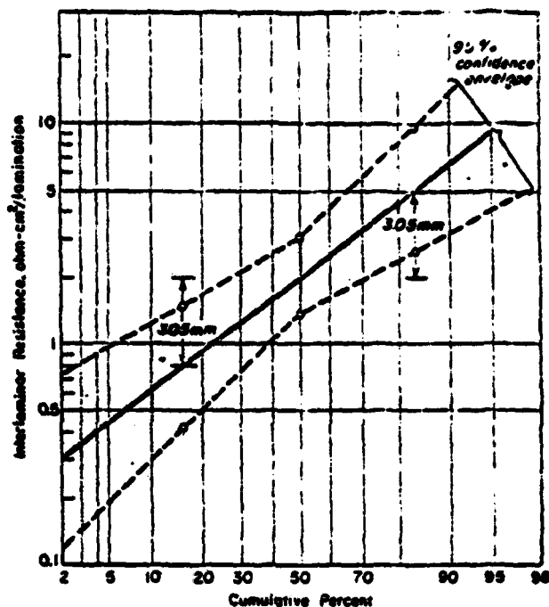
4—Confidence envelopes for logarithmic probability paper. Estimate of standard deviation ( s ) is made equivalent to distance between 50% ordinate and either 16% or 84% ordinate.
