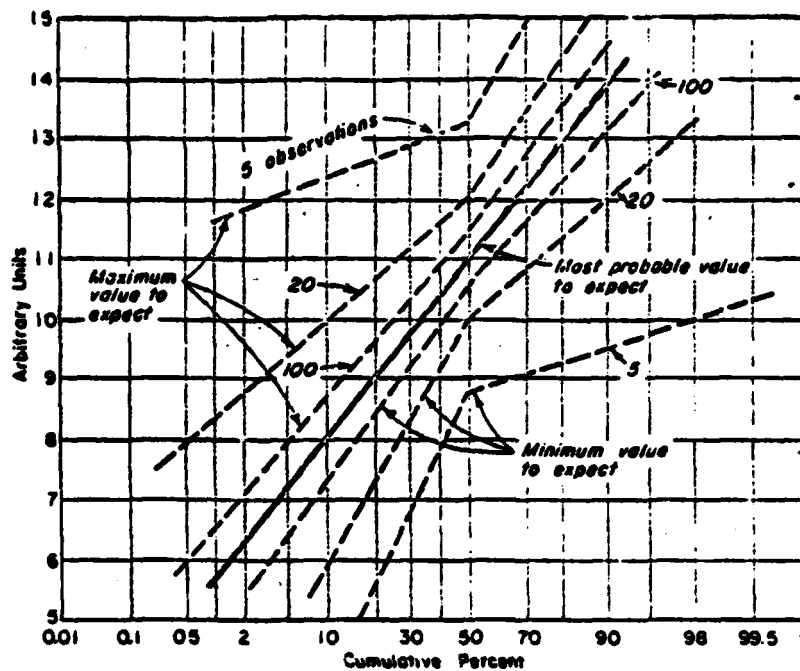
S —Reliability increases as the number of observations increases. A similar effect results when the confidence level is decreased.
