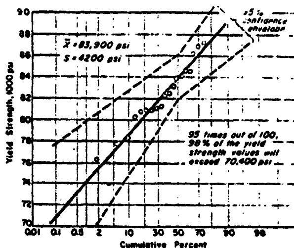
2—Distribution of yield strength forecast minimum expected values for use in setting specification limits.
