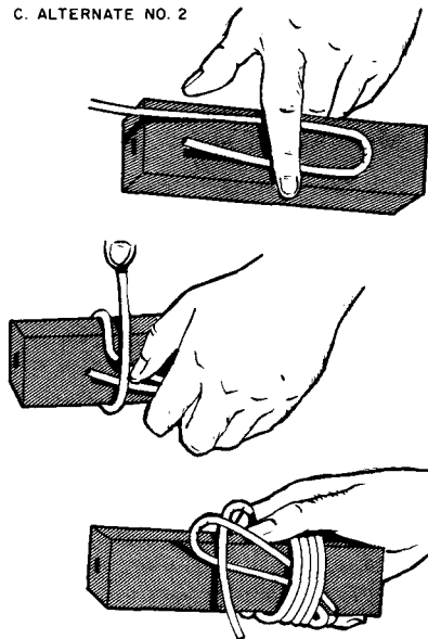
Figure 77. Detonating cord priming of demolition blocks.
