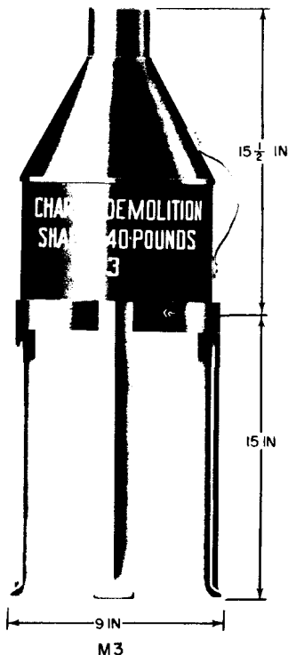
Figure 8. Shaped charges.
