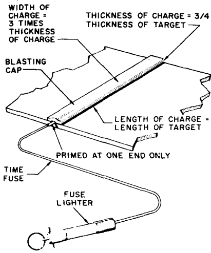
Figure 102. Ribbon charge.
