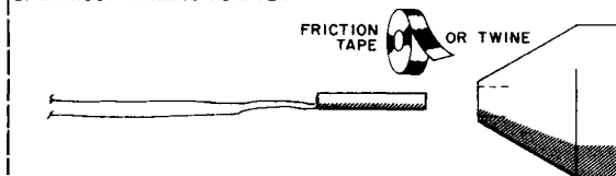
Figure 70. Electric priming of shaped charges.
