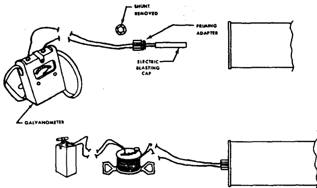
Figure 64. Electric priming of demolition block with priming adapter.
