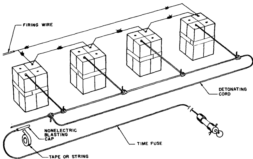
Figure 98. Combination dual firing system.
