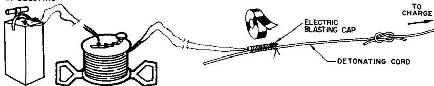
Figure 85. Electric and nonelectric assemblies attached to main line.
