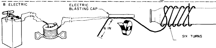
Figure 83. Detonating cord priming of bangalore torpedo.
