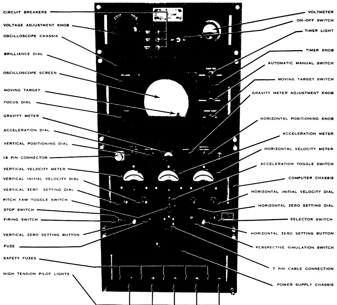
Figure 17. Simulator S-58.
