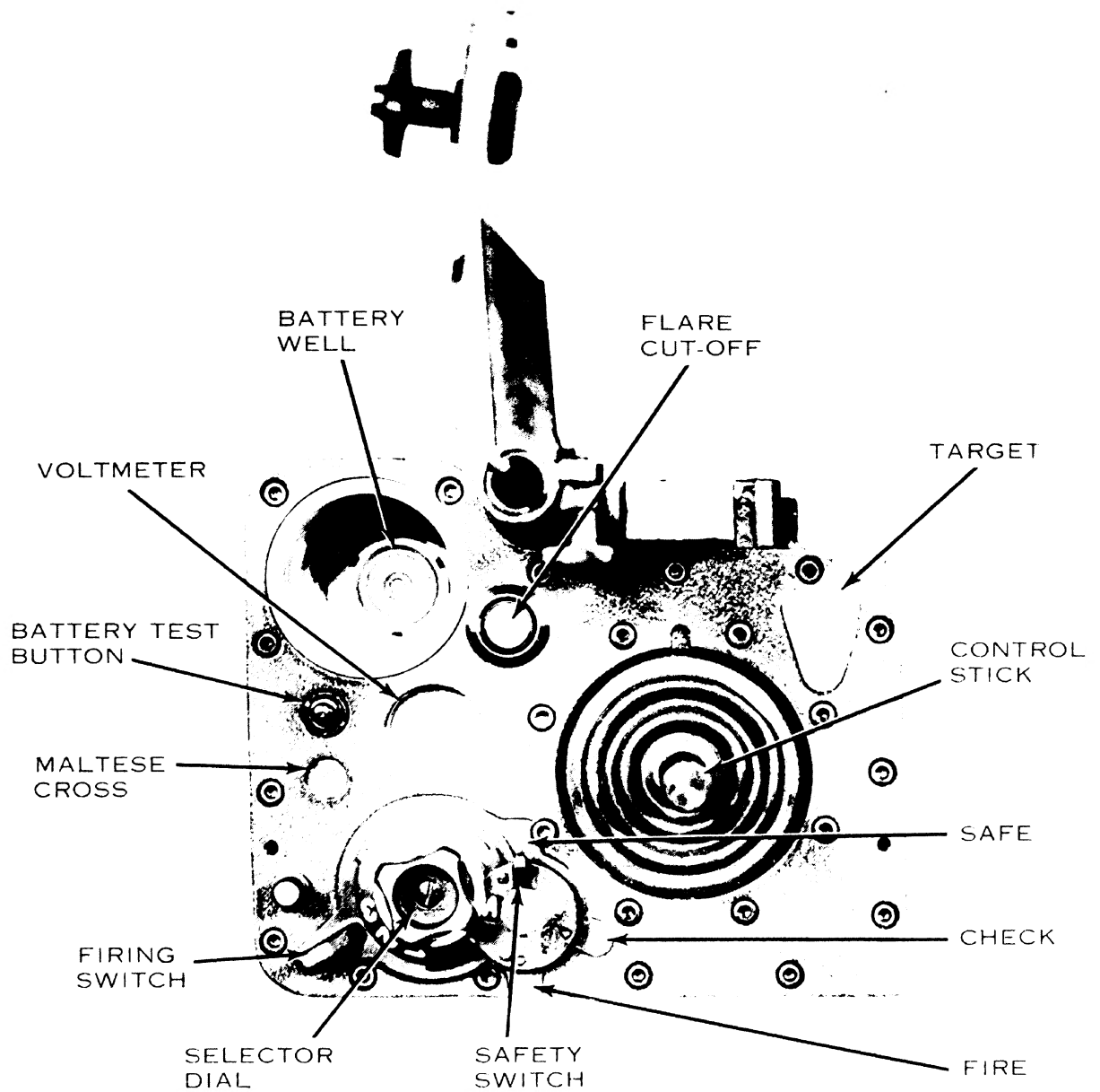
TOP VIEW (WITH BATTERY AND BINOCULARS REMOVED)
