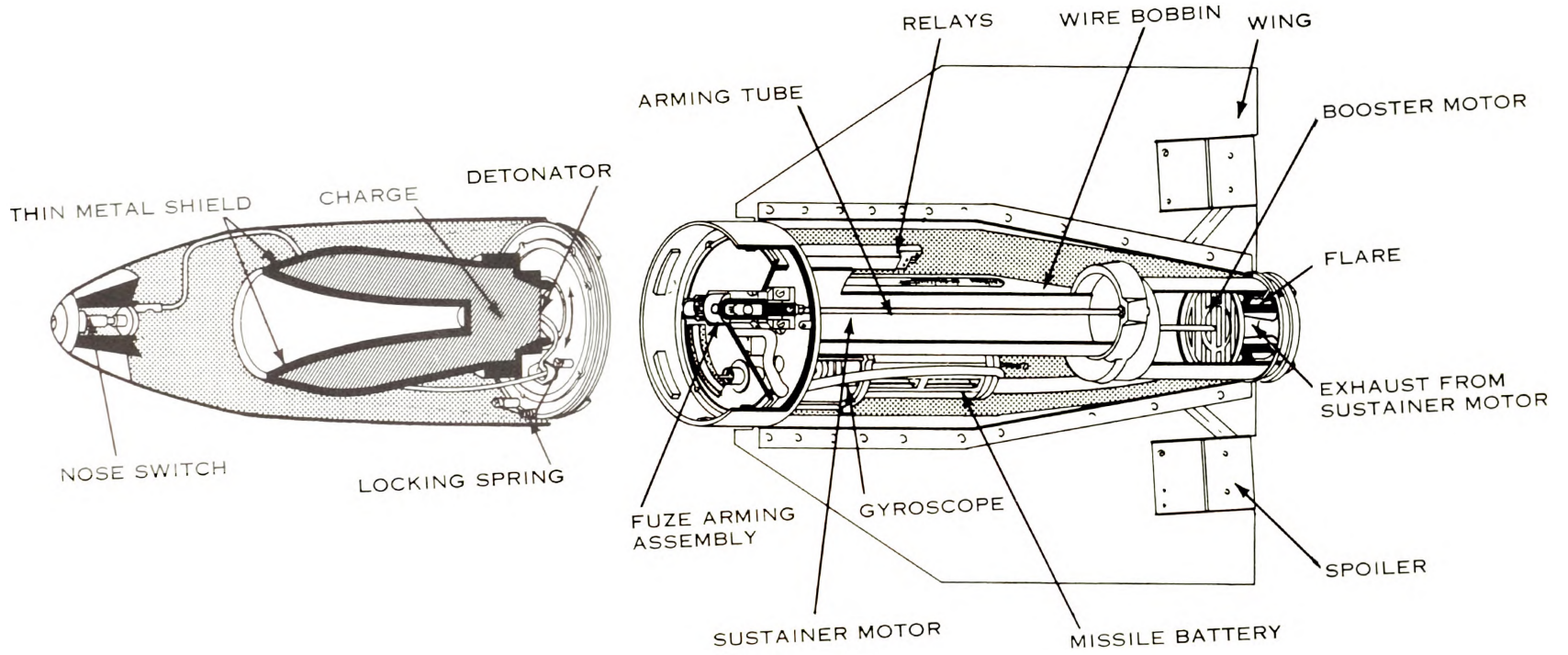
Figure 5. Cutaway drawing of the ENTAC.
