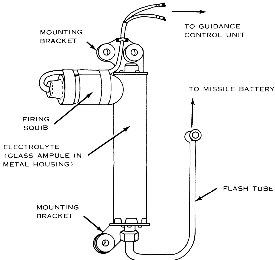
Figure 6. Battery activator.
