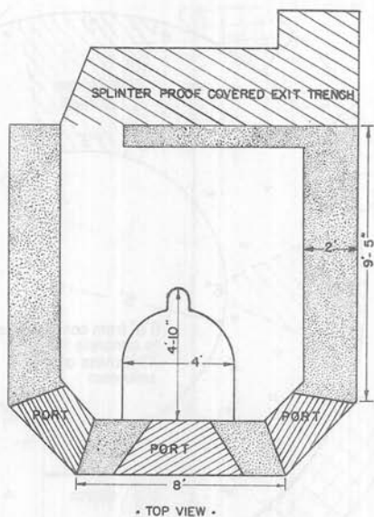
Sketch of Heavy Concrete Pillbox - Talisay Beach (See Photos Page 8)
