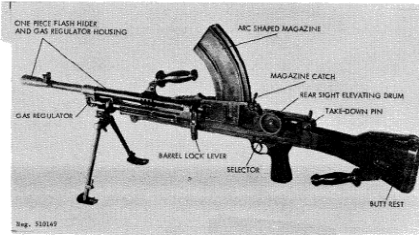
Figure 150. Mark 1 Bren.
