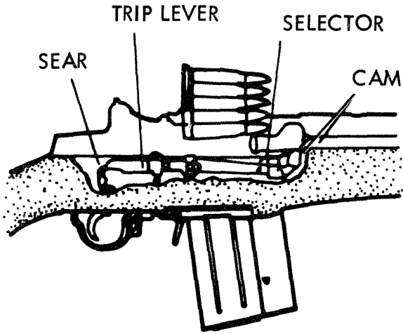
Figure 112. BM-59 Mechanism
