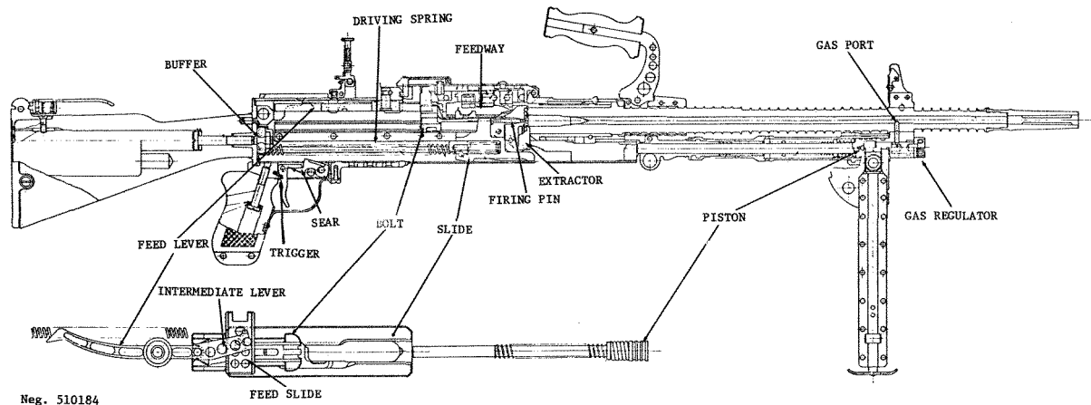
Figure 185. Type 62 section.
