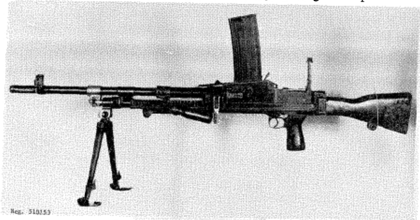
Figure 154. L4A1 Bren.
