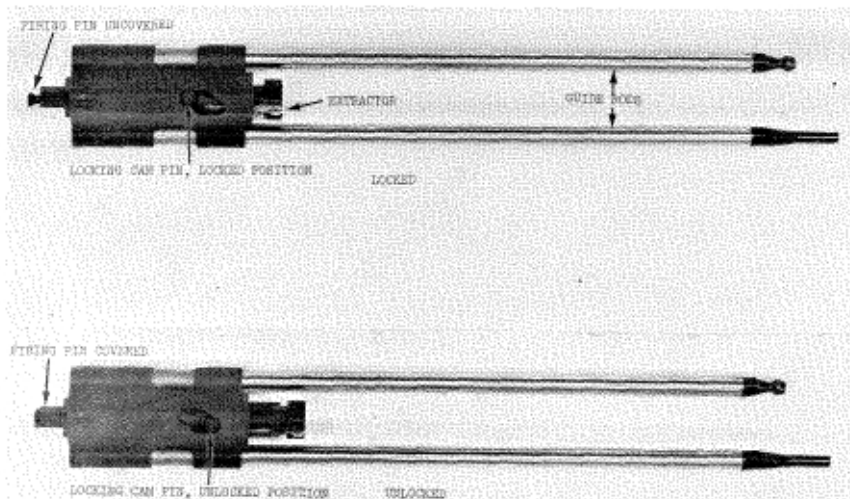
Figure 103.12. Bolt functioning.
