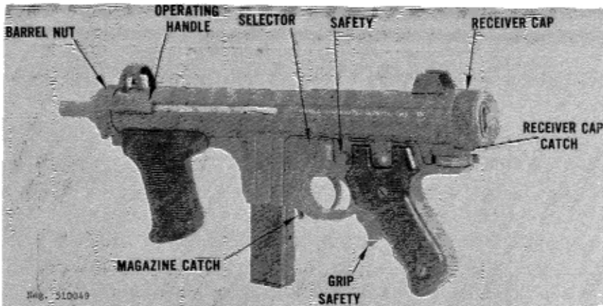
Figure 50. Beretta Model 12 submachinegun, stock folded, (late model).
