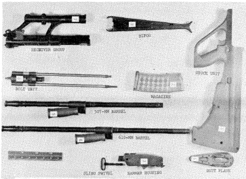
Figure 103.11. St.G 77 (AUG) field stripped.
