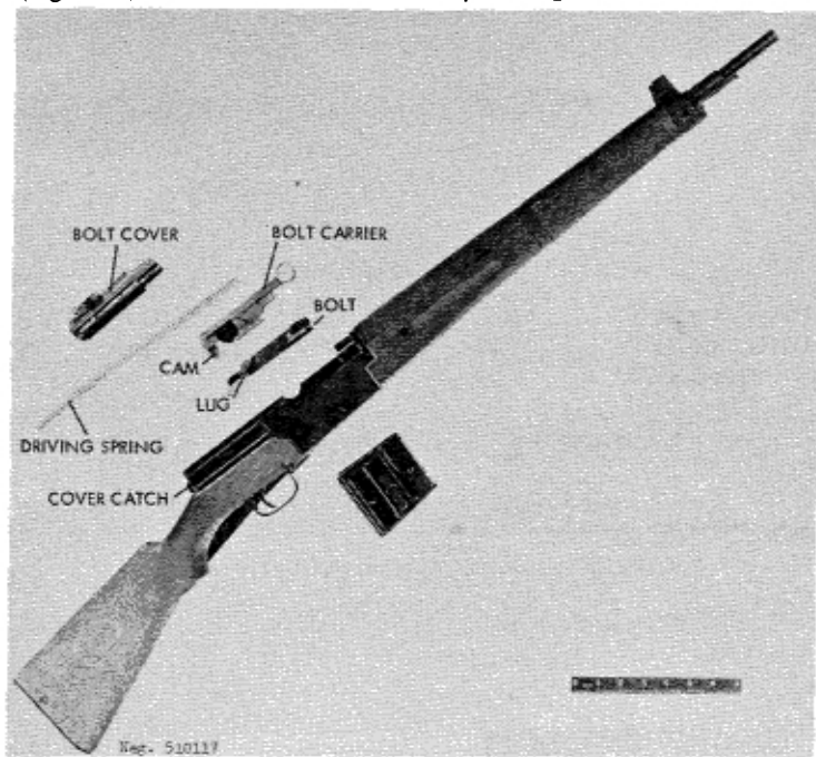
Figure 118. M.A.S. 49 disassembled.
