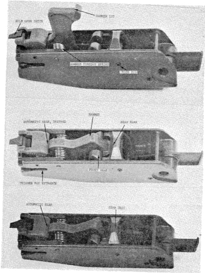
Figure 103.13. Hammer housing functioning.
