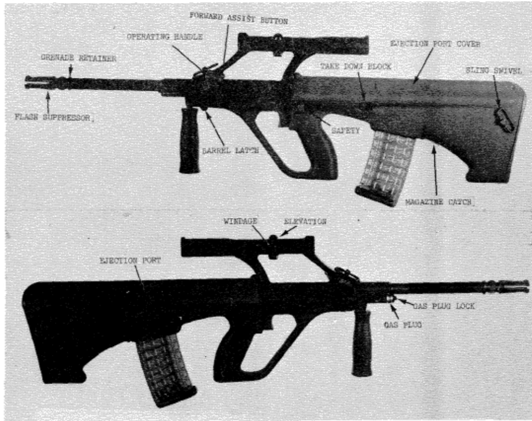
Figure 103.3. St.G 77 (AUG) controls.
