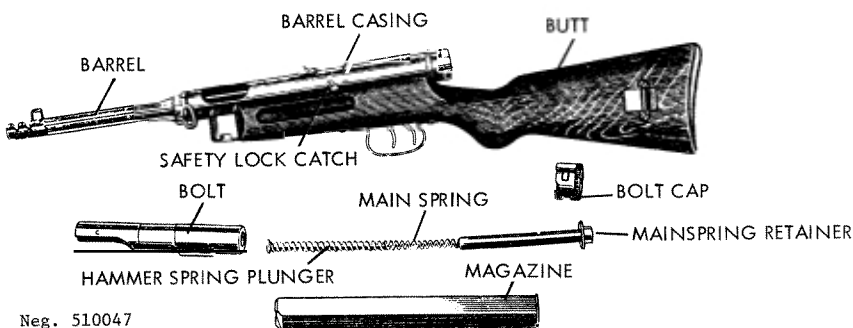
Figure 48. Beretta submachinegun, disassembled.
