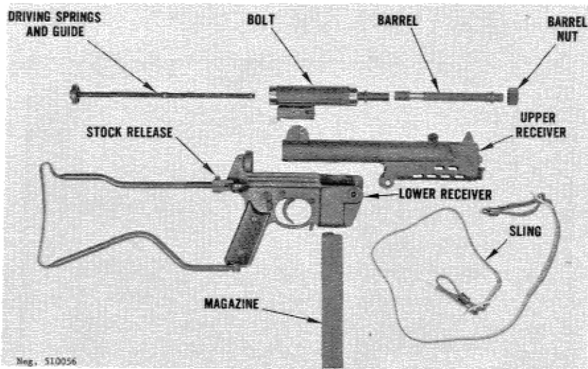
Figure 57. Walther MP-K disassembled.
