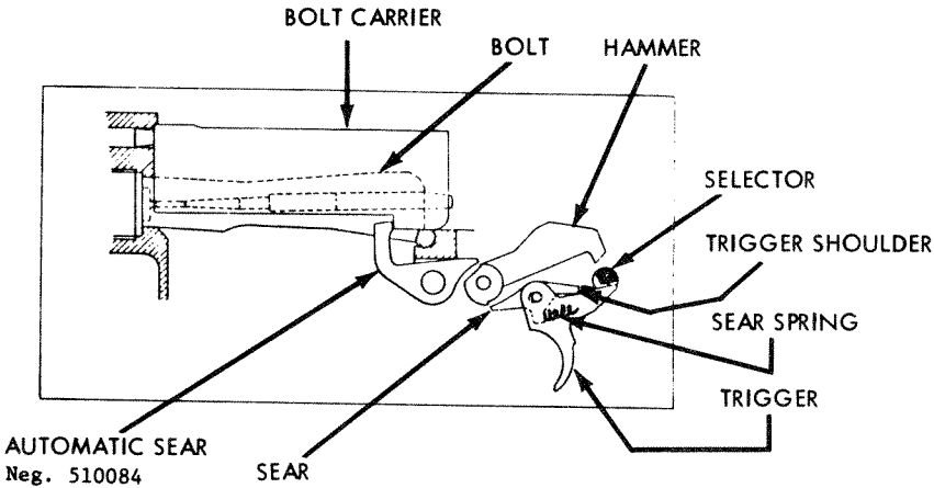
Figure 85. FN/FAL trigger.
