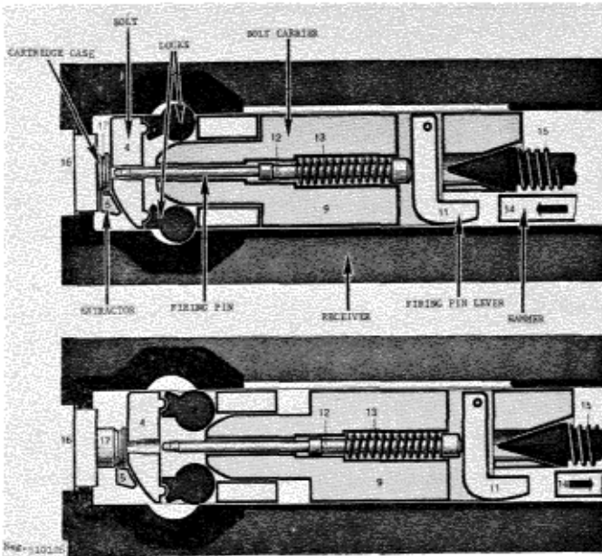
Figure 127. StG 57 bolt functioning.
