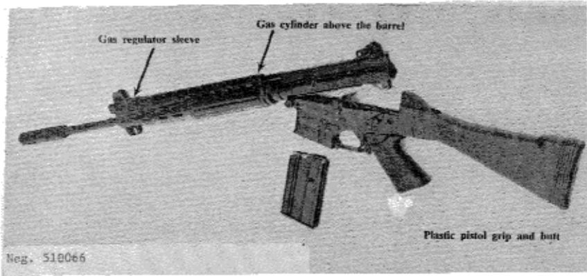
Figure 67. C.A.L. open for disassembly.
