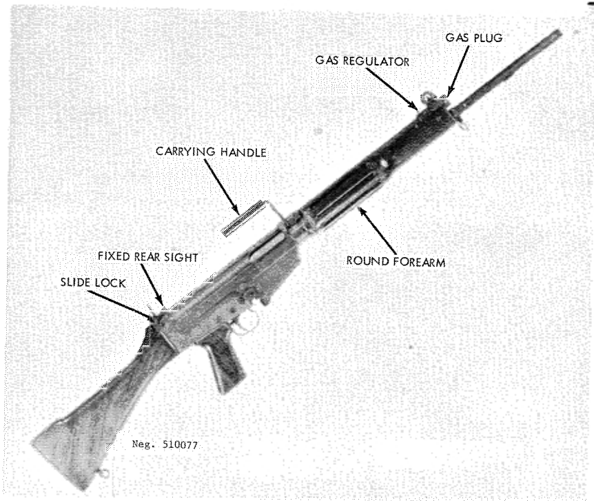
Figure 78. FN/FAL rifle, early version.
