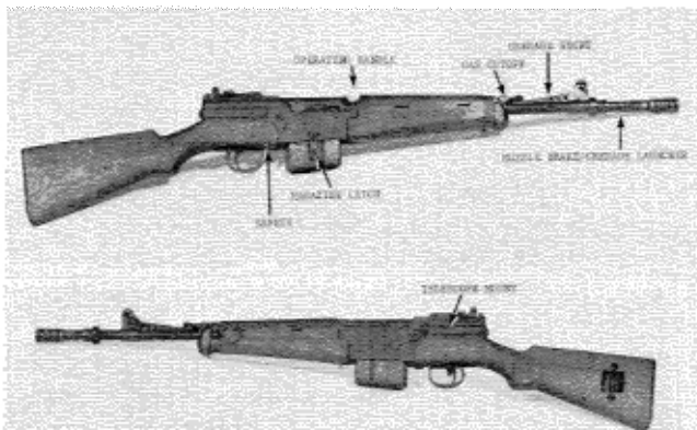
Figure 115. M.A.S. 49/56 Rifle
