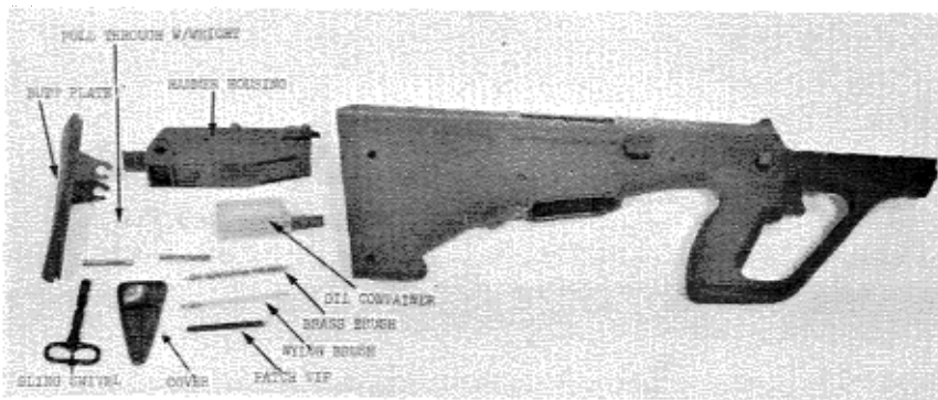
Figure 103.10. Stock unit disassembled.
