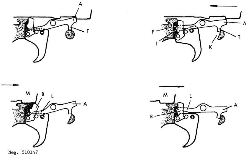
Figure 148. M.A.G. trigger functioning.
