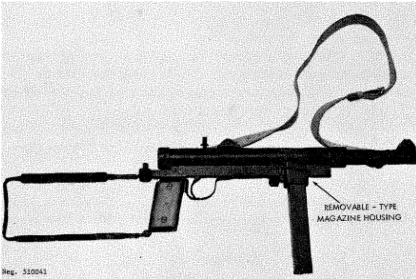
Figure 42. Swedish M45b submachinegun.
