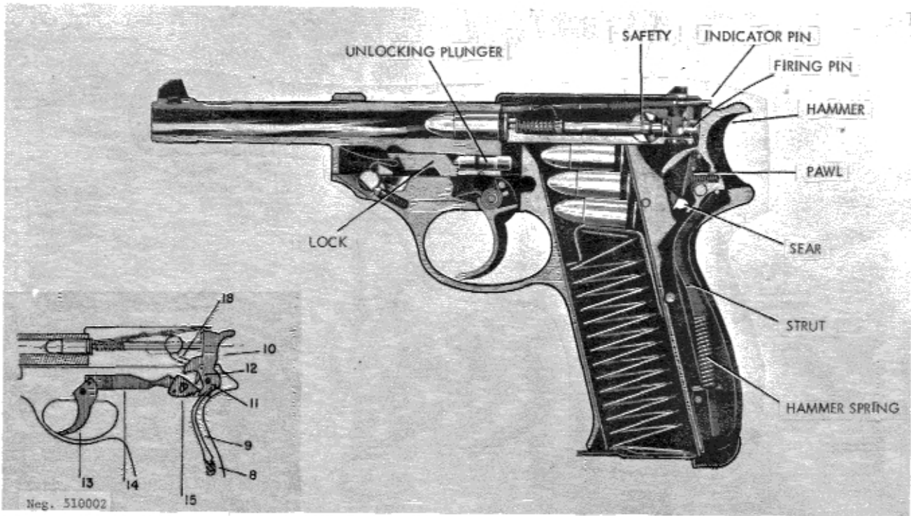
Figure 3. P1 pistol, section.
