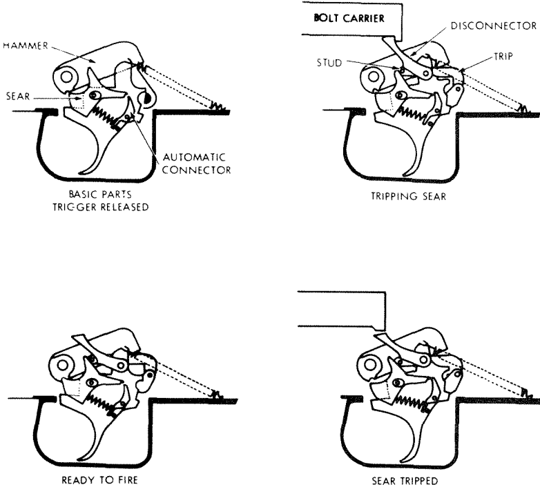
Figure 131. StG 57 trigger functioning.
