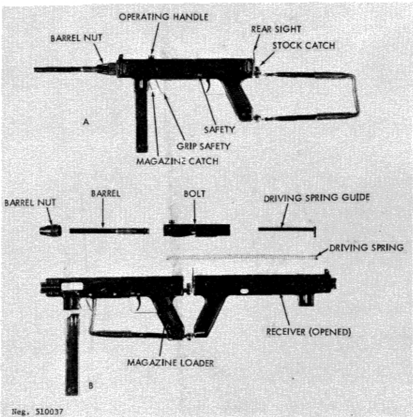
Figure 38. Danish Madsen Model 50 submachinegun.
