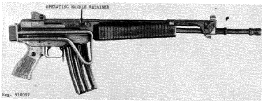
Figure 98. Beretta M70/.223 rifle with folding stock (early model).
