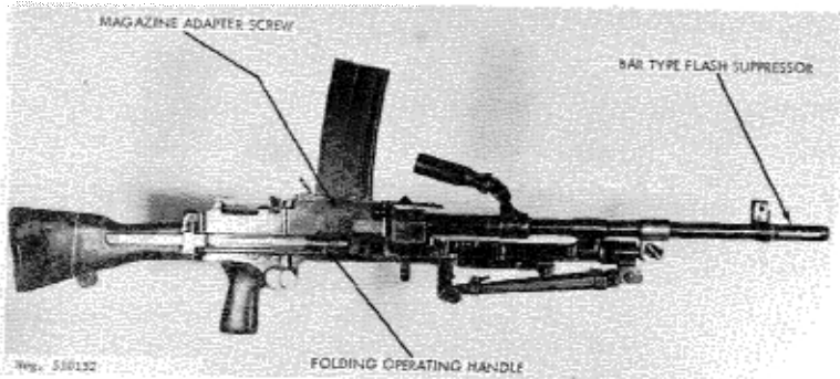
Figure 153. L4A1 Bren.
