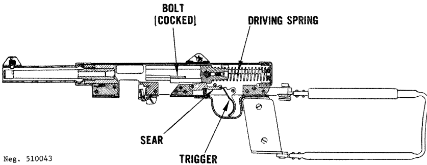
Figure 44. M45b section.
