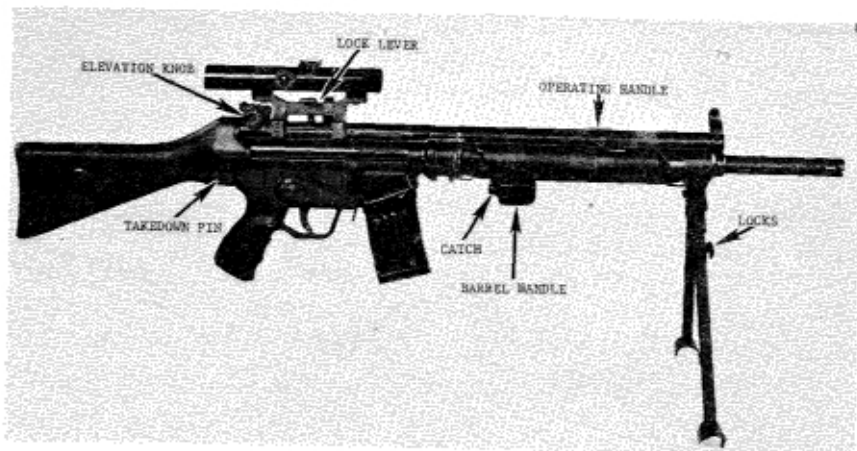
Figure 169. West German HK 13 light machinegun.
