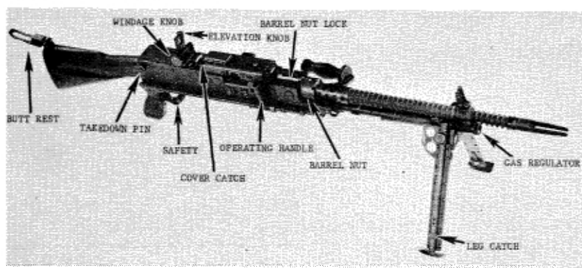
Figure 182. Japanese Type 62 machinegun.
