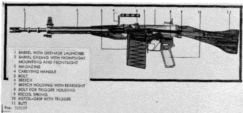
Figure 129. SIG 510-4 section.
