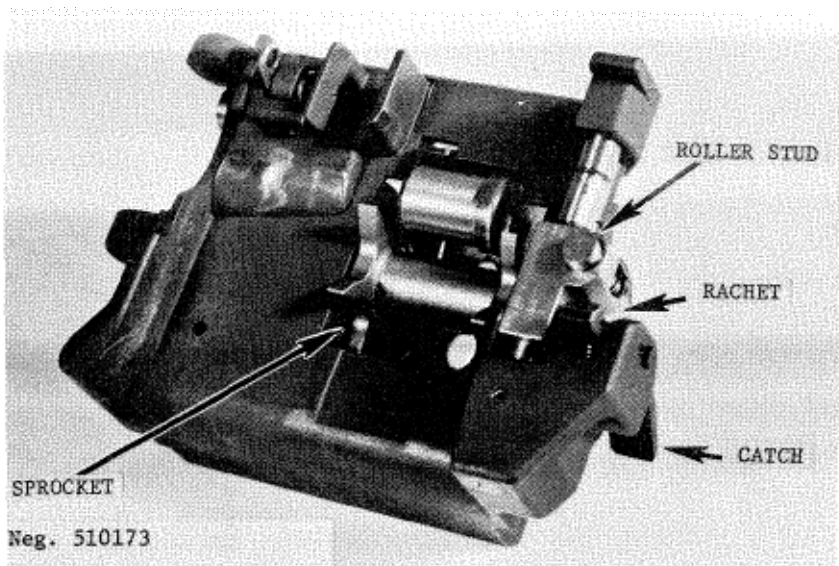
Figure 174. HK 21A1 feeder mechanism.
