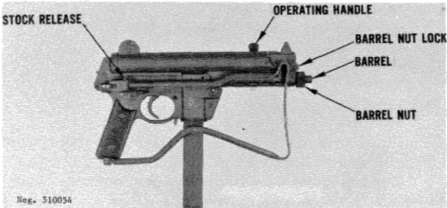
Figure 55. West German Walther MP-K submachinegun.
