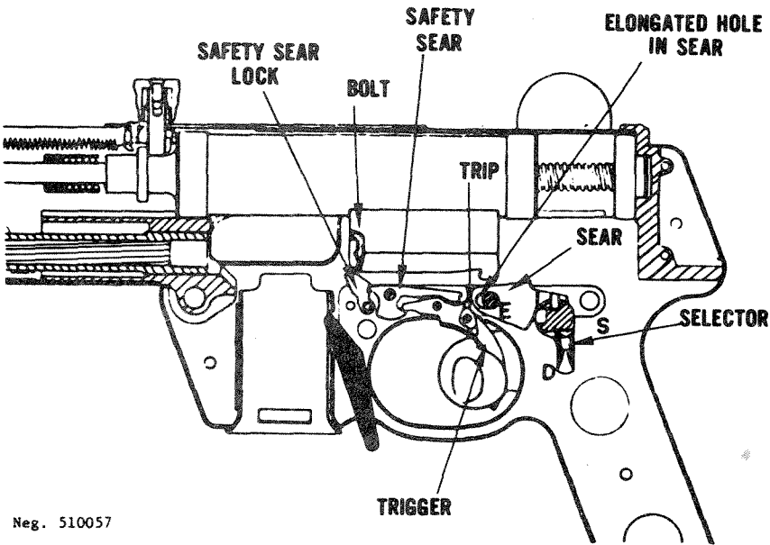
Figure 58. Walther MP-K or MP-L section.
