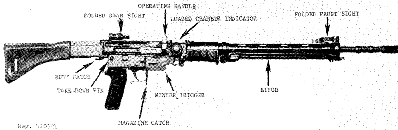
Figure 122. Swiss StG 57 assault rifle.
