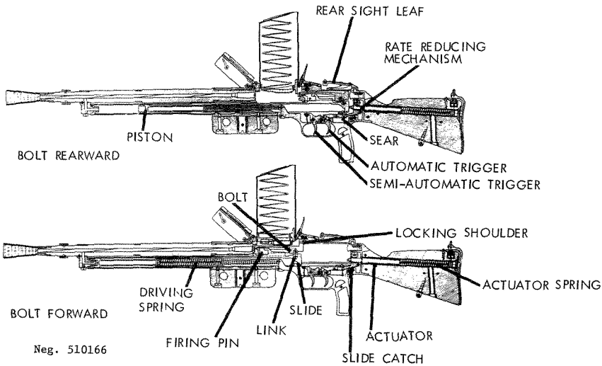
Figure 167. M24/29 section.
