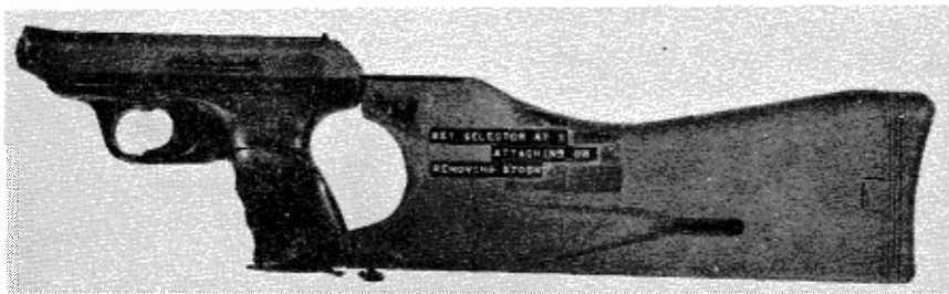
Figure 28.2.3. The VP-70 with holster-stock attached.
