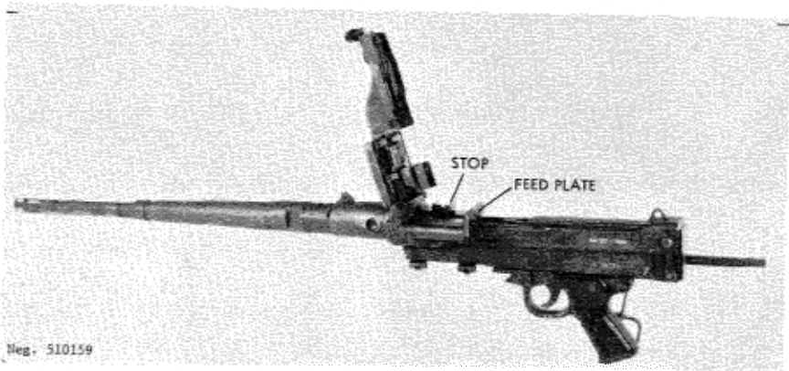
Figure 160. AAT-52 tank machinegun.
