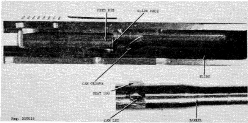
Figure 19. M.A.B. P15 barrel and slide.
