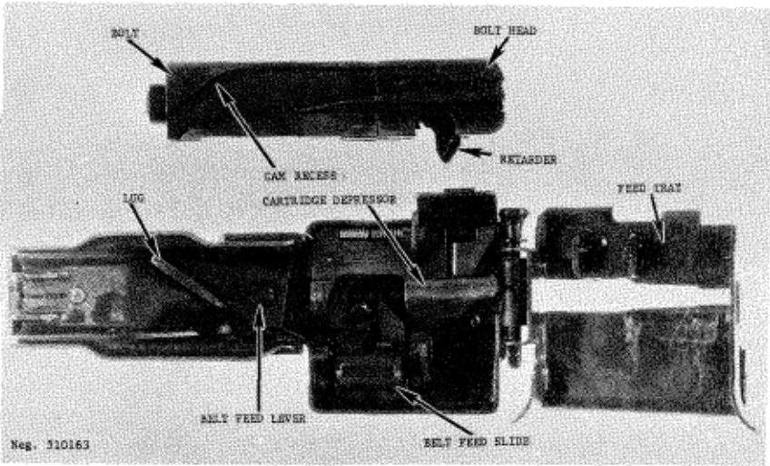
Figure 164. AA-52 bolt and feed cover.
