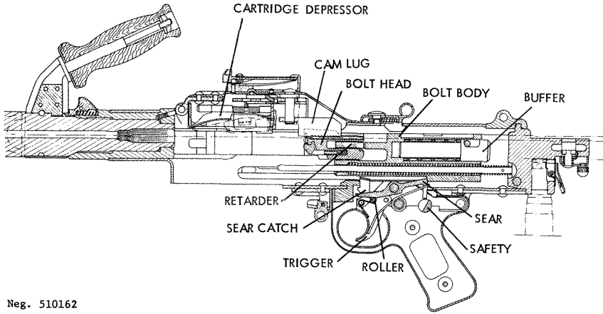
Figure 163. AA-52 section.
