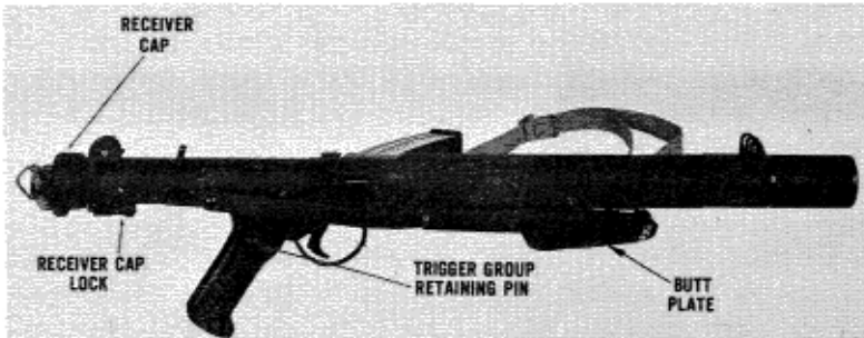
Figure 30. British L34A1 silenced submachinegun.
