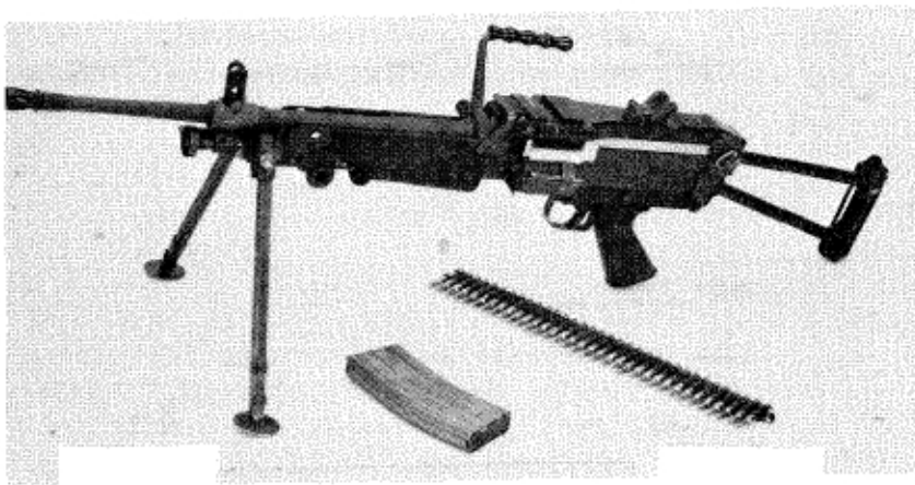
Figure 185.1. Belgian Minimi Light Machinegun
