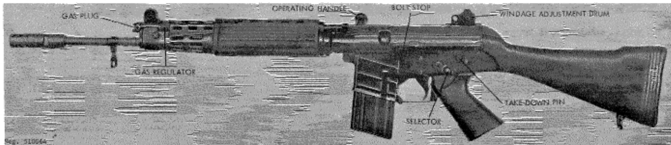
Figure 65. Belgium C.A.L. assault rifle.
