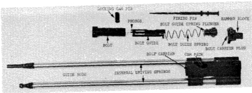
Figure 103.8. Bolt unit disassembled.
