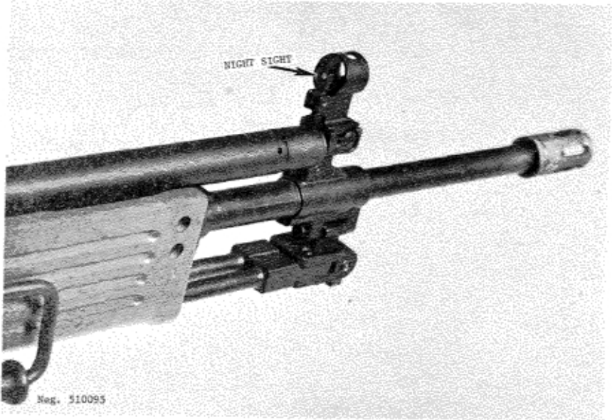
Figure 96. Galil front night sight.
