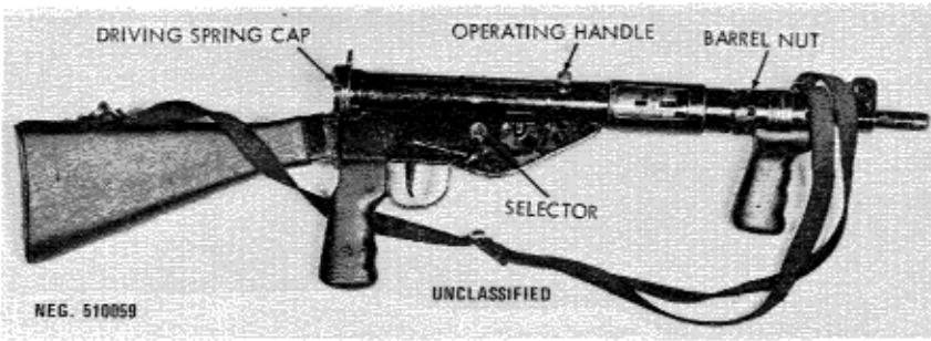
Figure 60. British Mark 5 Sten submachinegun.
