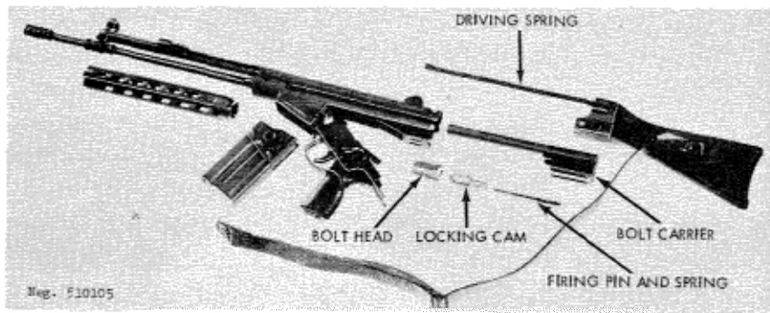
Figure 106. G3 disassembled.
