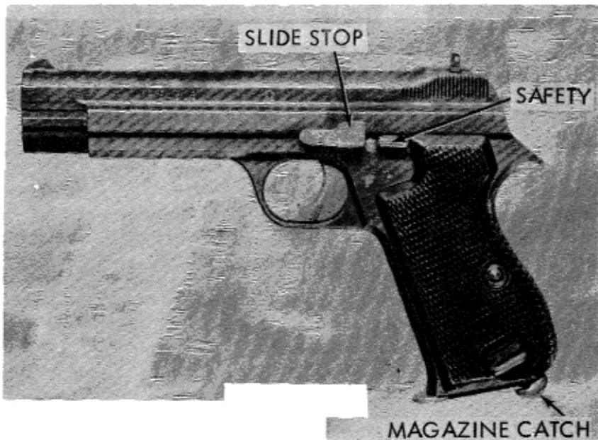
Figure 25. Swiss Model 49 (SIG P210) Pistol
