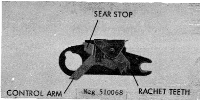
Figure 69. C.A.L. burst limiter.
