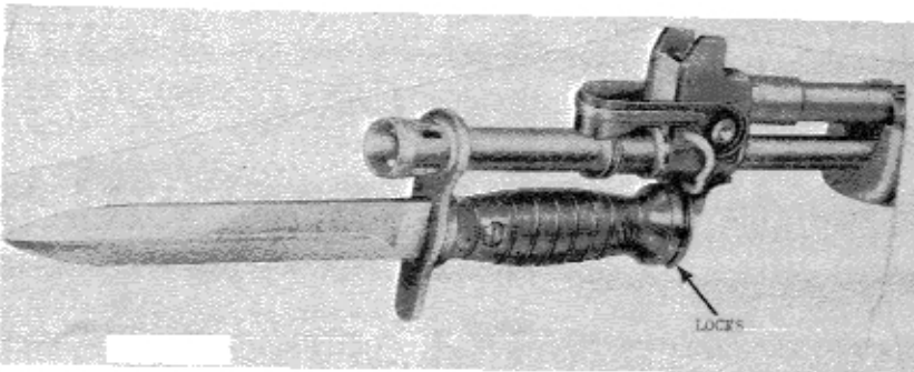
Figure 102. Beretta M70/.223 Bayonet
