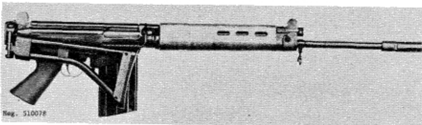
Figure 79. FN/FAL paratrooper's model.
