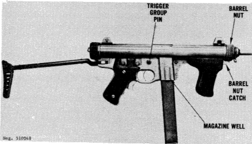
Figure 49. Italian Beretta Model 12 submachinegun (early model).
