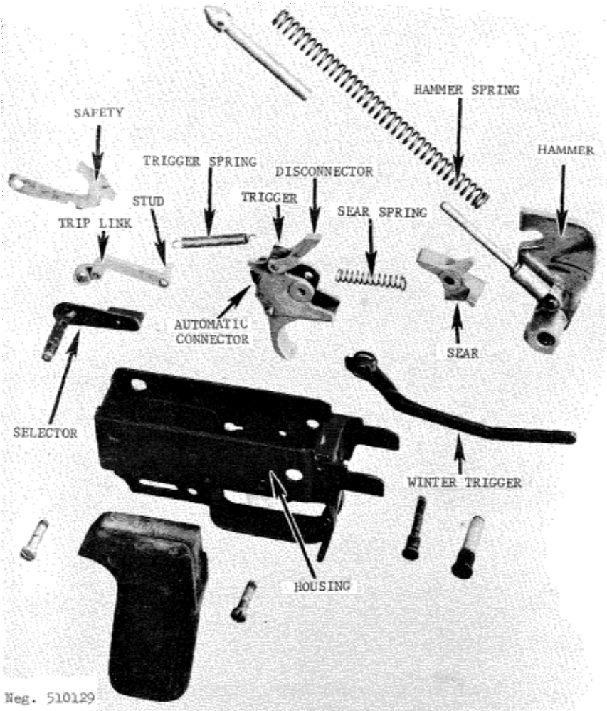
Figure 130. StG 57 trigger mechanism.
