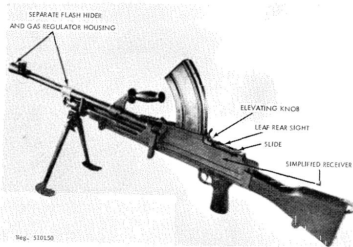
Figure 151. Mark 2 Bren.
