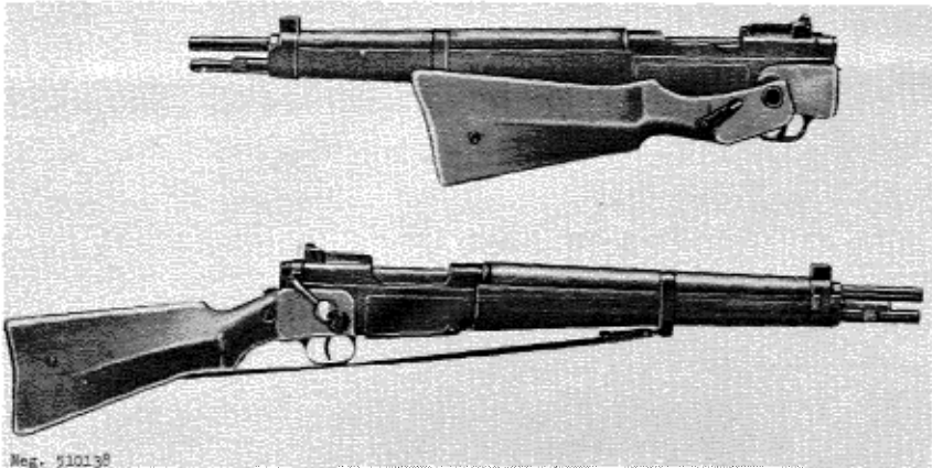
Figure 139. French M.A.S. 36 CR 39 rifle.
