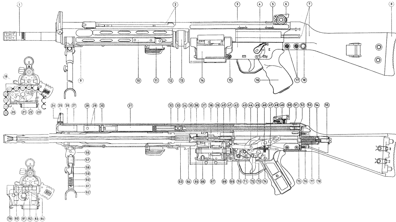
Figure 173. H21 section.
