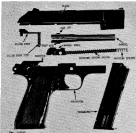
Figure 18. M.A.B. P15S disassembled.
