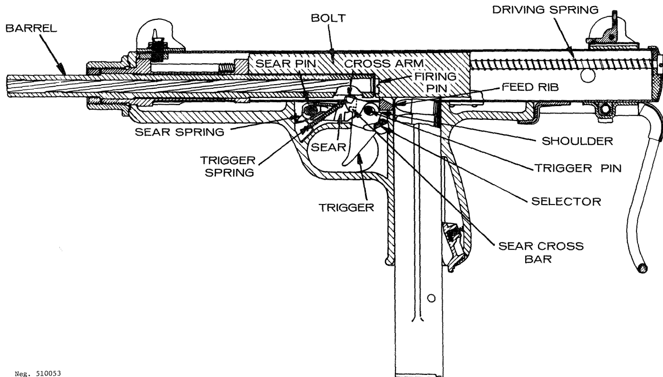
Figure 54. MPi Steyr 69 section.
