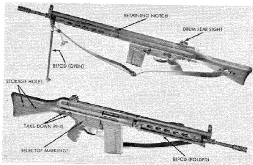
Figure 105. West German G3 rifle.
