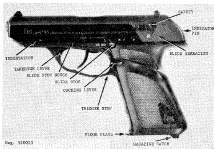
Figure 21. West German P9 pistol.
