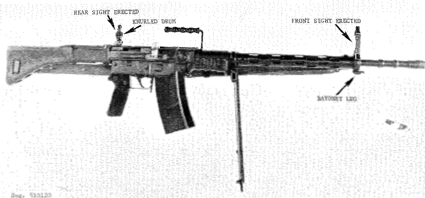
Figure 123. StG 57 with bipod extended.
