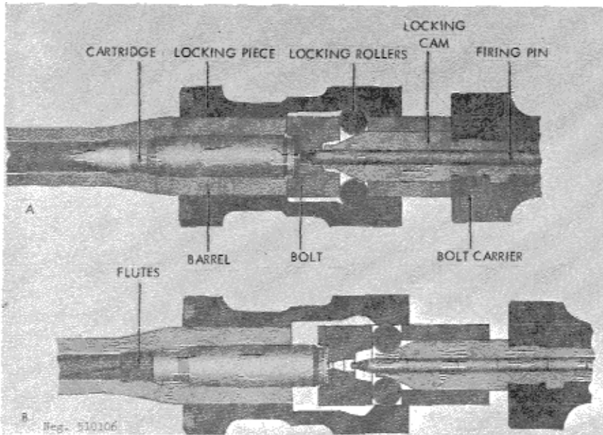
Figure 107. G3 bolt functioning.
