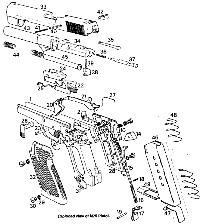
Figure 28.1.1. Swiss 9-mm Model 75 pistol, exploded view.
