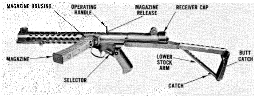
Figure 29. British L2A3 submachinegun.
