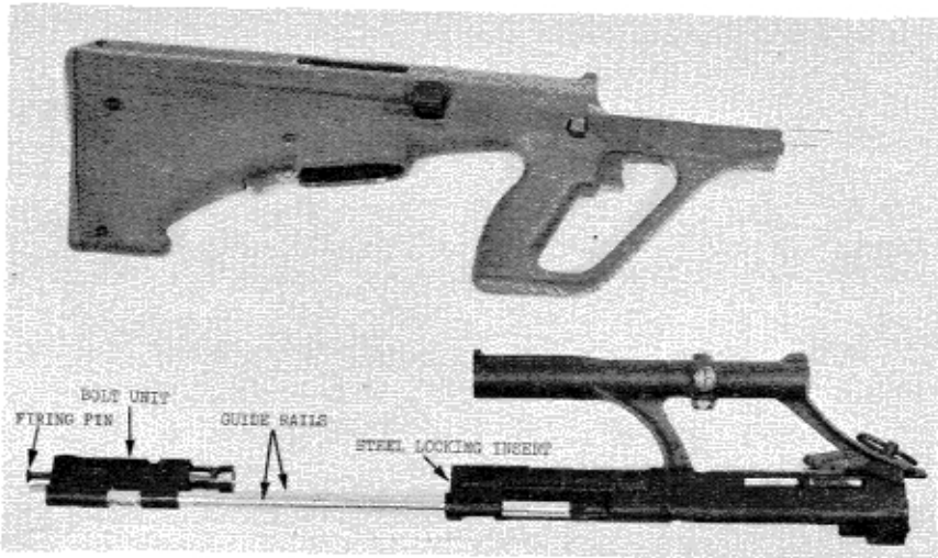
Figure 103.7. Removal of bolt mechanism from receiver.
