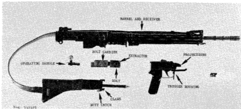
Figure 126. StG 57 disassembly.
