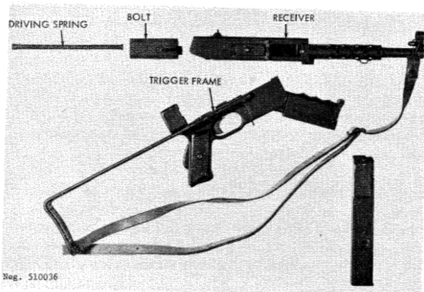
Figure 37. M.A.T. 49 disassembled.
