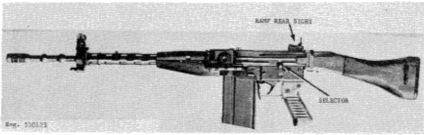
Figure 124. Swiss SIG 510-4 assault rifle.
