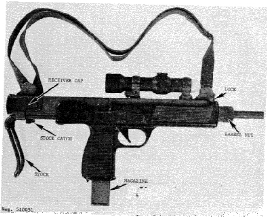
Figure 52. Austrian Steyr MPi Steyr 69 submachinegun.
