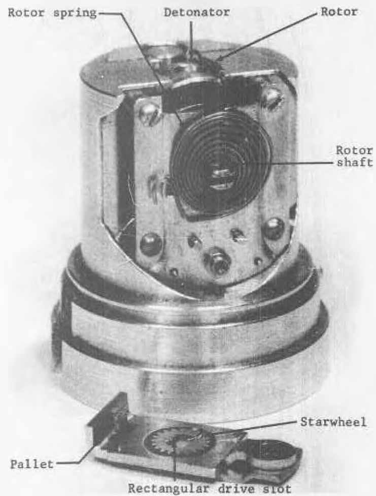
Figure 1. T278E7 (M530) and -E8 PIBD fuzes.
