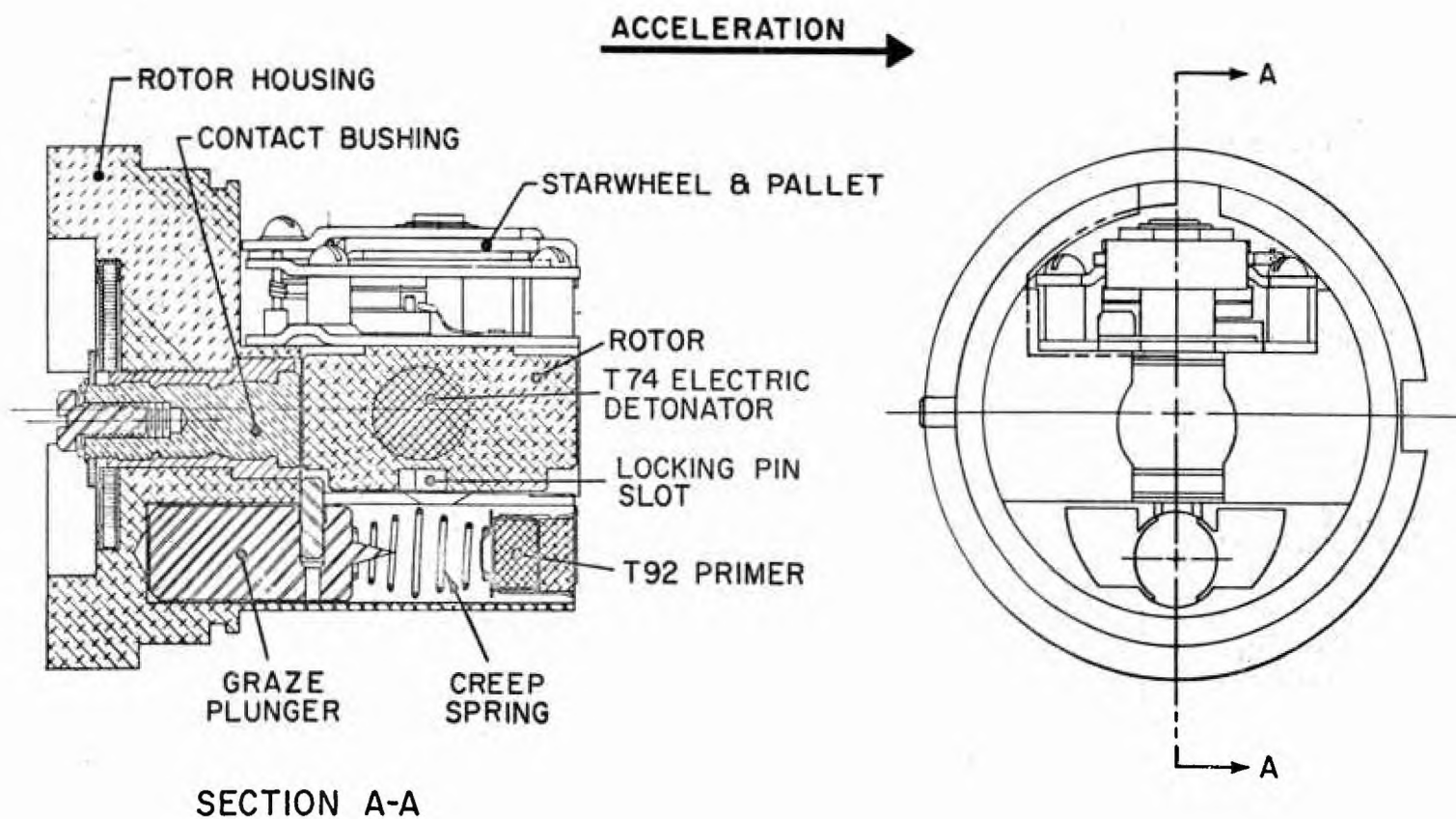
Figure 5. Line drawing of rotor housing release assembly (unarmed).
