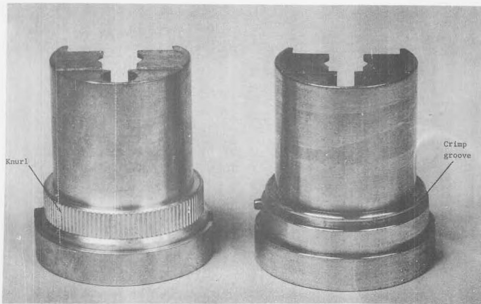
1125-62 Figure 12. Rotor housings designed for knurl press assembly and 360-deg crimp assembly of shield.
