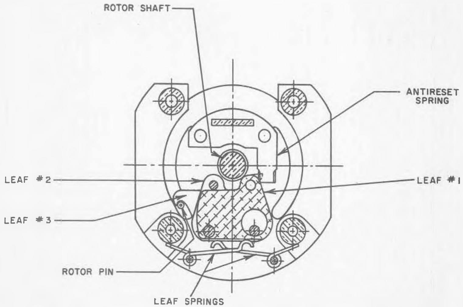
Figure 2. Sequential leaf setback release mechanism.
