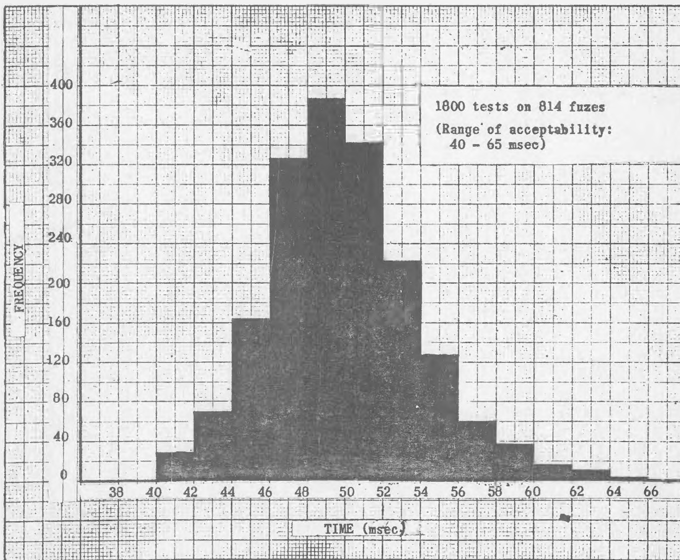
Figure 11. Graph showing frequency distribution of static rotor arming time of T278E8.
