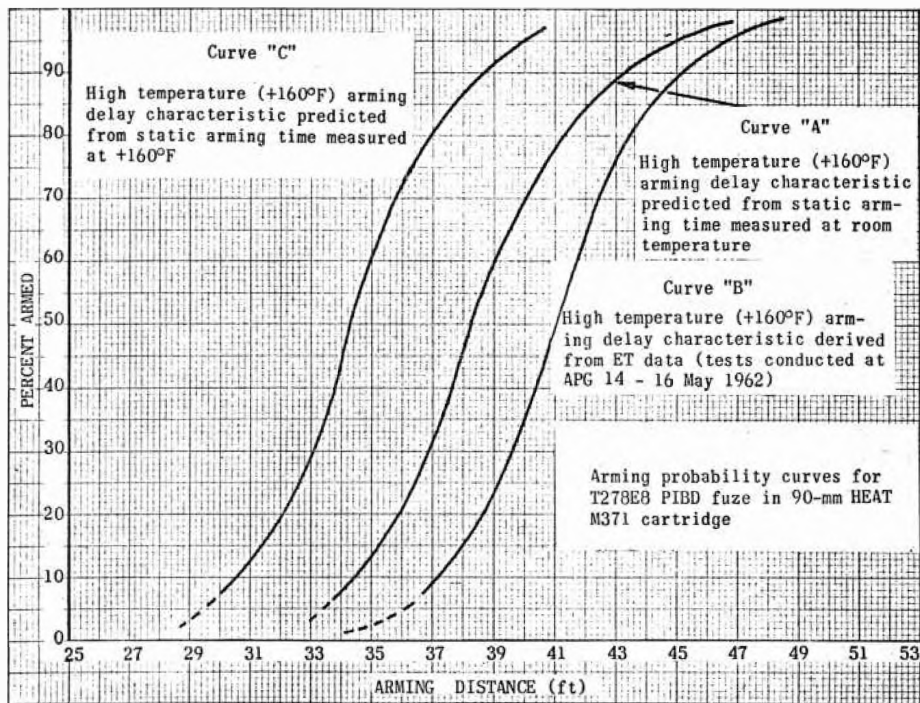
Figure 15. Arming delay characteristics at +160°F and room temperature.
