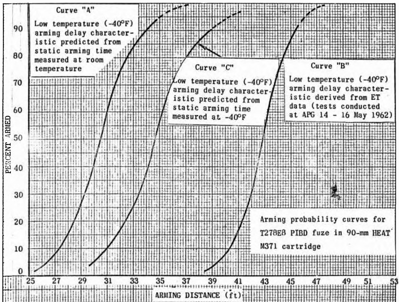
Figure 16. Arming delay characteristics at -40°F and room temperature.
