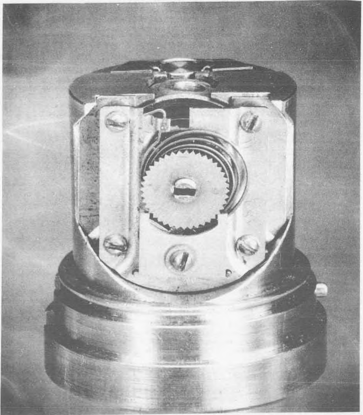
1981-61 Figure 8. Starwheel and pallet design.
