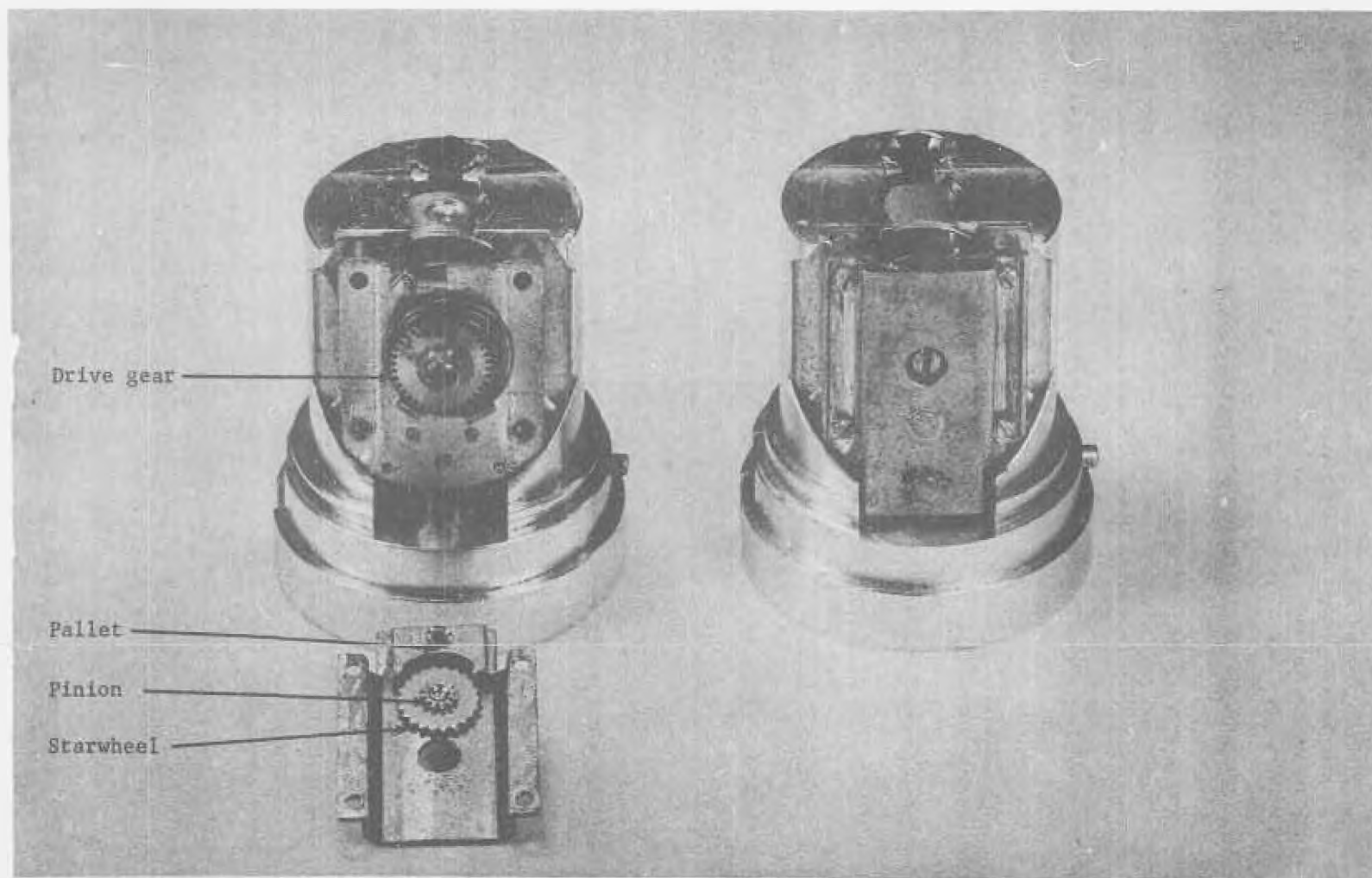
Figure 9. Modified starwheel and pallet design.
