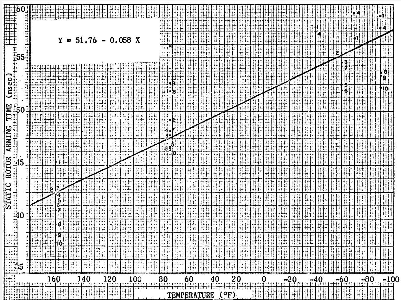
Figure 14. Static rotor arming time versus temperature for T278E8 fuze.
