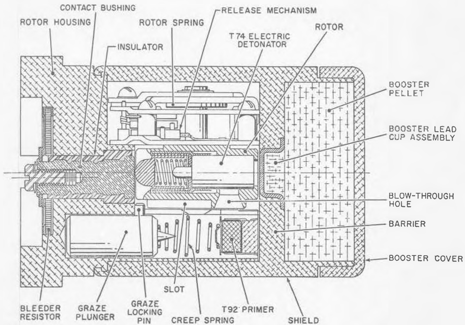
Figure 4. Line drawing of T278E8 fuze (armed).
