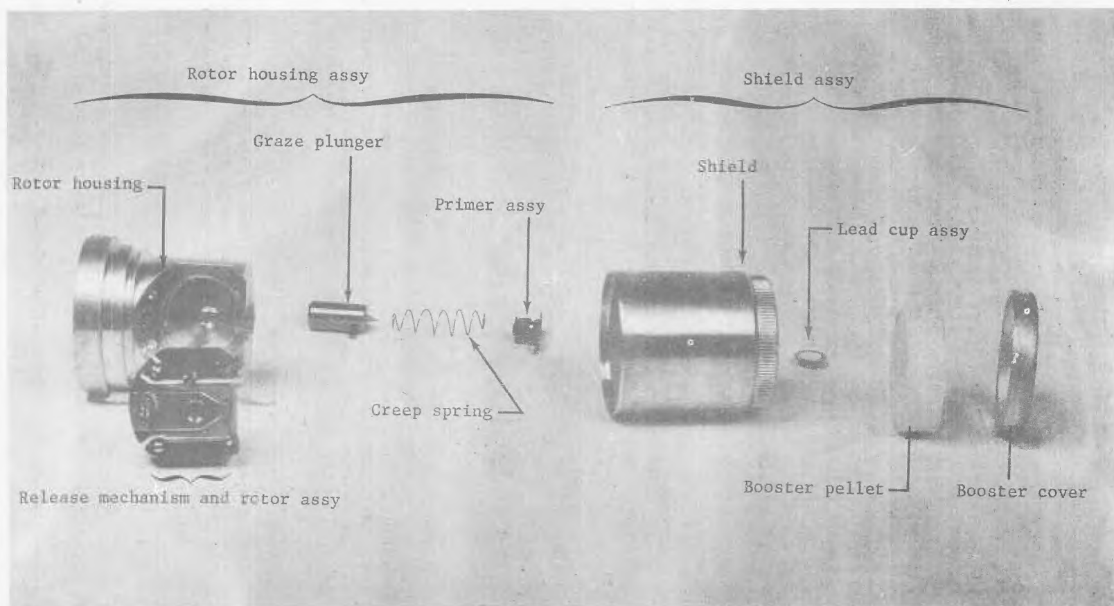
Figure 3. Exploded view of T278E8 fuze.
