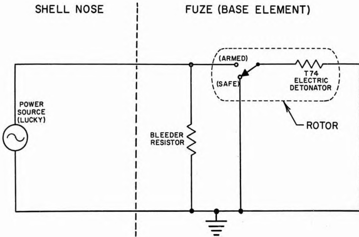
Figure 6. Circuit diagram of T278E8 fuze and shell assembly.
