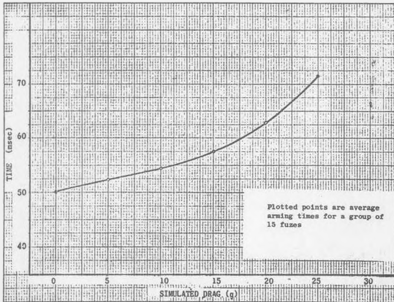
Figure 13. Drag deceleration effect (simulated by centrifuge) on T278E8 rotor arming time.
