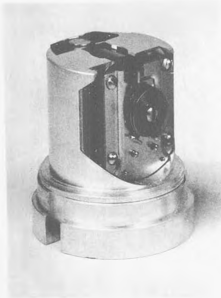
T278E7 fuze (M530) in safe position
