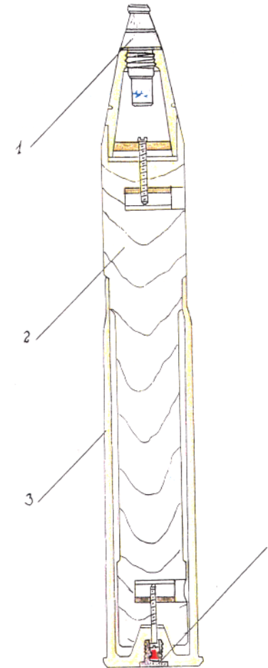
Figure 20. Training round.
