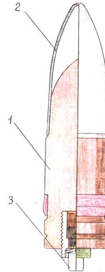
Figure 6. Solid AP shell with ballistic cap 1. Body 2. Cap 3. Tracer.
