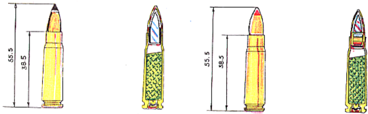
Figure 7-6 7.62 round model 56 with AP- incendiary bullet.
