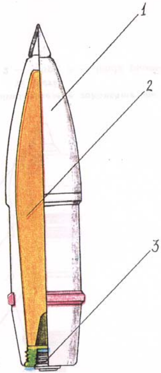
Figure 3. HE shell: 1. Body. 2. Explosive charge. 3. Fuze.
