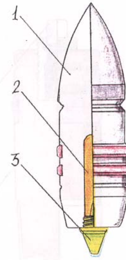
Figure 4. Standard sharp-nosed AP shell: 1. Body. 2. Explosive charge. 3. Fuze.
