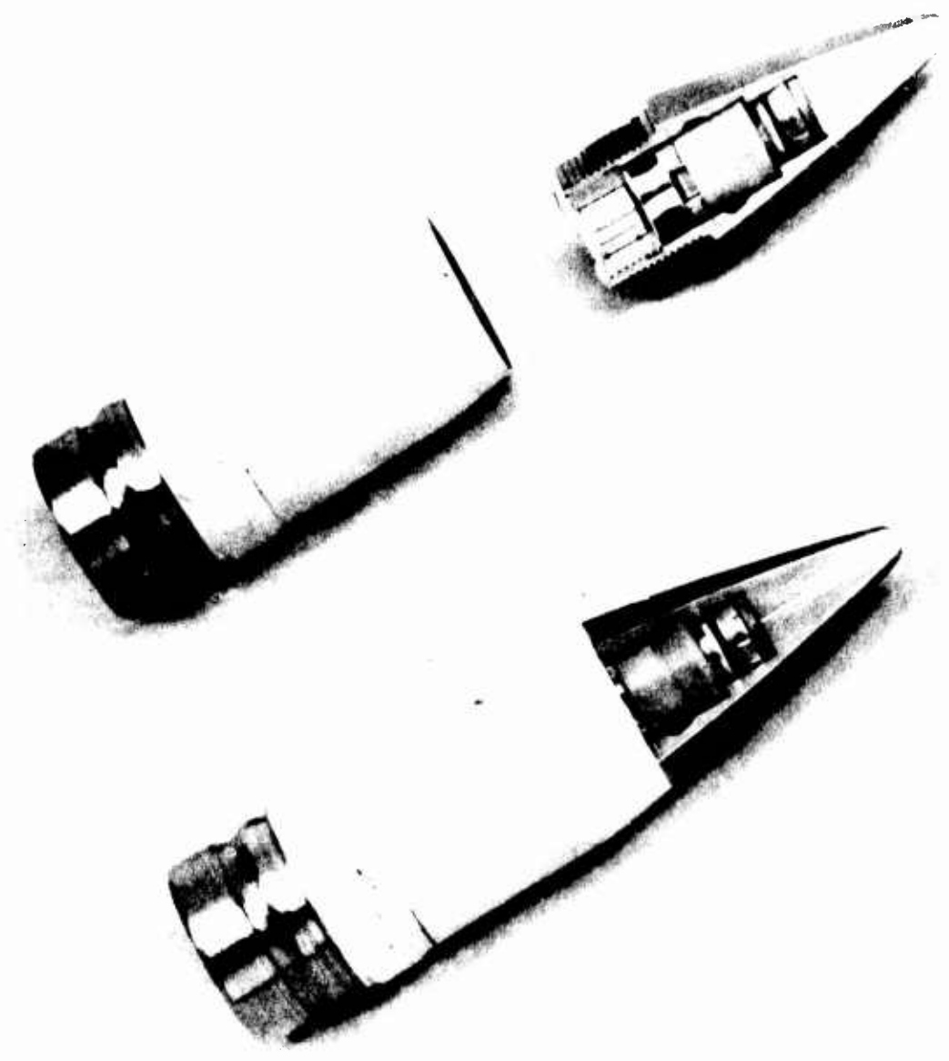
Figure B-3. Test Vehicle Projectile Assembly Cutaway View
