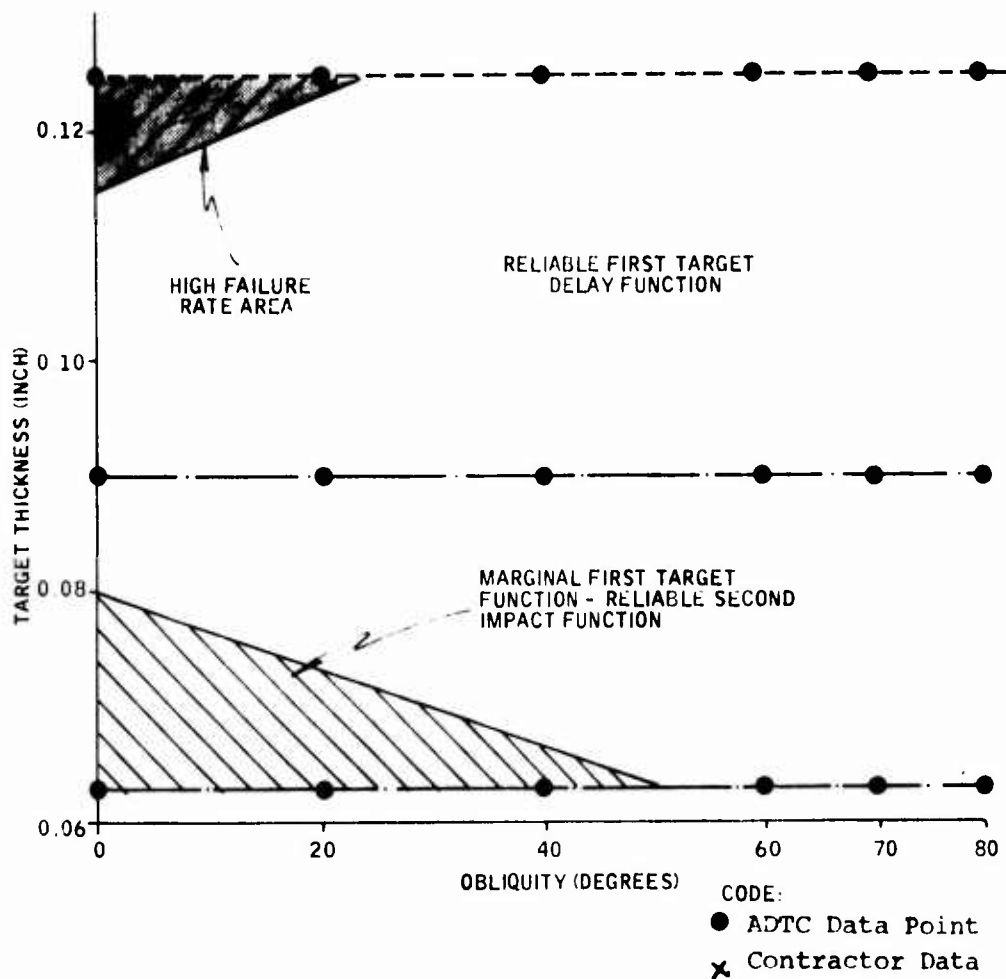
Figure 13. ADTC Delay Function Fuze Test Results - Impact Velocity = 3000 ft/s
