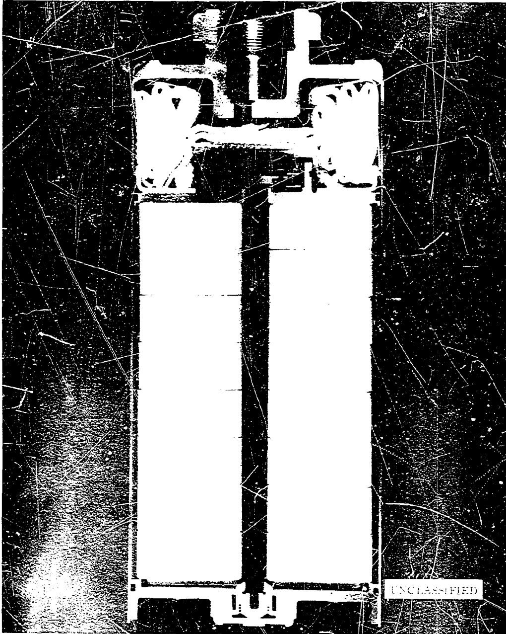
Figure 6. BLU 30/B Bomblet Display Model
