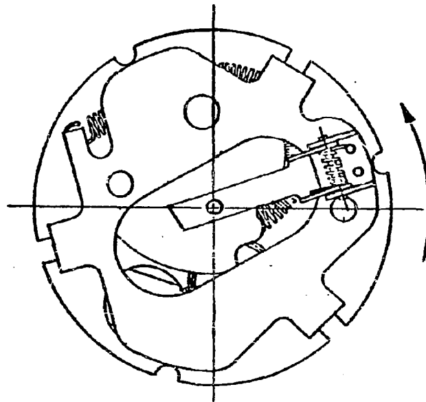
STORED ENERGY FIRING PIN ASSEMBLY
