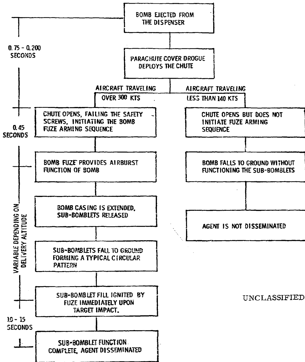
Figure 11. Bomblet Function Sequence
