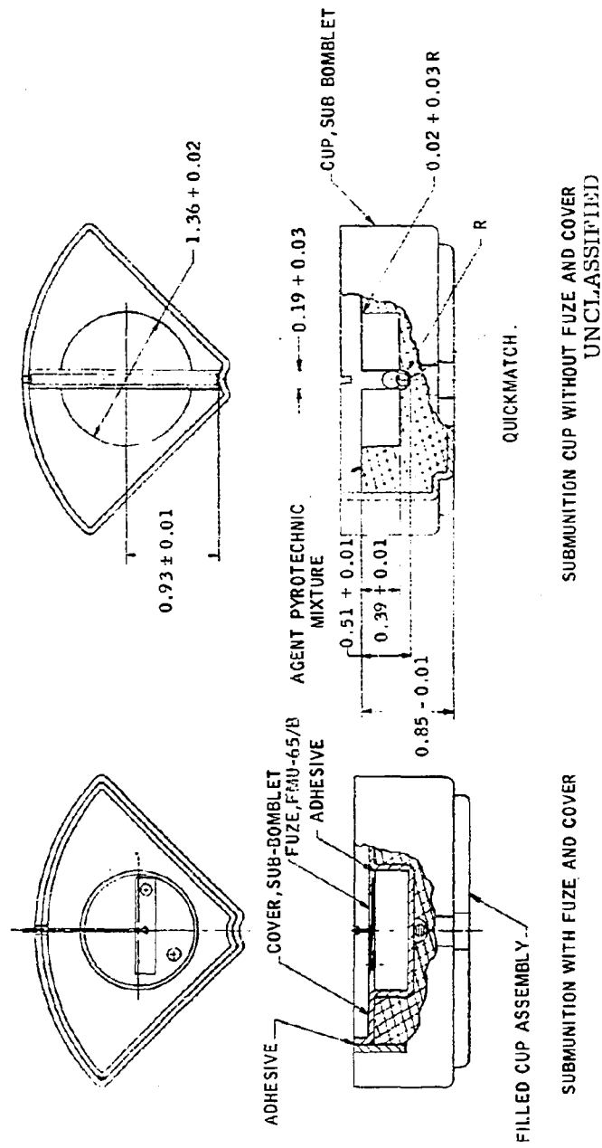
Figure 9. Sub-bomblet Configuration
