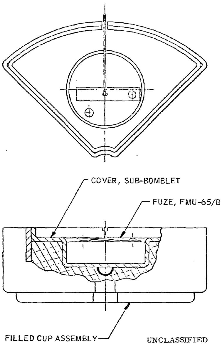
Figure 41. Sub-bomblet Configuration
