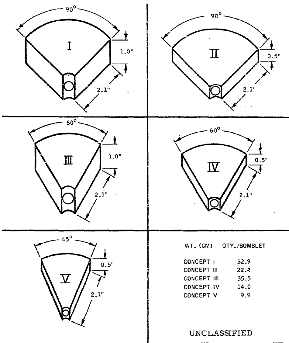
Figure 12. Sub-bomblet Candidate Designs
