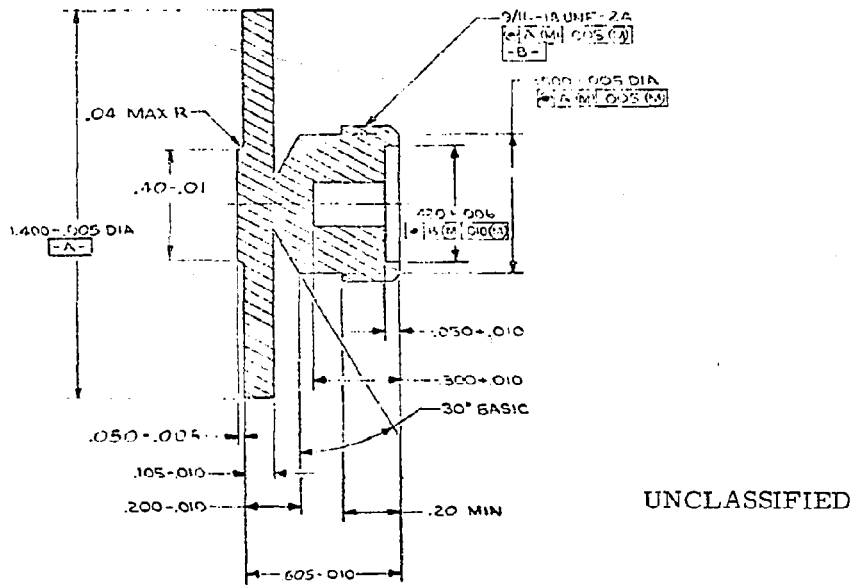
Figure 39. Revised Explosive Bolt
