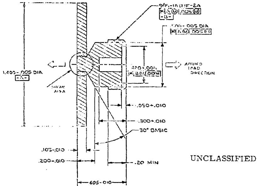
Figure 38. Explosive Bolt Structure Failure
